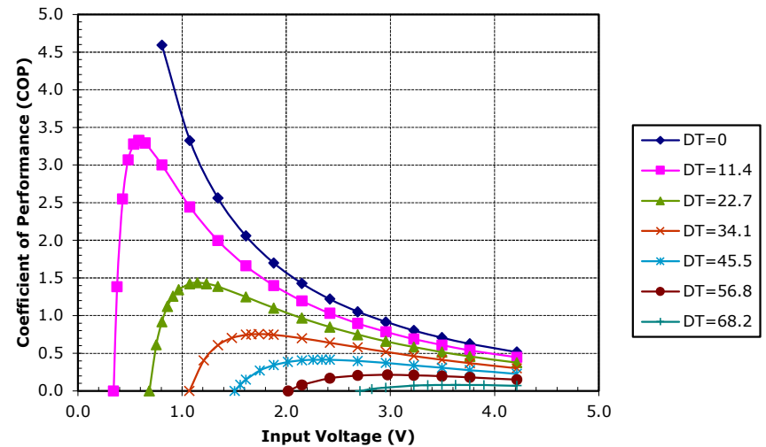
Unpotted TE-31-1.0-2.5 at a hot-side temperature of 50 °C
