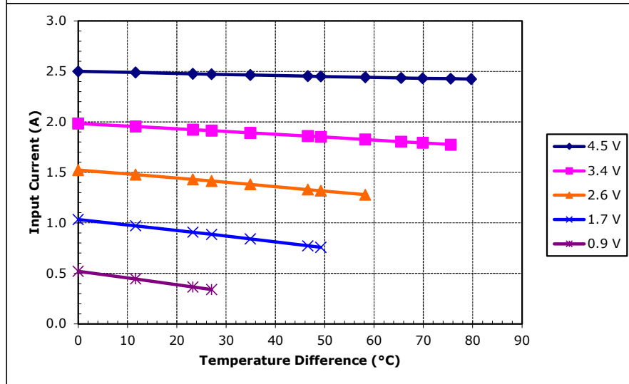
Potted TE-31-1.0-2.0 at a hot-side temperature of 70 °C
