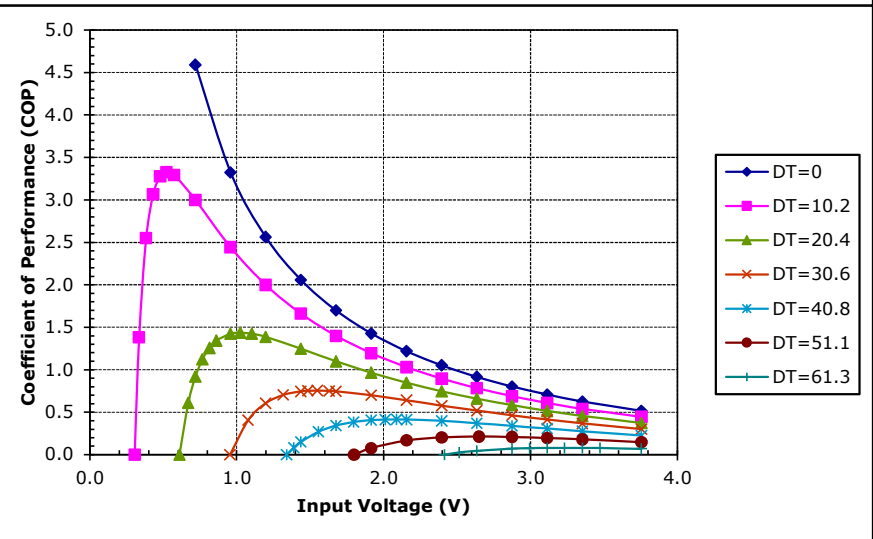
Unpotted TE-31-1.0-2.0 at a hot-side temperature of 30 °C
