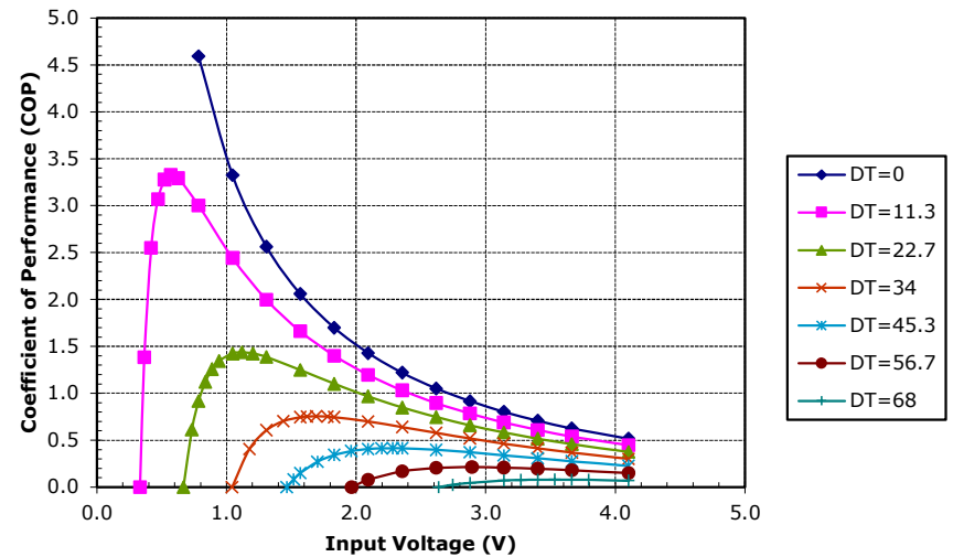
Unpotted TE-31-1.0-2.0 at a hot-side temperature of 50 °C
