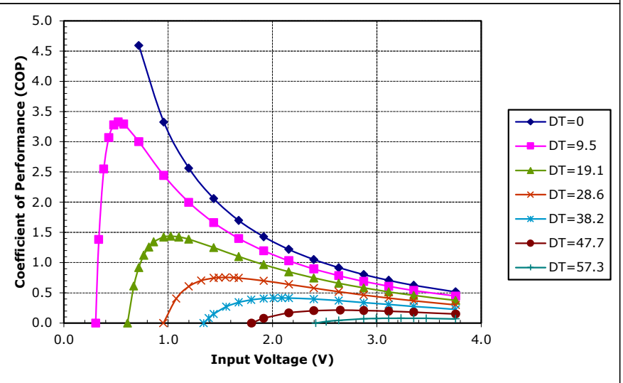
Potted TE-31-1.0-2.0 at a hot-side temperature of 30 °C
