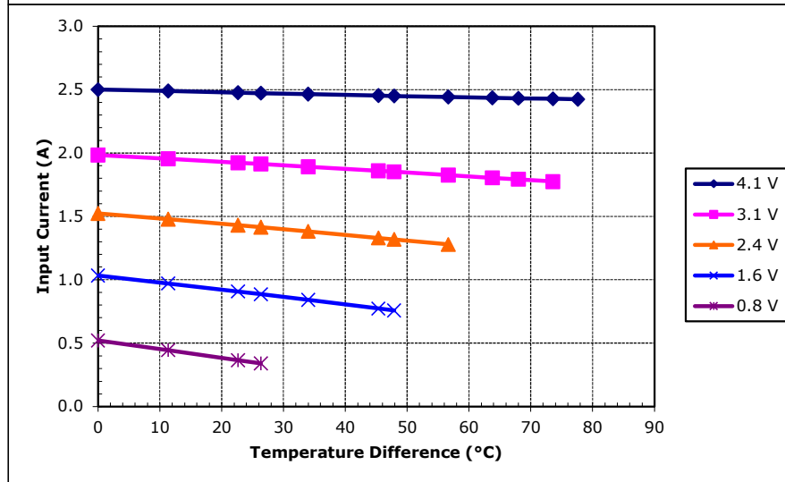
Unpotted TE-31-1.0-2.0 at a hot-side temperature of 50 °C
