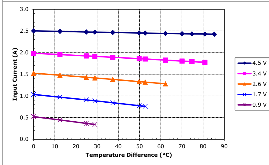
Unpotted TE-31-1.0-2.0 at a hot-side temperature of 70 °C
