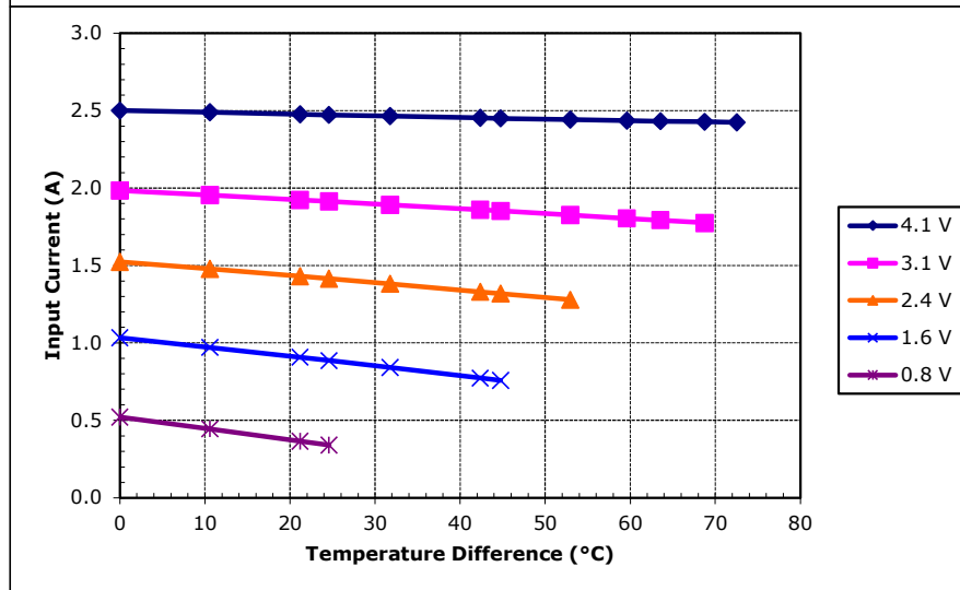
Potted TE-31-1.0-2.0 at a hot-side temperature of 50 °C
