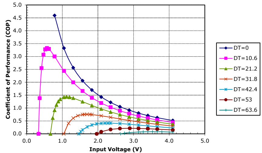
Potted TE-31-1.0-2.0 at a hot-side temperature of 50 °C
