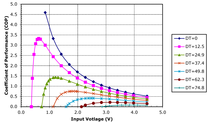
Unpotted TE-31-1.0-2.0 at a hot-side temperature of 70 °C
