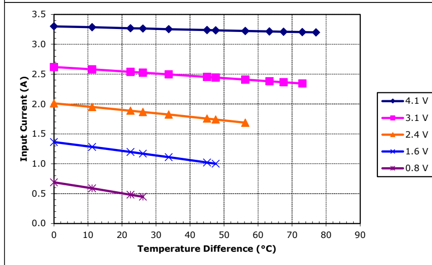
Unpotted TE-31-1.0-1.5 at a hot-side temperature of 50 °C
