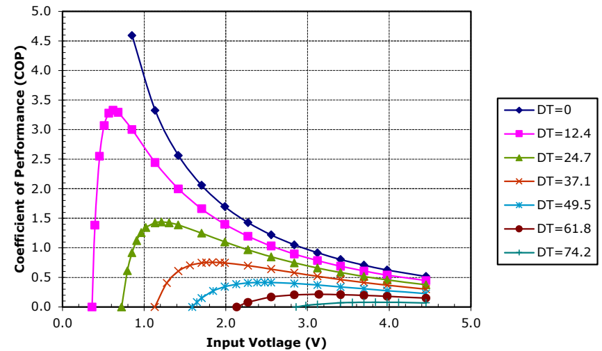
Unpotted TE-31-1.0-1.5 at a hot-side temperature of 70 °C
