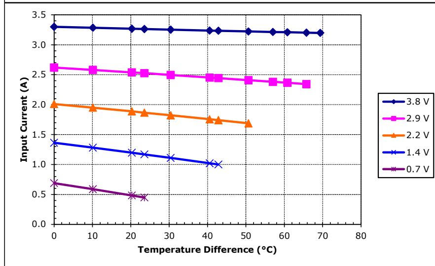
Unpotted TE-31-1.0-1.5 at a hot-side temperature of 30 °C
