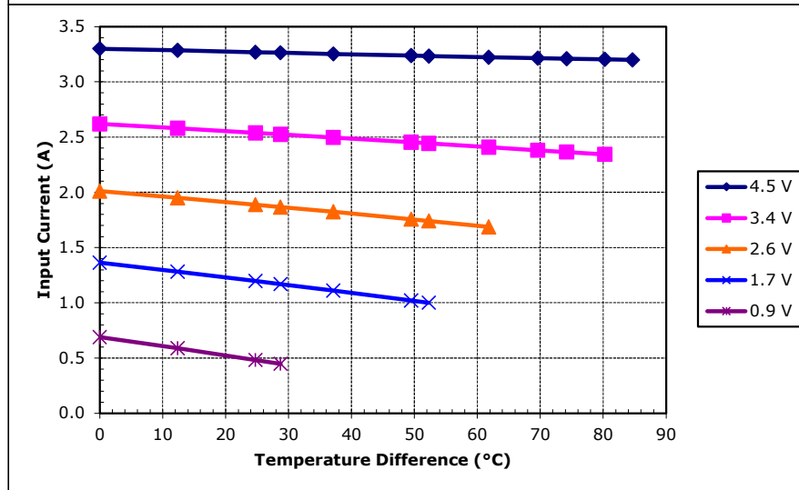
Unpotted TE-31-1.0-1.5 at a hot-side temperature of 70 °C
