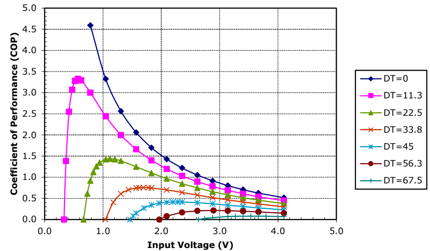
Unpotted TE-31-1.0-1.5 at a hot-side temperature of 50 °C
