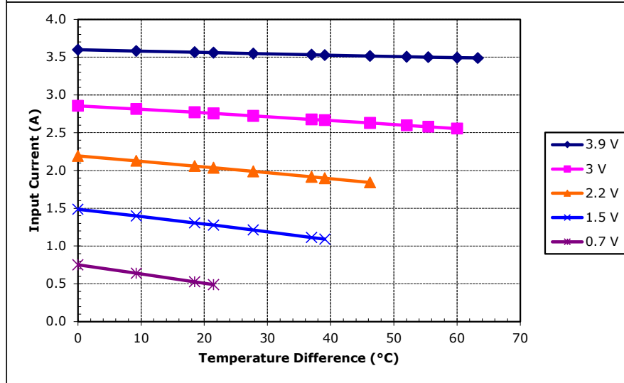
Potted TE-31-1.0-1.3 at a hot-side temperature of 30 °C
