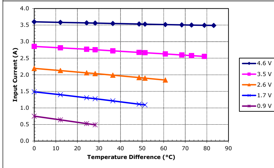
Unpotted TE-31-1.0-1.3 at a hot-side temperature of 70 °C
