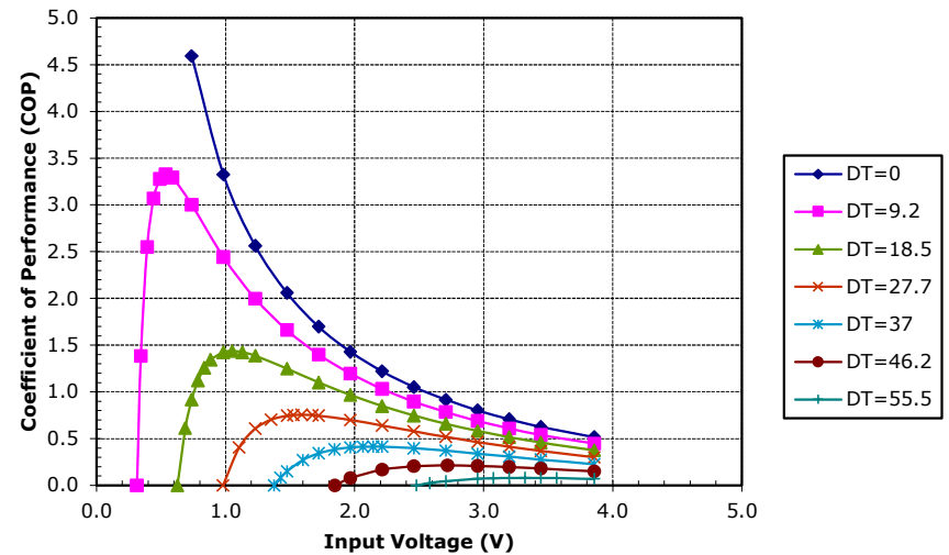
Potted TE-31-1.0-1.3 at a hot-side temperature of 30 °C
