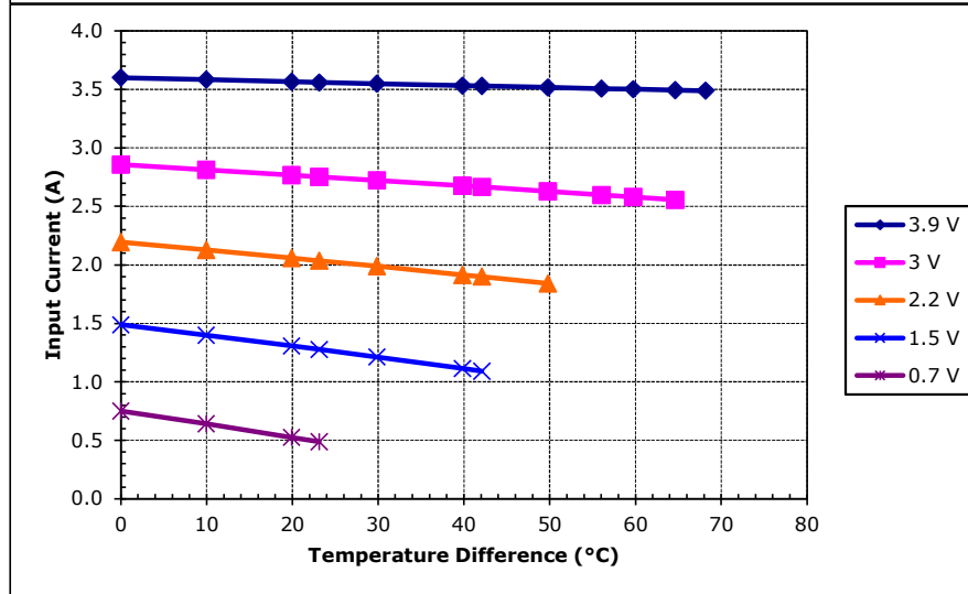
Unpotted TE-31-1.0-1.3 at a hot-side temperature of 30 °C
