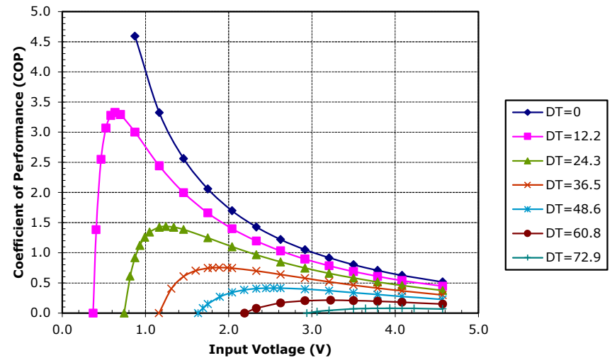
Unpotted TE-31-1.0-1.3 at a hot-side temperature of 70 °C
