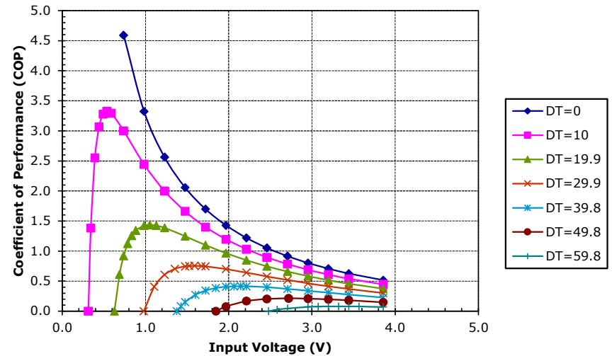
Unpotted TE-31-1.0-1.3 at a hot-side temperature of 30 °C
