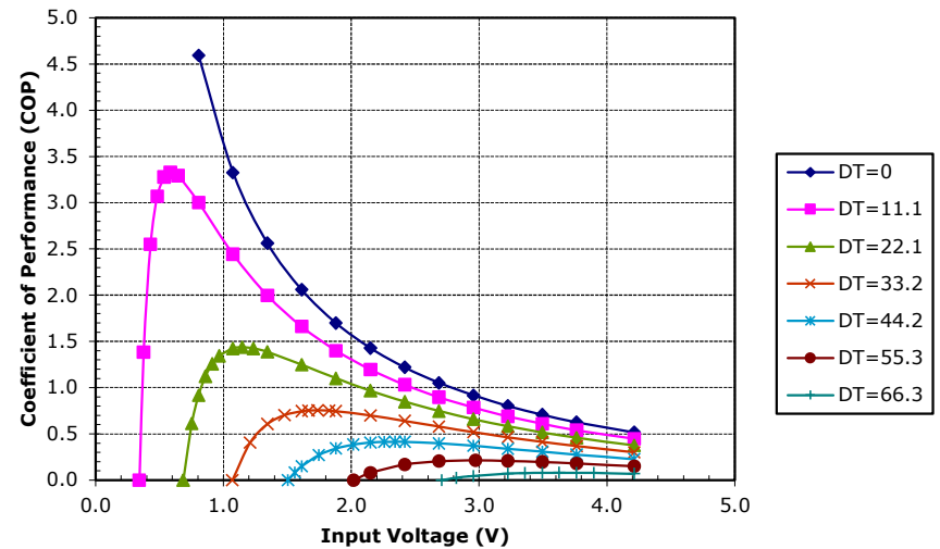
Unpotted TE-31-1.0-1.3 at a hot-side temperature of 50 °C
