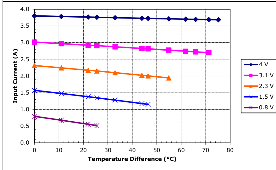
Unpotted VT-31-1.0-1.3 at a hot-side temperature of 50 °C
