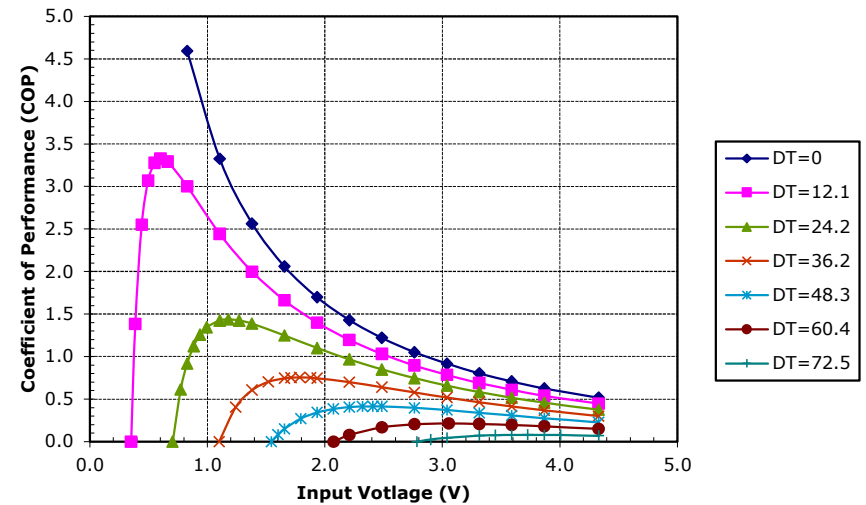
Unpotted VT-31-1.0-1.3 at a hot-side temperature of 70 °C
