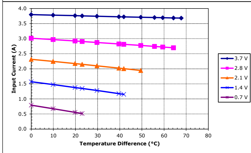
Unpotted VT-31-1.0-1.3 at a hot-side temperature of 30 °C
