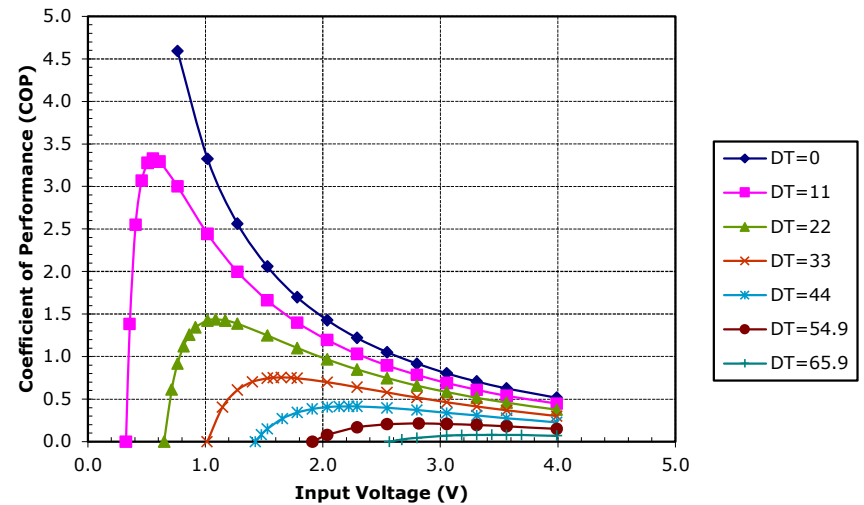
Unpotted VT-31-1.0-1.3 at a hot-side temperature of 50 °C
