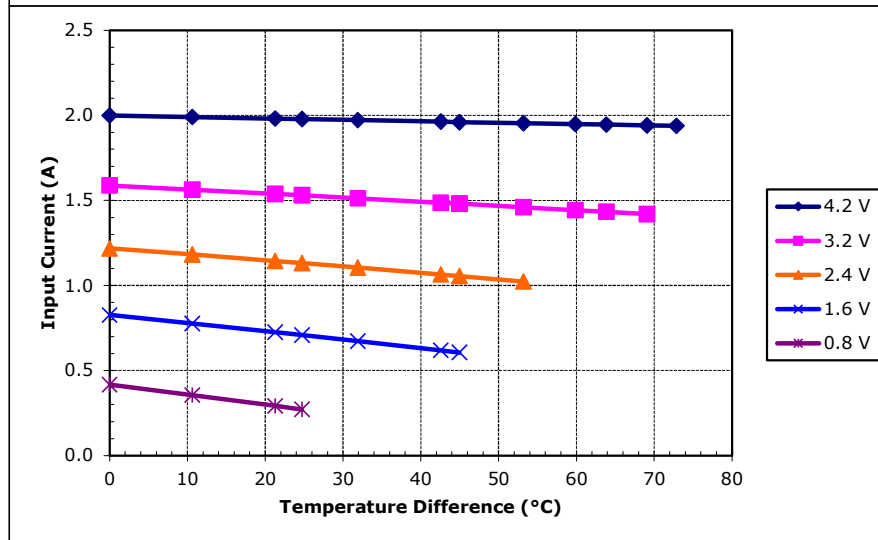
Potted TE-31-1.0-2.5 at a hot-side temperature of 50 °C
