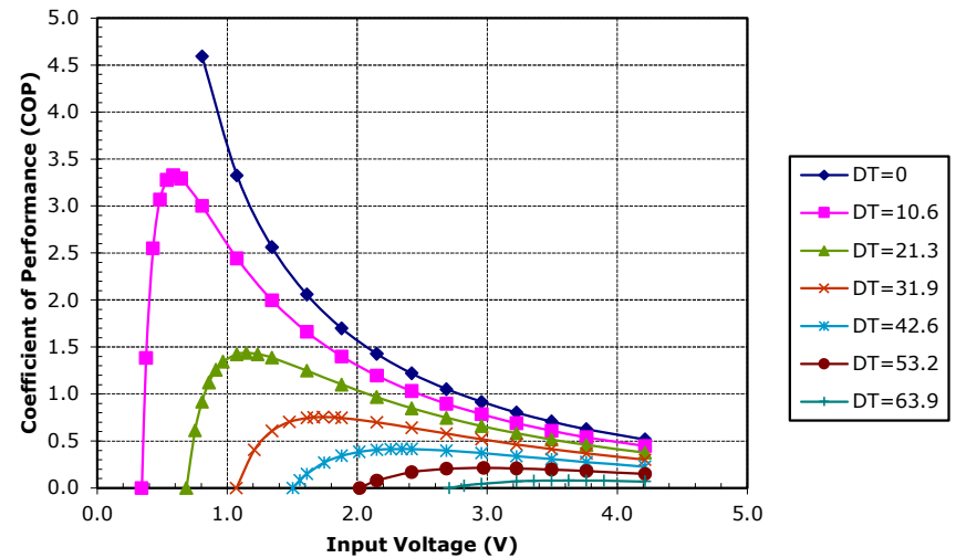
Potted TE-31-1.0-2.5 at a hot-side temperature of 50 °C
