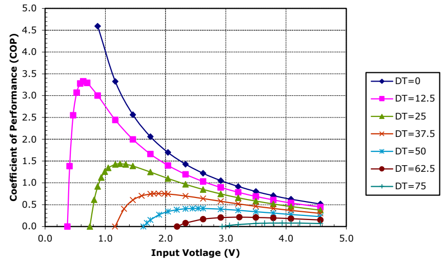
Unpotted TE-31-1.0-2.5 at a hot-side temperature of 70 °C
