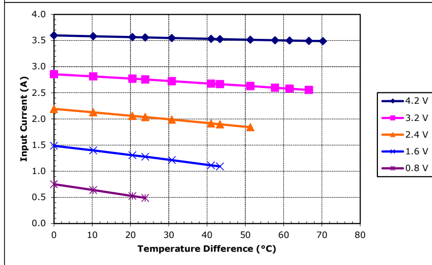
Potted TE-31-1.0-1.3 at a hot-side temperature of 50 °C
