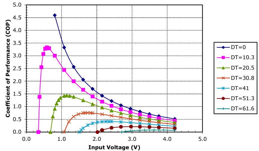
Potted TE-31-1.0-1.3 at a hot-side temperature of 50 °C
