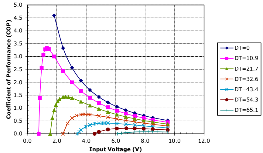
Unpotted VT-71-1.4-1.15 at a hot-side temperature of 50 °C
