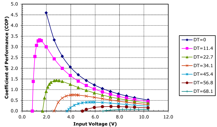
Potted VT-71-1.4-1.15 at a hot-side temperature of 70 °C
