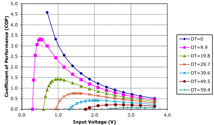
Unpotted VT-31-1.0-1.3 at a hot-side temperature of 30 °C
