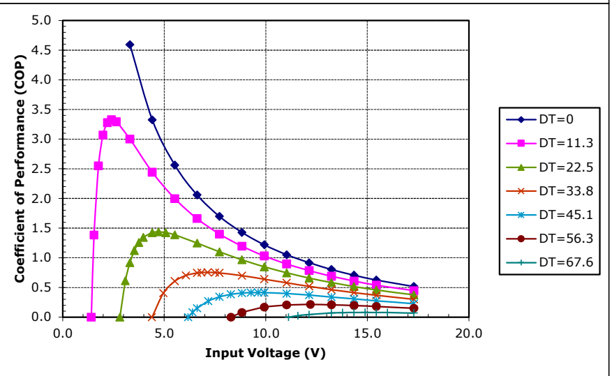
Unpotted VT-127-1.4-1.5-72 at a hot-side temperature of 50 °C
