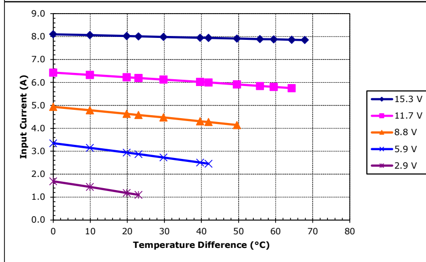
Unpotted VT-127-1.4-1.15-71 at a hot-side temperature of 30 °C
