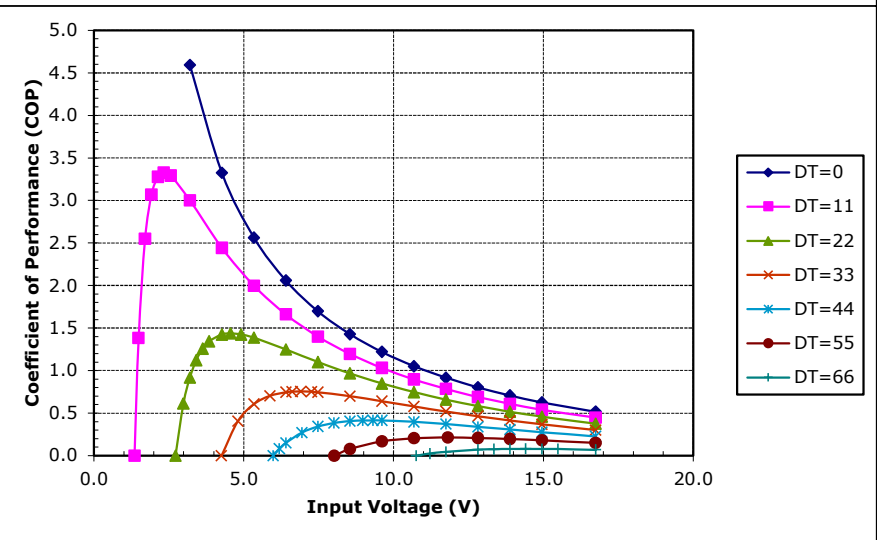
Unpotted VT-127-1.4-1.15-71 at a hot-side temperature of 50 °C
