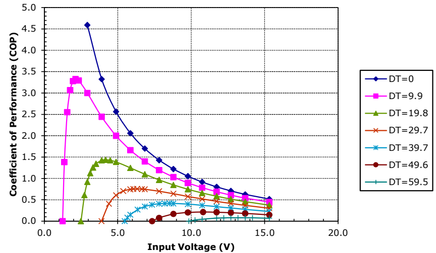
Unpotted VT-127-1.4-1.15-71 at a hot-side temperature of 30 °C
