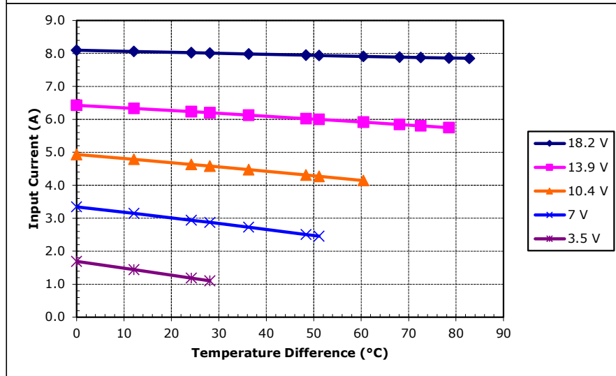
Unpotted VT-127-1.4-1.15-71 at a hot-side temperature of 70 °C
