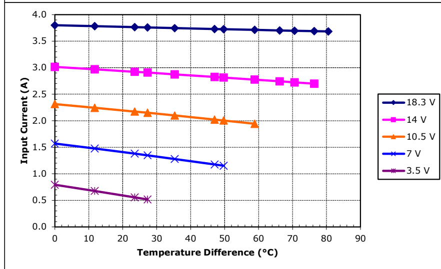
Potted VT-127-1.0-1.3-71 at a hot-side temperature of 70 °C
