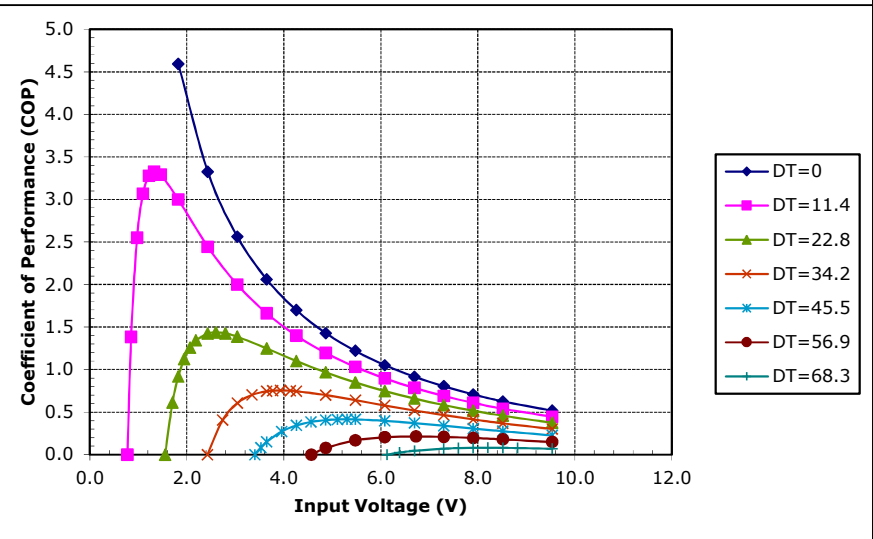
Unpotted TE-71-1.4-2.5 at a hot-side temperature of 50 °C
