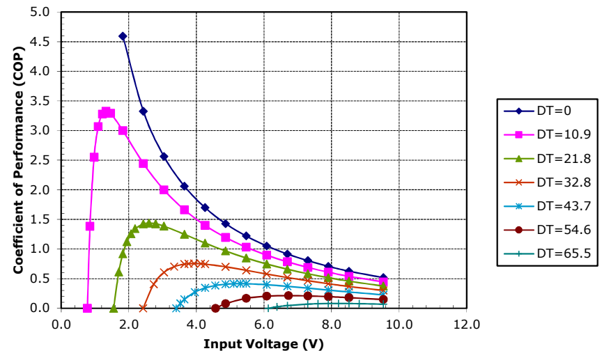
Potted TE-71-1.4-2.5 at a hot-side temperature of 50 °C
