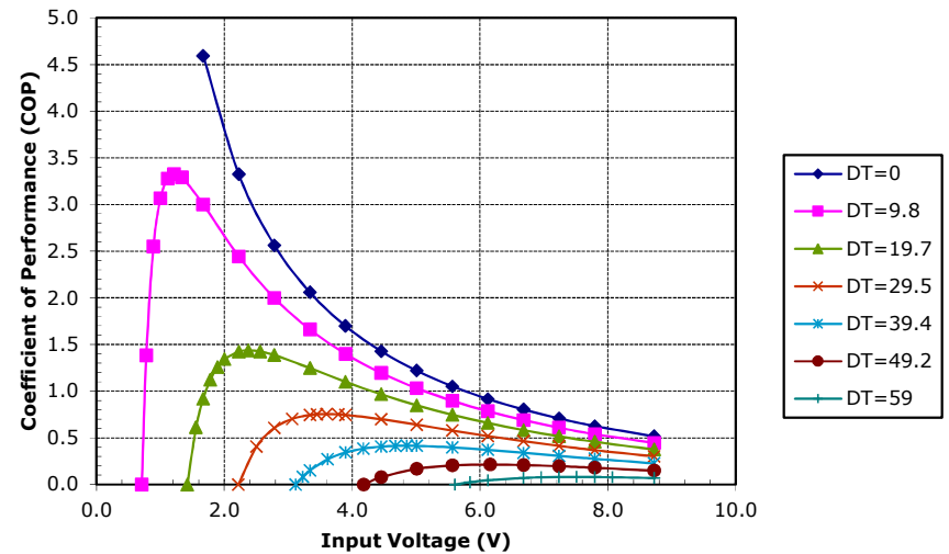
Potted TE-71-1.4-2.5 at a hot-side temperature of 30 °C
