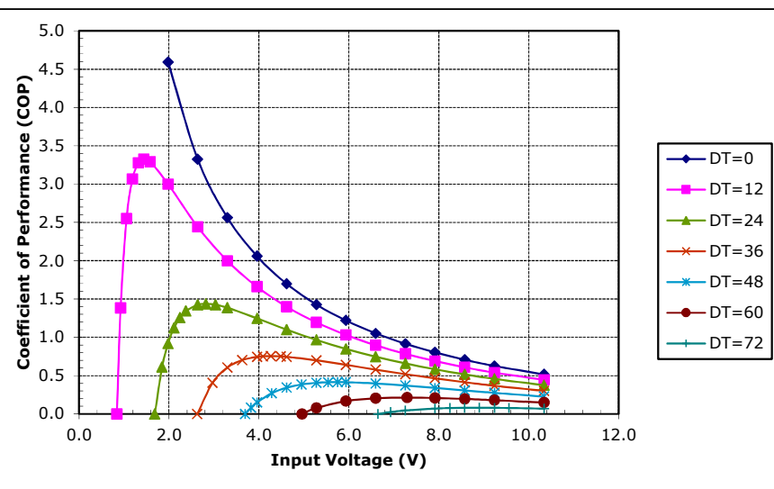
Potted TE-71-1.4-2.5 at a hot-side temperature of 70 °C
