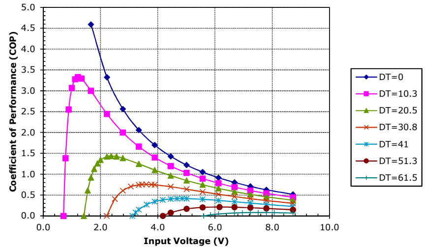
Unpotted TE-71-1.4-2.5 at a hot-side temperature of 30 °C
