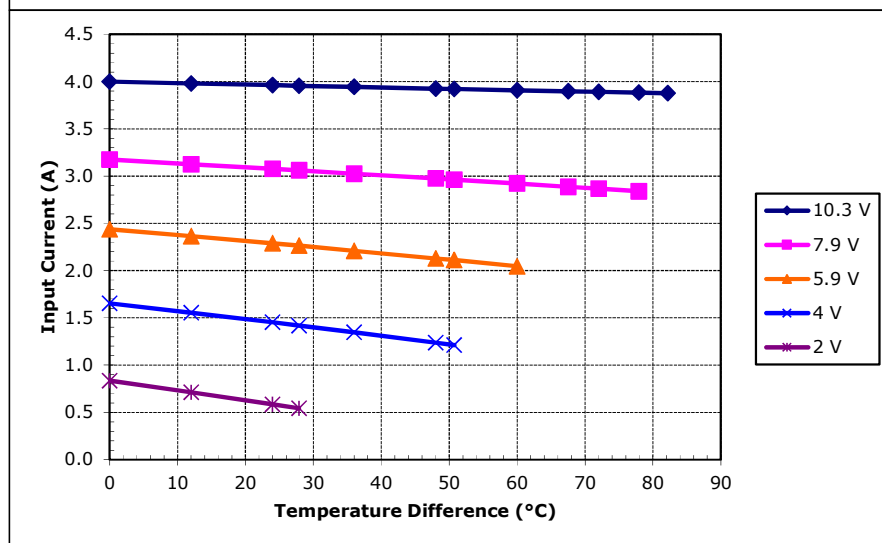
Potted TE-71-1.4-2.5 at a hot-side temperature of 70 °C
