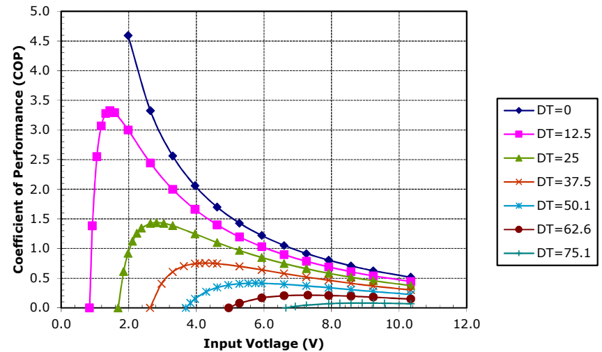
Unpotted TE-71-1.4-2.5 at a hot-side temperature of 70 °C
