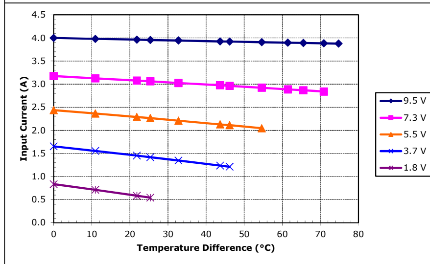
Potted TE-71-1.4-2.5 at a hot-side temperature of 50 °C
