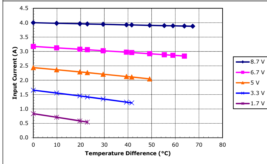
Potted TE-71-1.4-2.5 at a hot-side temperature of 30 °C
