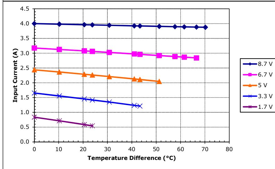
Unpotted TE-71-1.4-2.5 at a hot-side temperature of 30 °C
