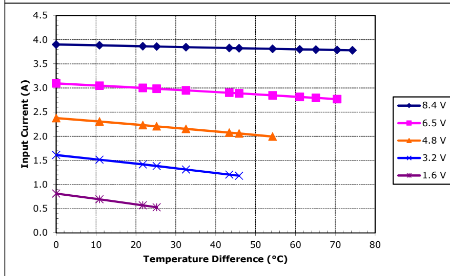
Potted TE-63-1.4-2.5 at a hot-side temperature of 50 °C
