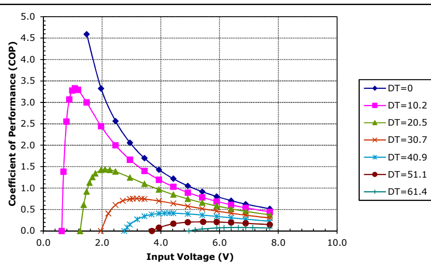
Unpotted TE-63-1.4-2.5 at a hot-side temperature of 30 °C
