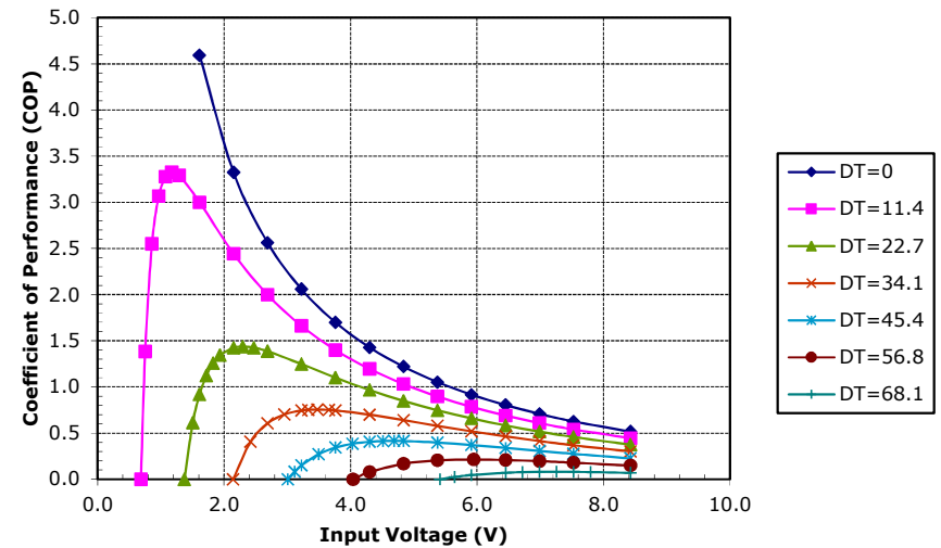
Unpotted TE-63-1.4-2.5 at a hot-side temperature of 50 °C
