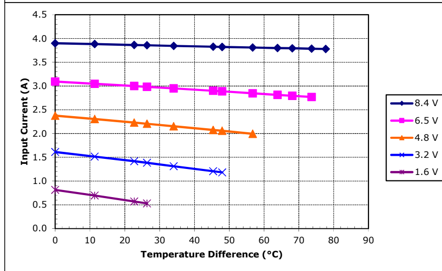
Unpotted TE-63-1.4-2.5 at a hot-side temperature of 50 °C
