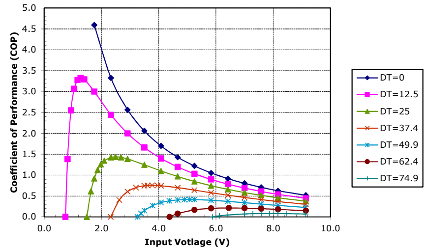
Unpotted TE-63-1.4-2.5 at a hot-side temperature of 70 °C
