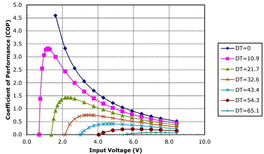
Potted TE-63-1.4-2.5 at a hot-side temperature of 50 °C
