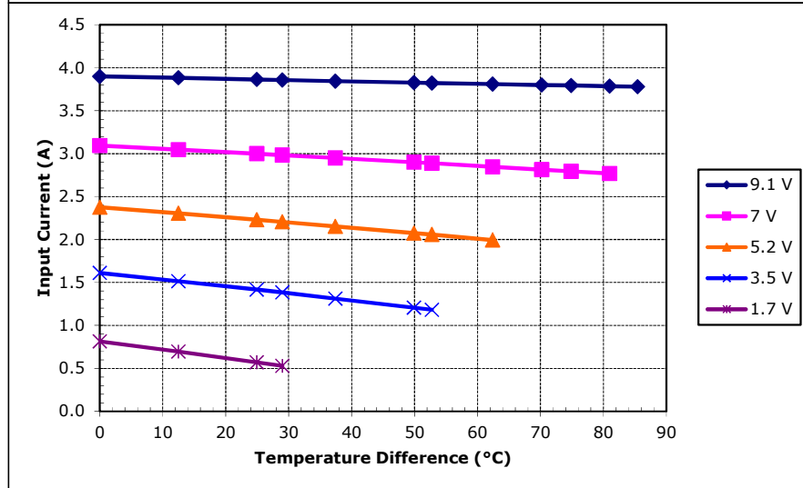
Unpotted TE-63-1.4-2.5 at a hot-side temperature of 70 °C
