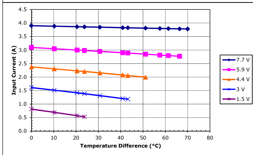
Unpotted TE-63-1.4-2.5 at a hot-side temperature of 30 °C
