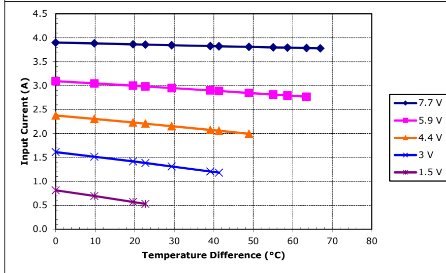
Potted TE-63-1.4-2.5 at a hot-side temperature of 30 °C
