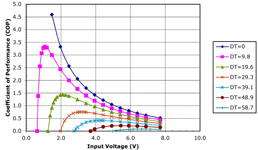
Potted TE-63-1.4-2.5 at a hot-side temperature of 30 °C
