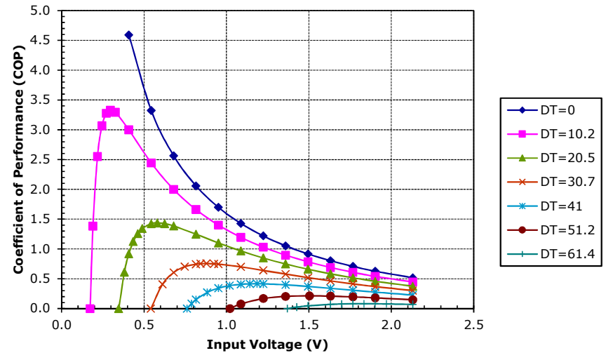
Unpotted TE-17-1.4-2.5 at a hot-side temperature of 30 °C
