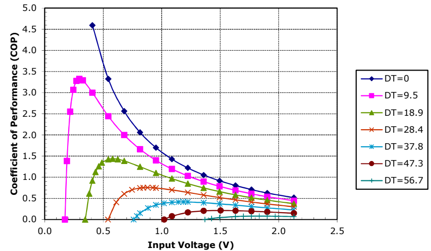
Potted TE-17-1.4-2.5 at a hot-side temperature of 30 °C
