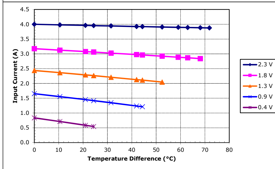
Potted TE-17-1.4-2.5 at a hot-side temperature of 50 °C
