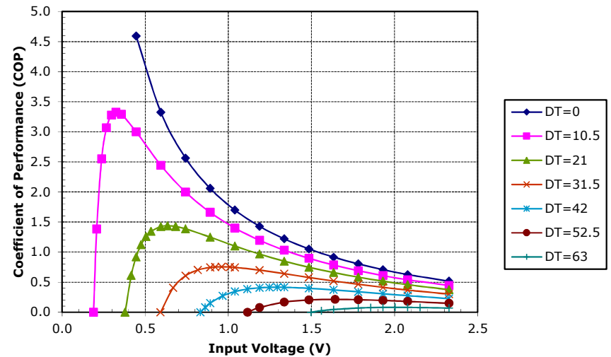
Potted TE-17-1.4-2.5 at a hot-side temperature of 50 °C
