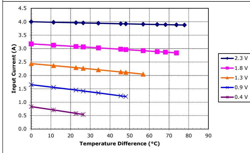
Unpotted TE-17-1.4-2.5 at a hot-side temperature of 50 °C
