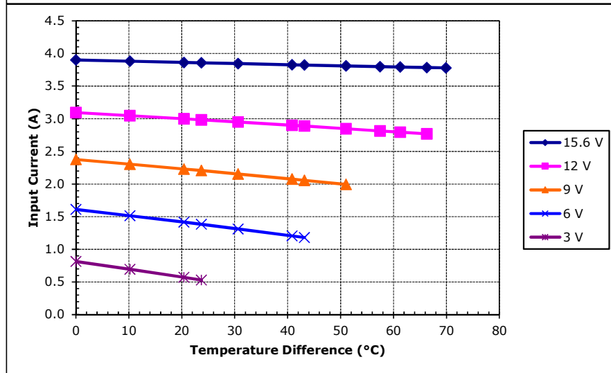
Unpotted HP-127-1.4-2.5-72 at a hot-side temperature of 30 °C
