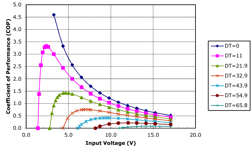
Potted HP-127-1.4-2.5-72 at a hot-side temperature of 50 °C
