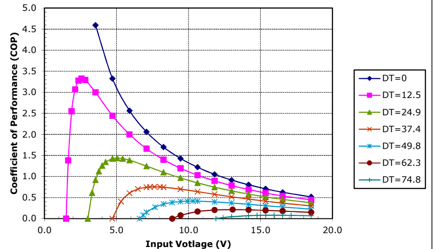
Unpotted HP-127-1.4-2.5-72 at a hot-side temperature of 70 °C
