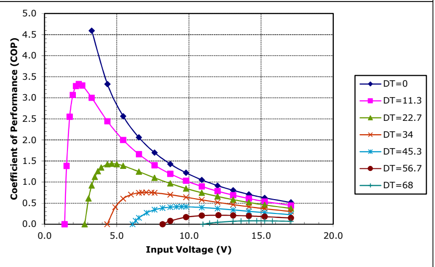
Unpotted HP-127-1.4-2.5-72 at a hot-side temperature of 50 °C
