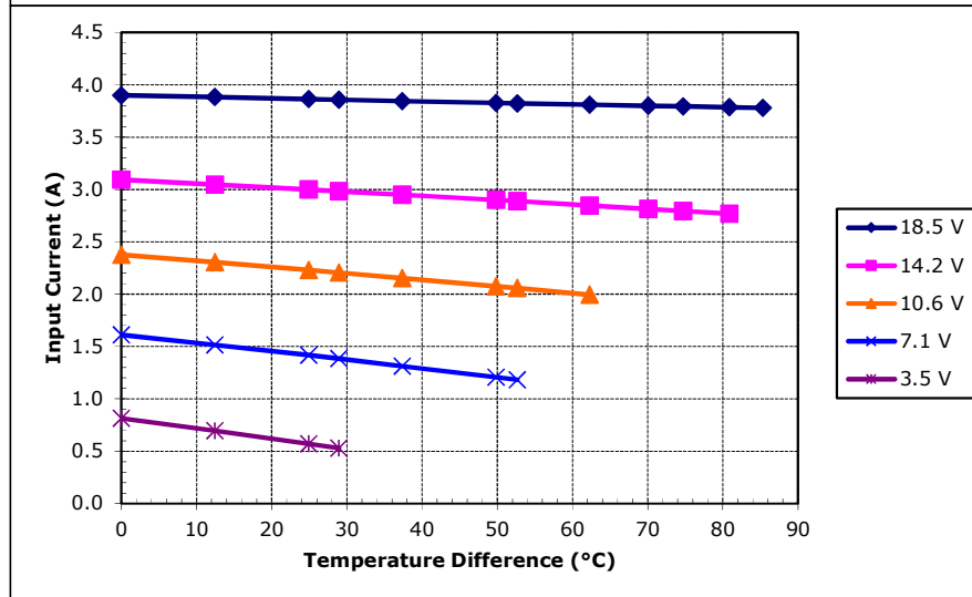
Unpotted HP-127-1.4-2.5-72 at a hot-side temperature of 70 °C
