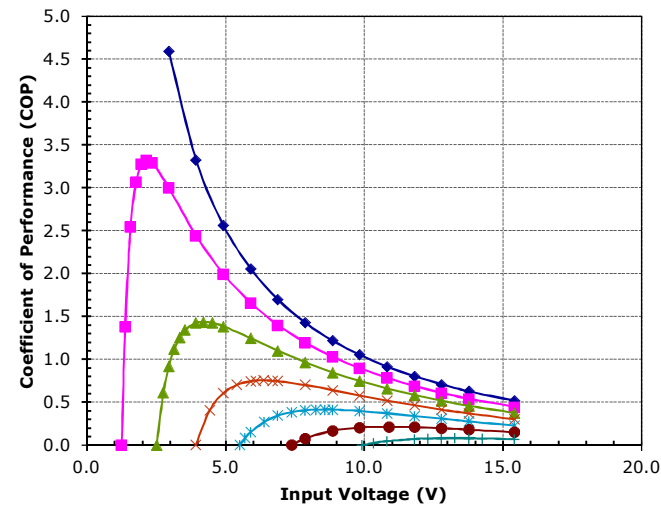
Unpotted VT-127-1.0-1.3-71 at a hot-side temperature of 30 °C
