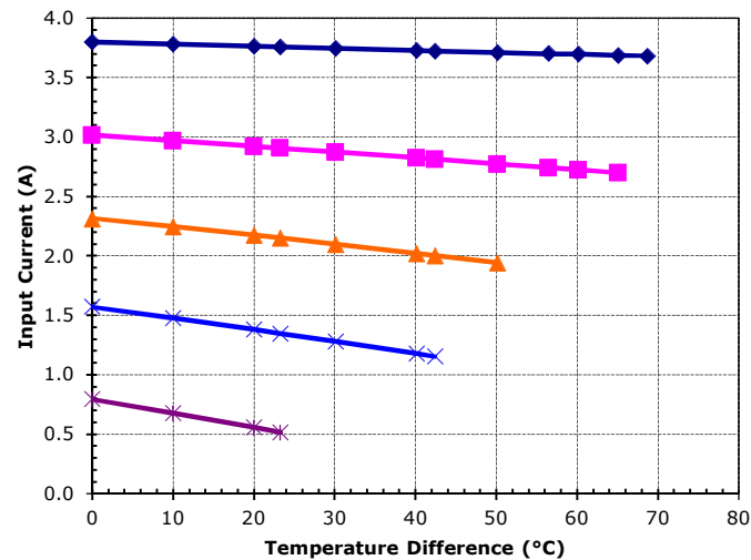
Unpotted VT-127-1.0-1.3-71 at a hot-side temperature of 30 °C
