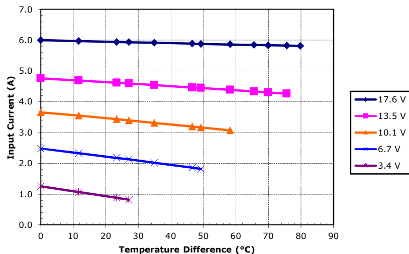
Unpotted HP-127-1.4-1.5-74 at a hot-side temperature of 50 °C
