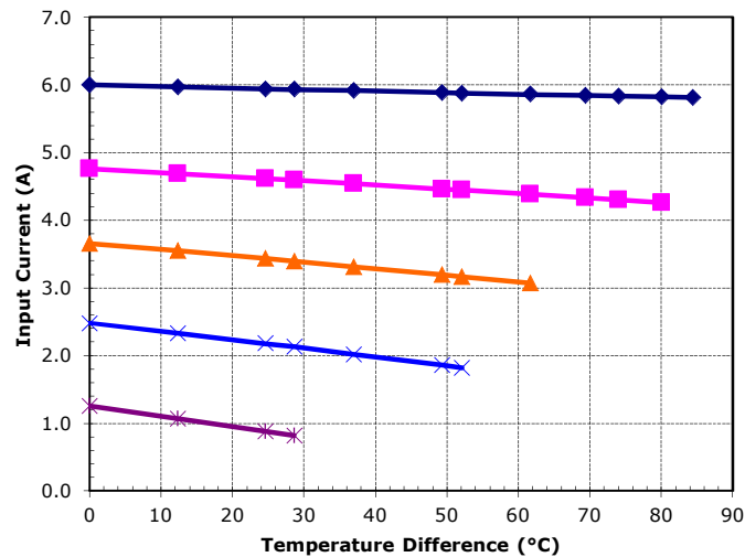
Potted HP-127-1.4-1.5-74 at a hot-side temperature of 70 °C
