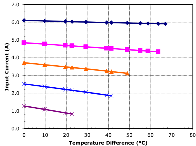
Potted HP-127-1.4-1.5-72 at a hot-side temperature of 30 °C
