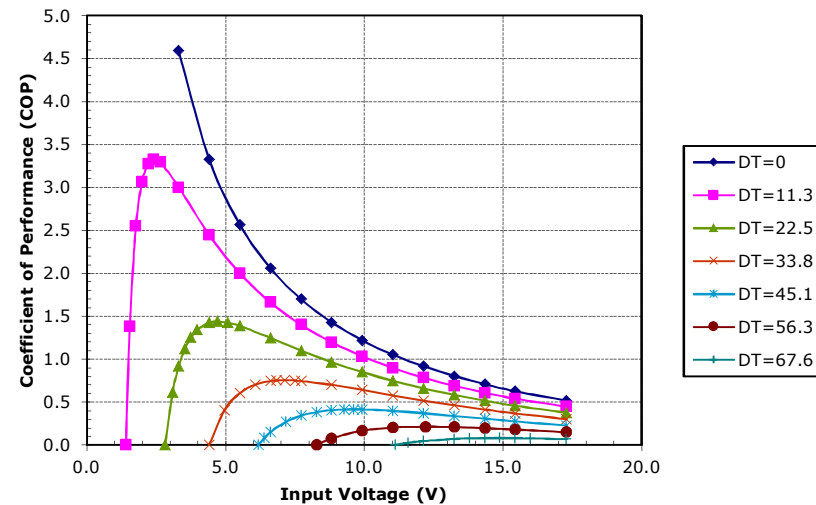
Unpotted HP-127-1.4-1.5-72 at a hot-side temperature of 50 °C
