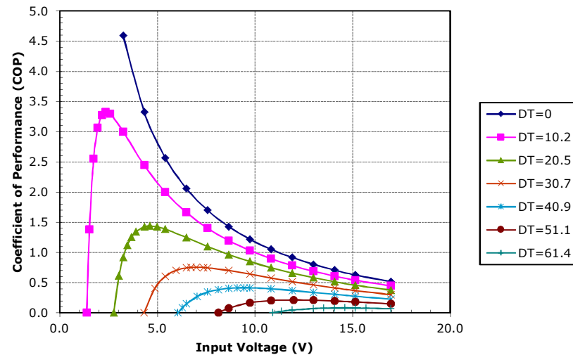
Potted HP-127-1.0-0.8 at a hot-side temperature of 50 °C
