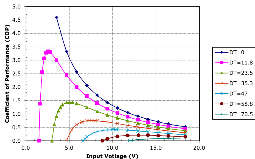
Unpotted HP-127-1.0-0.8 at a hot-side temperature of 70 °C
