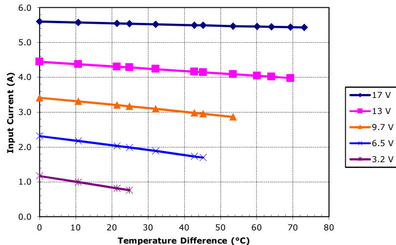
Unpotted HP-127-1.0-0.8 at a hot-side temperature of 50 °C
