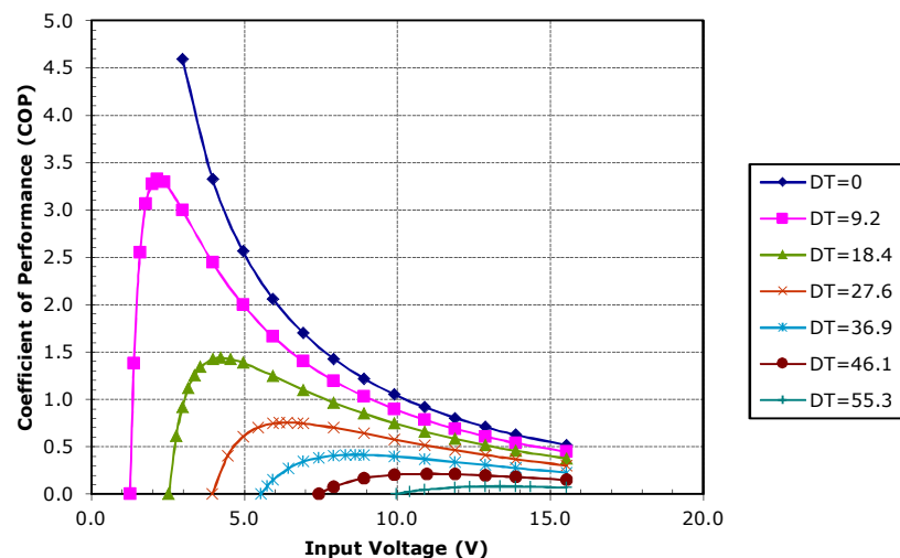
Potted HP-127-1.0-0.8 at a hot-side temperature of 30 °C
