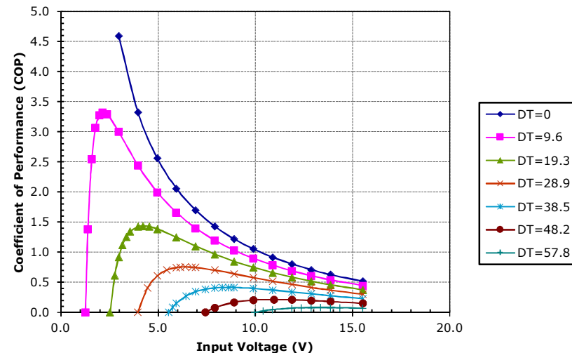
Unpotted HP-127-1.0-0.8 at a hot-side temperature of 30 °C
