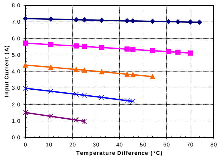
Potted SP-254-1.0-1.3 (Parallel) at a hot-side temperature of 50 °C
