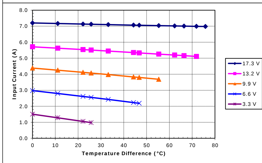
Unpotted SP-254-1.0-1.3 (Parallel) at a hot-side temperature of 50 °C
