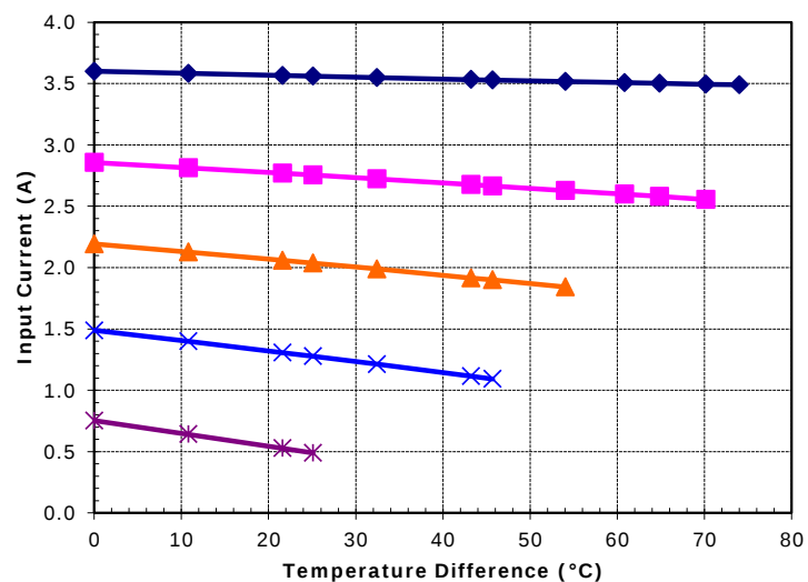
Potted SP-254-1.0-1.3 (Series) at a hot-side temperature of 50 °C
