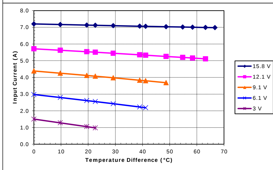
Potted SP-254-1.0-1.3 (Parallel) at a hot-side temperature of 30 °C
