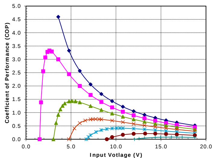
Unpotted SP-254-1.0-1.3 (Parallel) at a hot-side temperature of 70 °C
