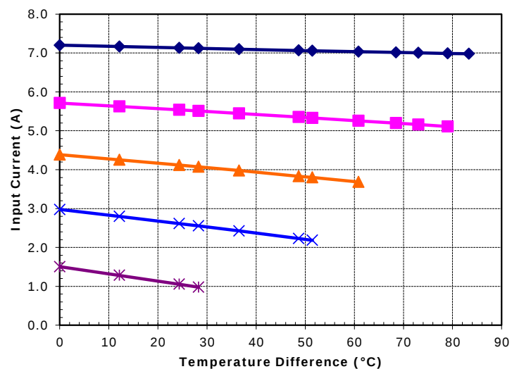
Unpotted SP-254-1.0-1.3 (Parallel) at a hot-side temperature of 70 °C
