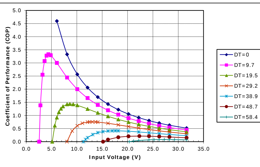
Potted SP-254-1.0-1.3 (Series) at a hot-side temperature of 30 °C
