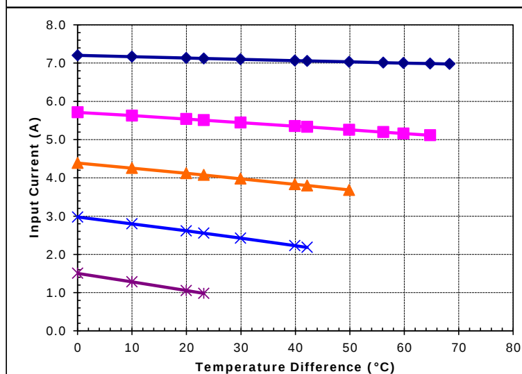
Unpotted SP-254-1.0-1.3 (Parallel) at a hot-side temperature of 30 °C
