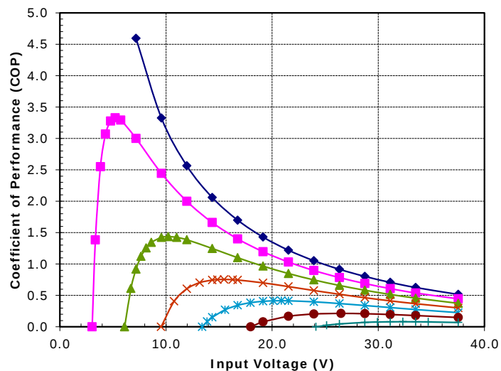
Potted SP-254-1.0-1.3 (Series) at a hot-side temperature of 70 °C
