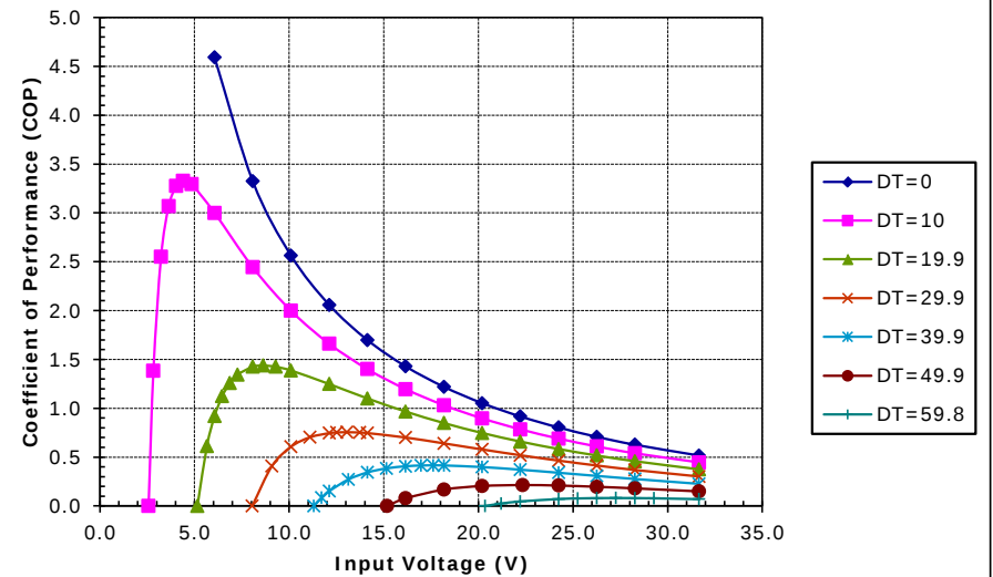
Unpotted SP-254-1.0-1.3 (Series) at a hot-side temperature of 30 °C
