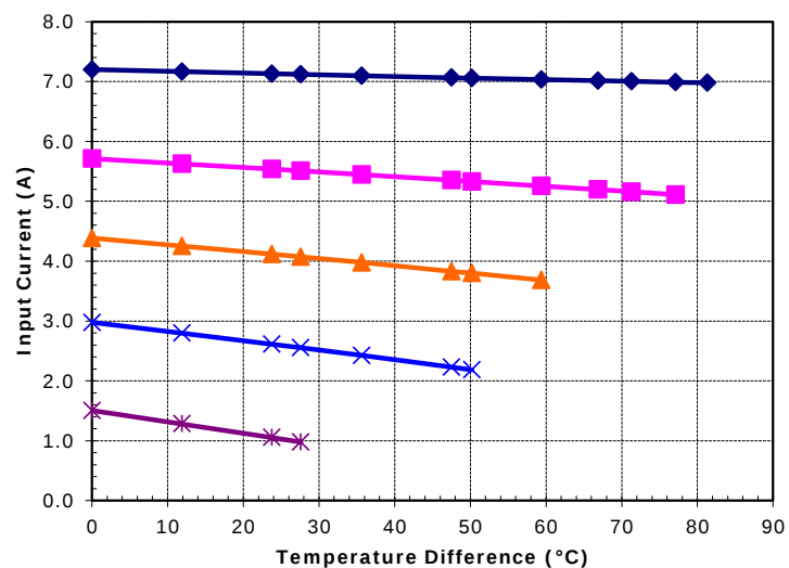
Potted SP-254-1.0-1.3 (Parallel) at a hot-side temperature of 70 °C
