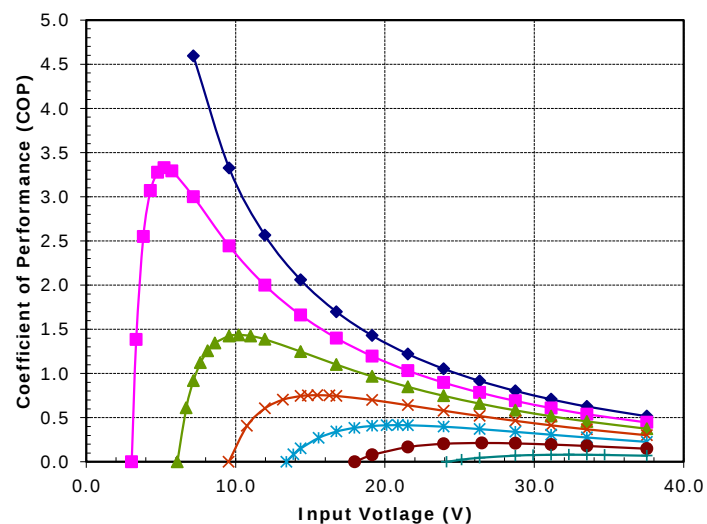
Unpotted SP-254-1.0-1.3 (Series) at a hot-side temperature of 70 °C
