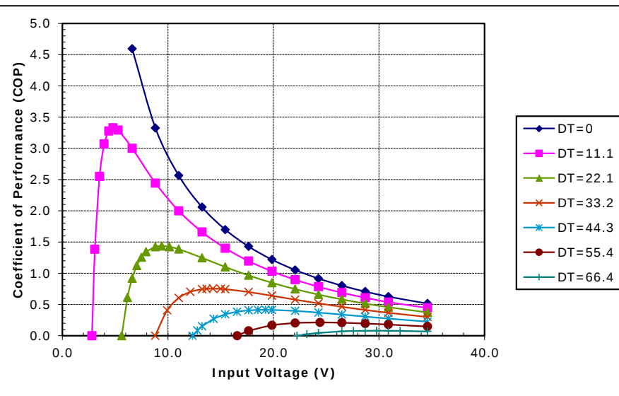
Unpotted SP-254-1.0-1.3 (Series) at a hot-side temperature of 50 °C
