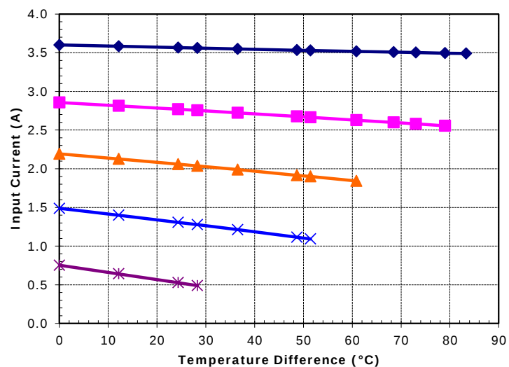
Unpotted SP-254-1.0-1.3 (Series) at a hot-side temperature of 70 °C
