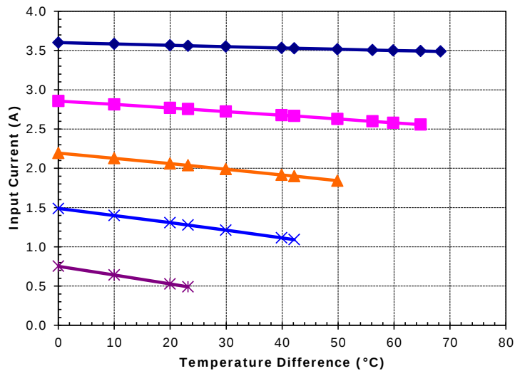
Unpotted SP-254-1.0-1.3 (Series) at a hot-side temperature of 30 °C
