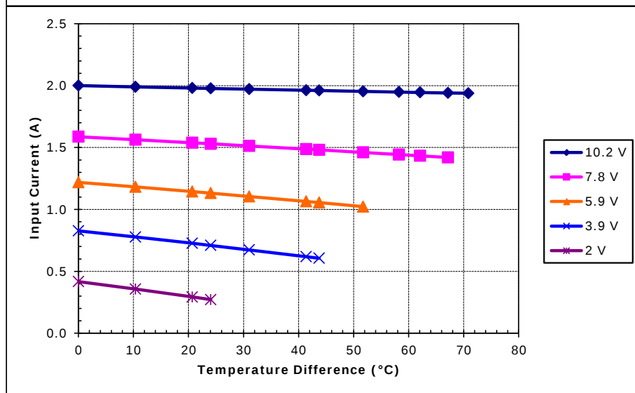
Unpotted TE-83-1.0-2.5 at a hot-side temperature of 30 °C
