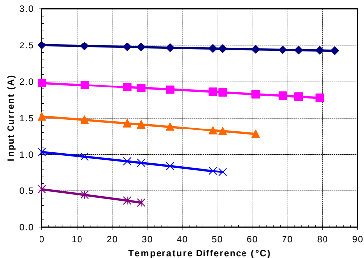
Potted TE-83-1.0-2.0 at a hot-side temperature of 70 °C
