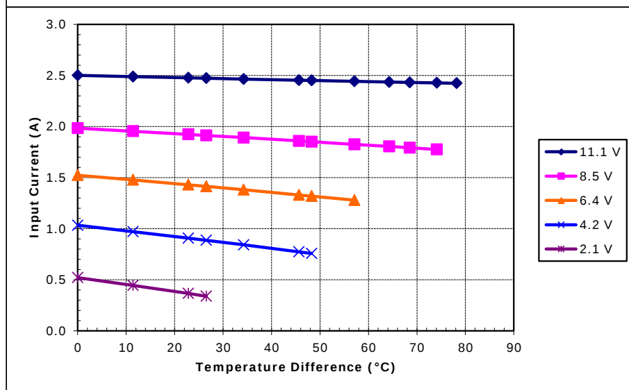
Unpotted TE-83-1.0-2.0 at a hot-side temperature of 50 °C
