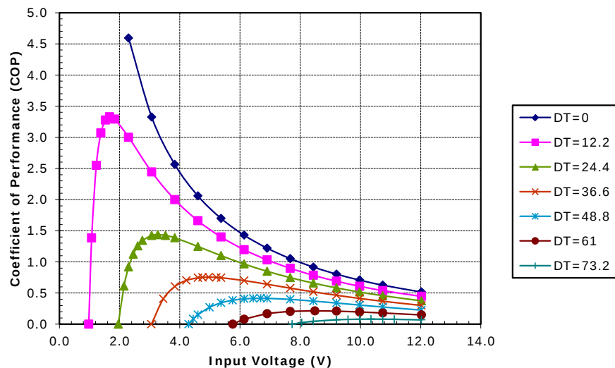
Potted TE-83-1.0-2.0 at a hot-side temperature of 70 °C
