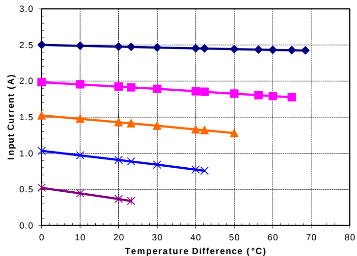
Potted TE-83-1.0-2.0 at a hot-side temperature of 30 °C
