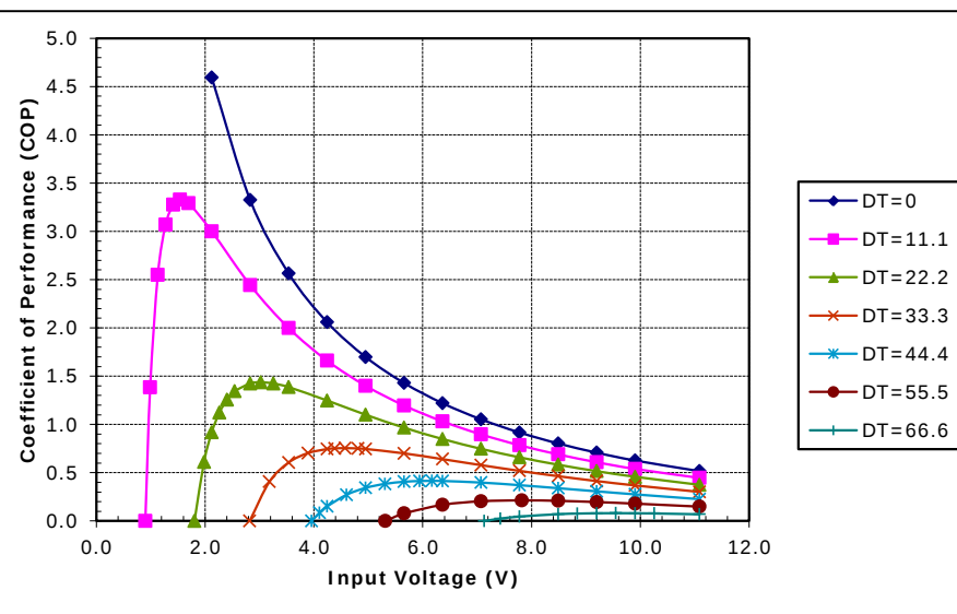
Potted TE-83-1.0-2.0 at a hot-side temperature of 50 °C
