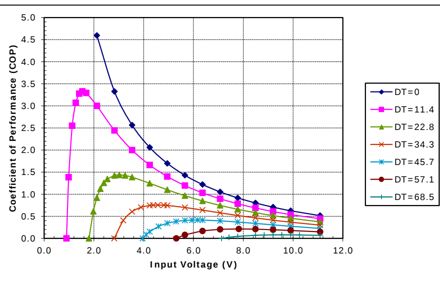
Unpotted TE-83-1.0-2.0 at a hot-side temperature of 50 °C
