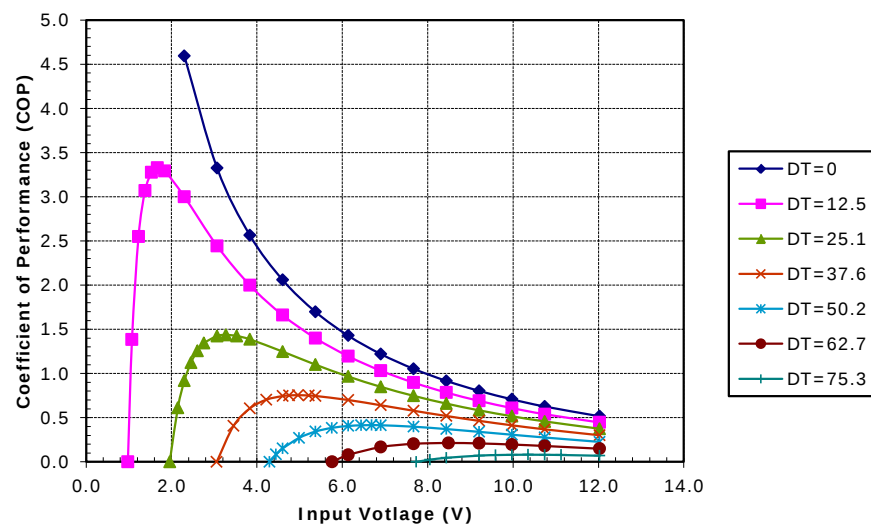
Unpotted TE-83-1.0-2.0 at a hot-side temperature of 70 °C
