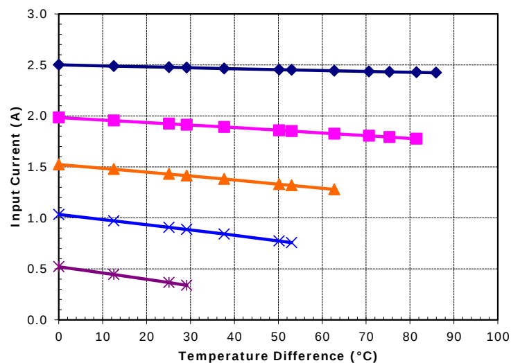
Unpotted TE-83-1.0-2.0 at a hot-side temperature of 70 °C
