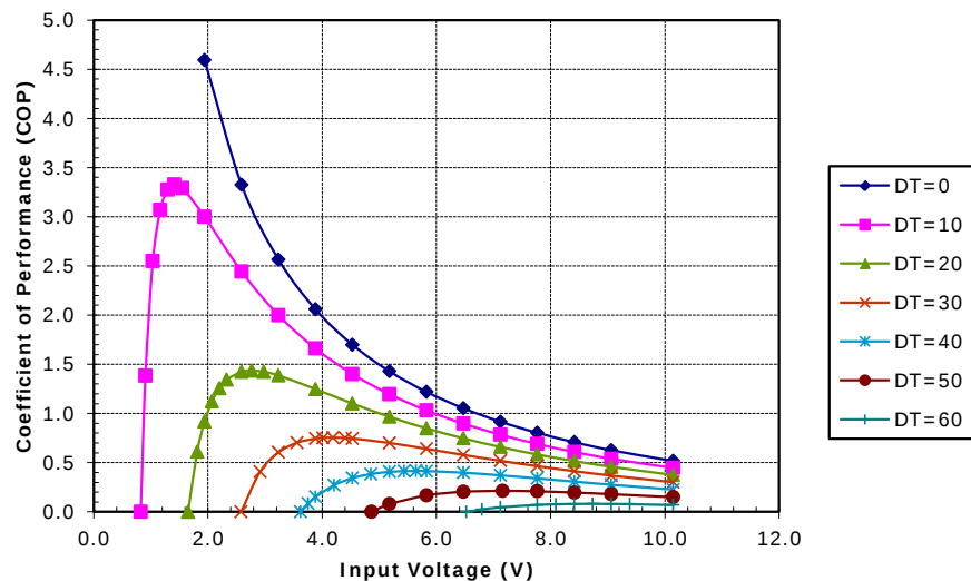
Potted TE-83-1.0-2.0 at a hot-side temperature of 30 °C
