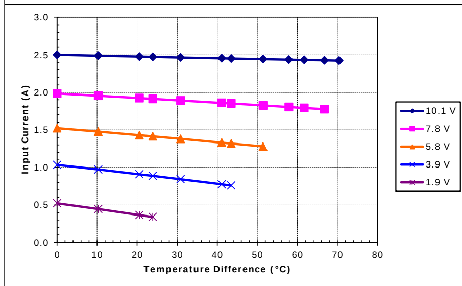
Unpotted TE-83-1.0-2.0 at a hot-side temperature of 30 °C
