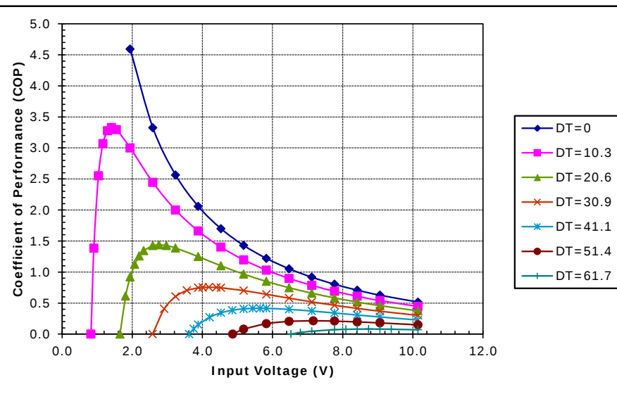
Unpotted TE-83-1.0-2.0 at a hot-side temperature of 30 °C
