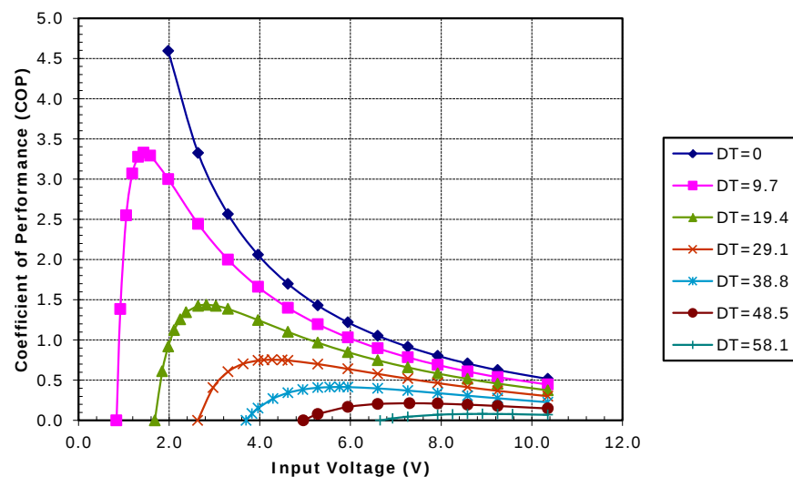
Potted TE-83-1.0-1.3 at a hot-side temperature of 30 °C
