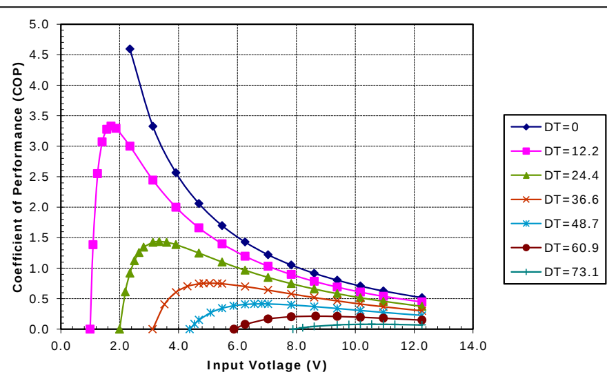
Unpotted TE-83-1.0-1.3 at a hot-side temperature of 70 °C
