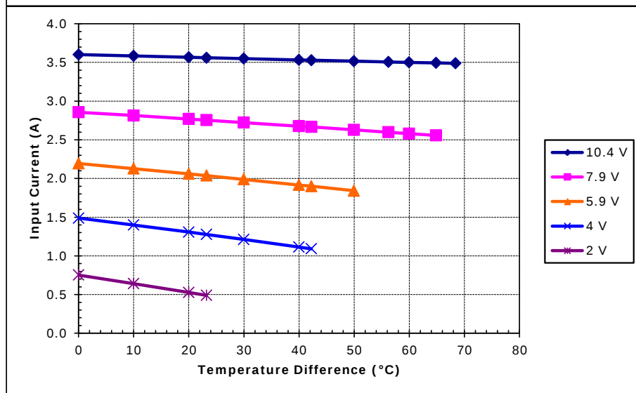
Unpotted TE-83-1.0-1.3 at a hot-side temperature of 30 °C
