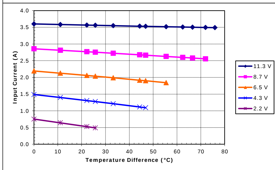
Unpotted TE-83-1.0-1.3 at a hot-side temperature of 50 °C
