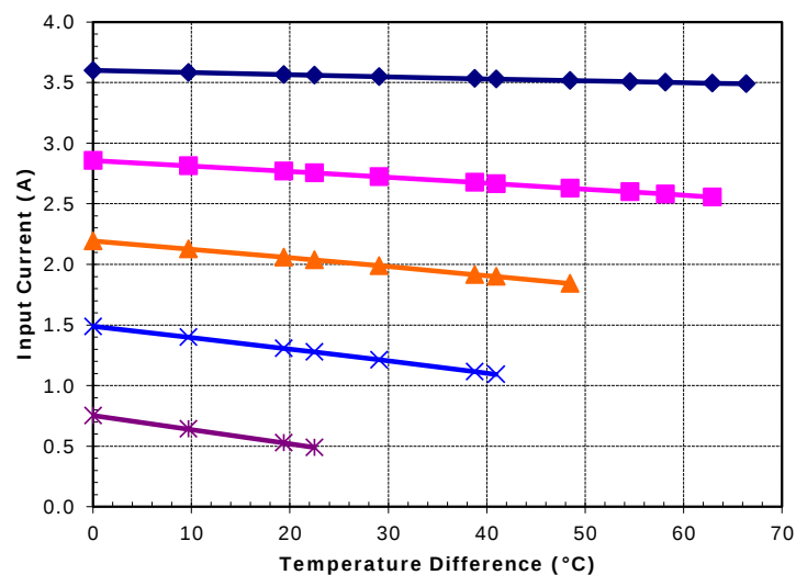
Potted TE-83-1.0-1.3 at a hot-side temperature of 30 °C
