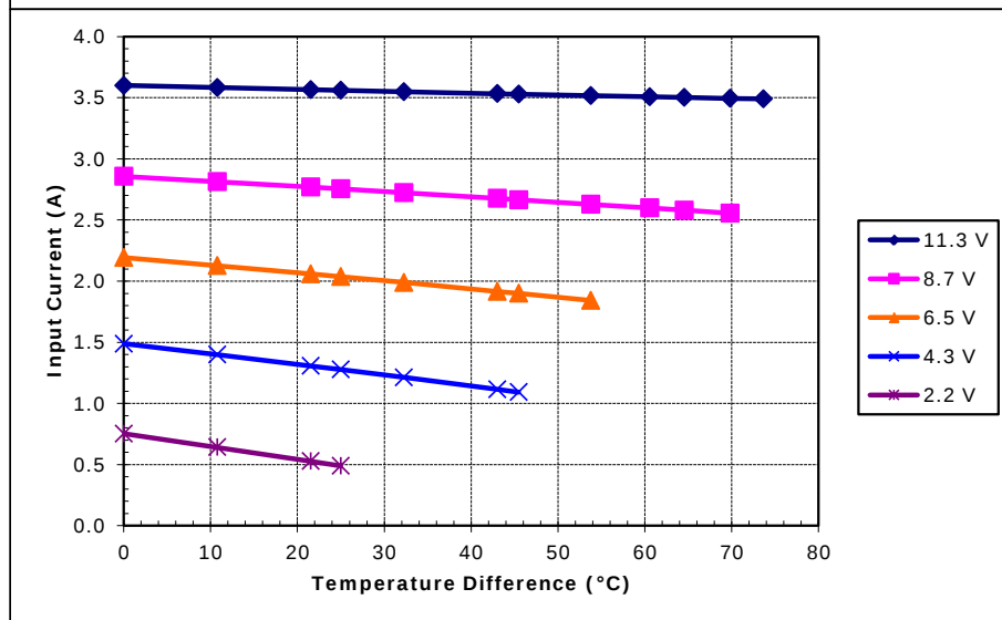
Potted TE-83-1.0-1.3 at a hot-side temperature of 50 °C
