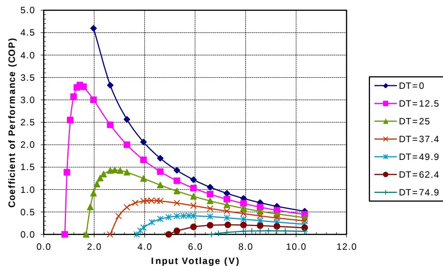
Unpotted TE-71-2.0-2.5 at a hot-side temperature of 70 °C
