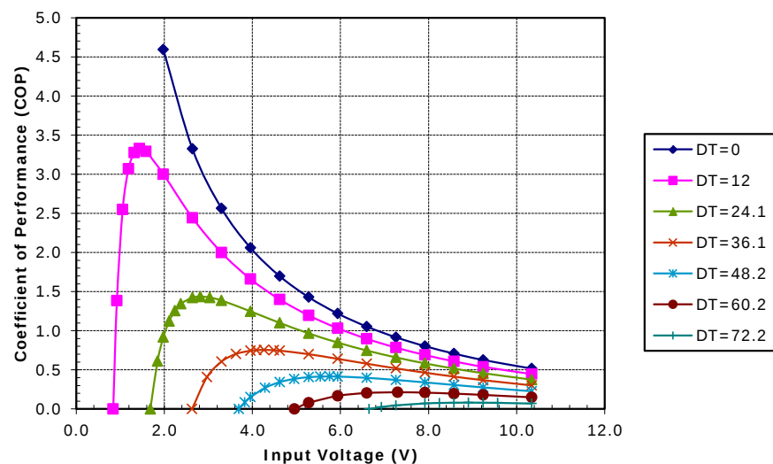
Potted TE-71-2.0-2.5 at a hot-side temperature of 70 °C
