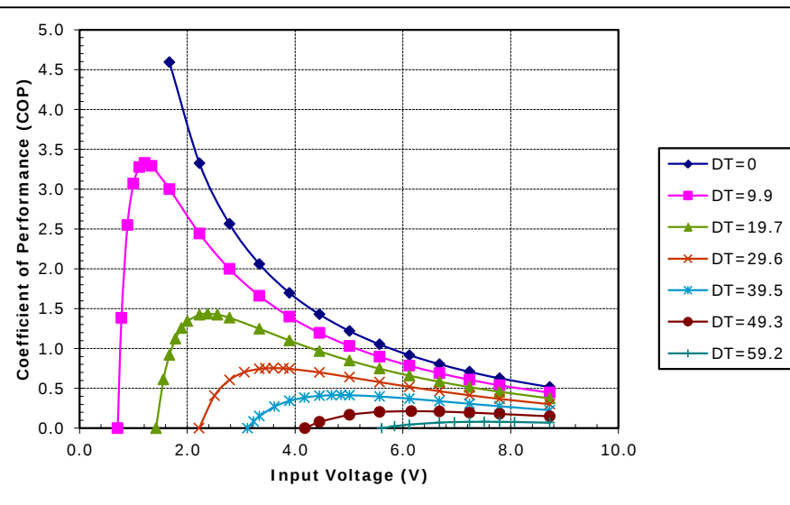
Potted TE-71-2.0-2.5 at a hot-side temperature of 30 °C
