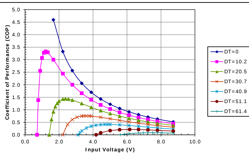
Unpotted TE-71-2.0-2.5 at a hot-side temperature of 30 °C
