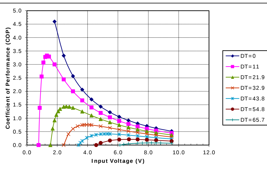
Potted TE-71-2.0-2.5 at a hot-side temperature of 50 °C
