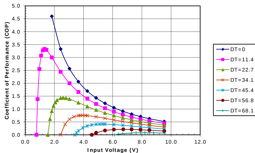
Unpotted TE-71-2.0-2.5 at a hot-side temperature of 50 °C
