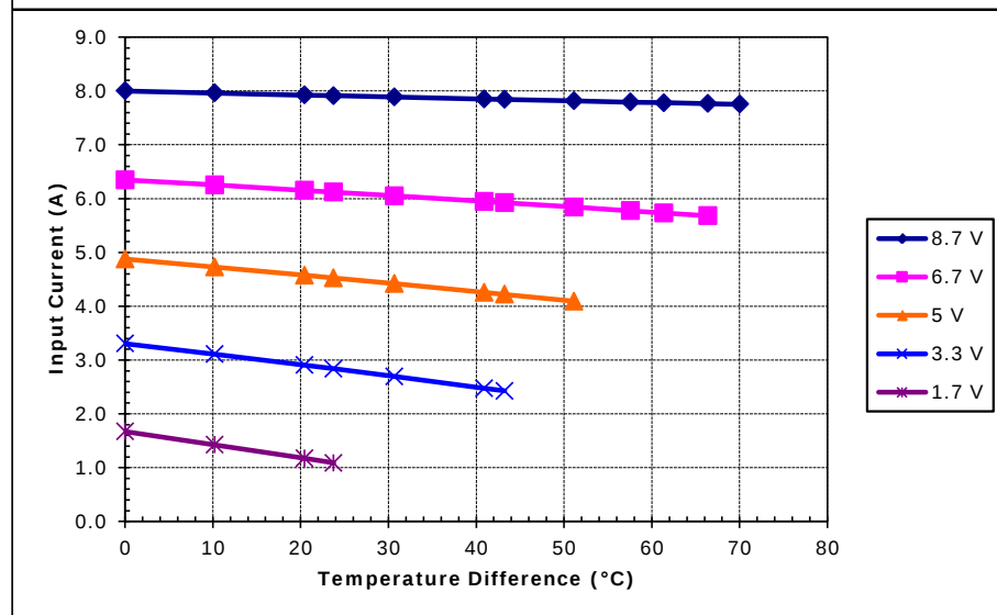
Unpotted TE-71-2.0-2.5 at a hot-side temperature of 30 °C
