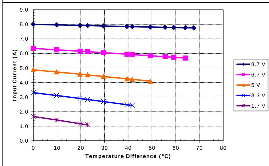
Potted TE-71-2.0-2.5 at a hot-side temperature of 30 °C
