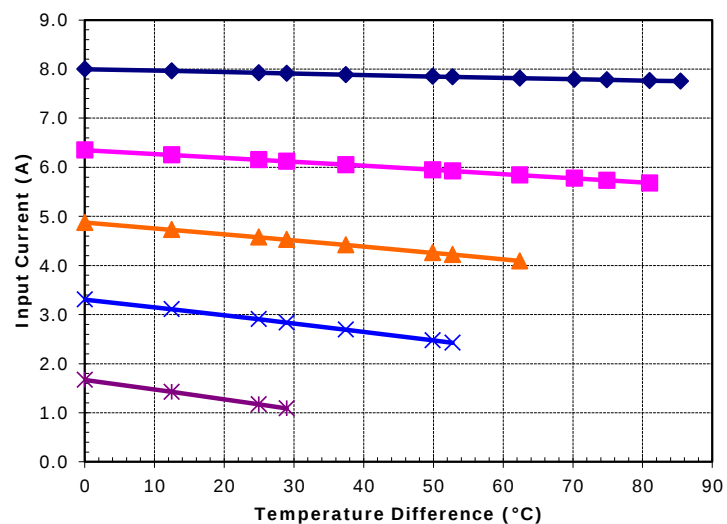
Unpotted TE-71-2.0-2.5 at a hot-side temperature of 70 °C
