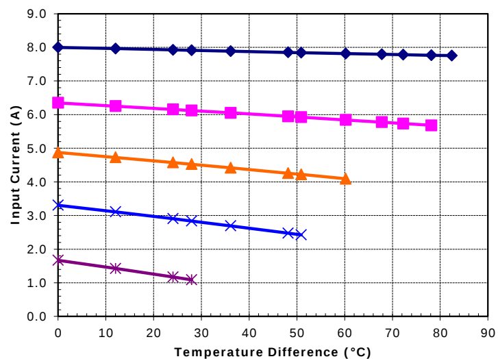
Potted TE-71-2.0-2.5 at a hot-side temperature of 70 °C
