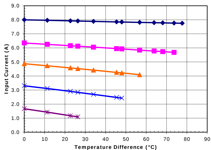
Unpotted TE-71-2.0-2.5 at a hot-side temperature of 50 °C
