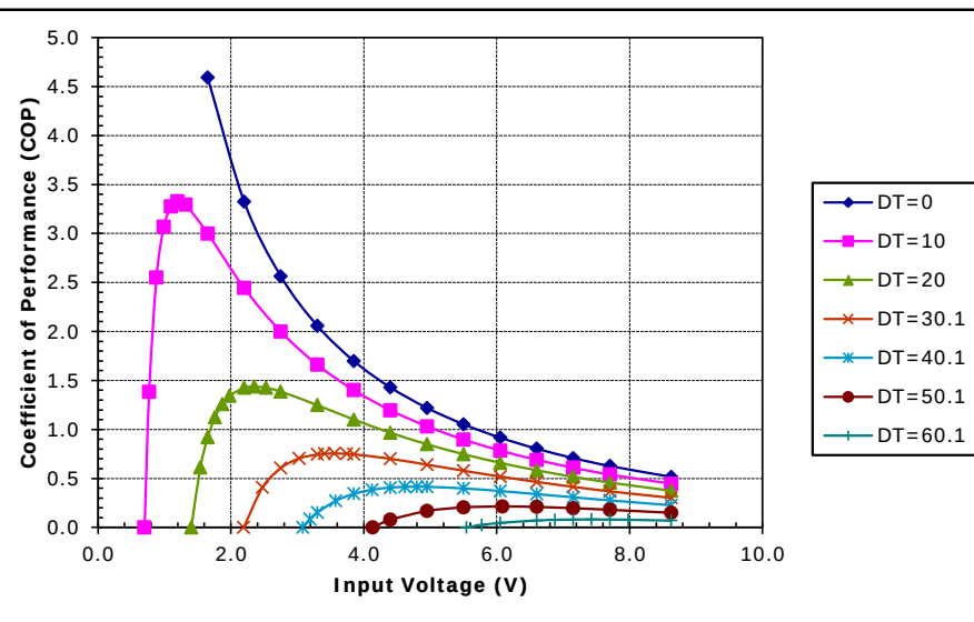
Unpotted TE-71-2.0-1.5 at a hot-side temperature of 30 °C
