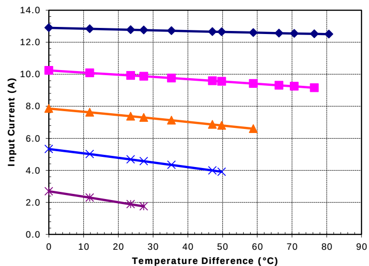
Potted TE-71-2.0-1.5 at a hot-side temperature of 70 °C
