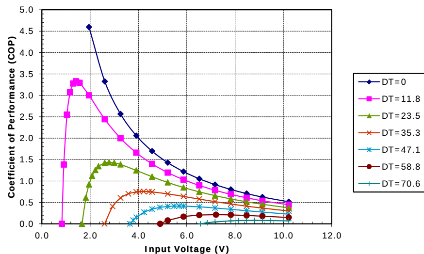
Potted TE-71-2.0-1.5 at a hot-side temperature of 70 °C
