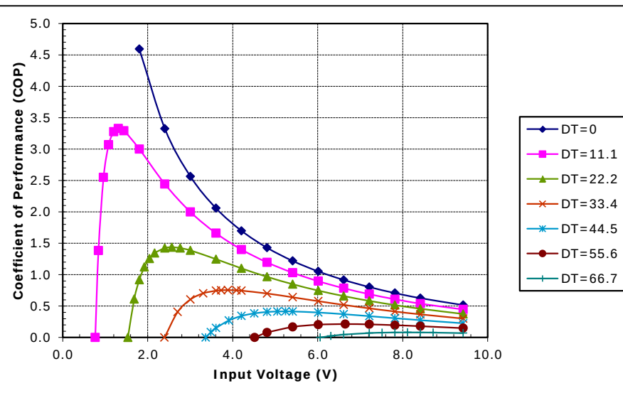
Unpotted TE-71-2.0-1.5 at a hot-side temperature of 50 °C
