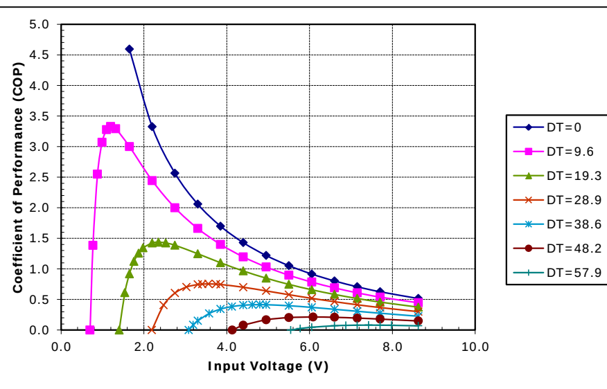
Potted TE-71-2.0-1.5 at a hot-side temperature of 30 °C
