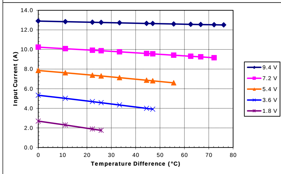
Unpotted TE-71-2.0-1.5 at a hot-side temperature of 50 °C
