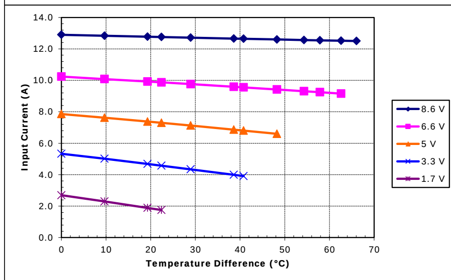
Potted TE-71-2.0-1.5 at a hot-side temperature of 30 °C
