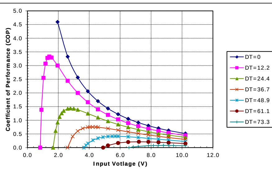
Unpotted TE-71-2.0-1.5 at a hot-side temperature of 70 °C
