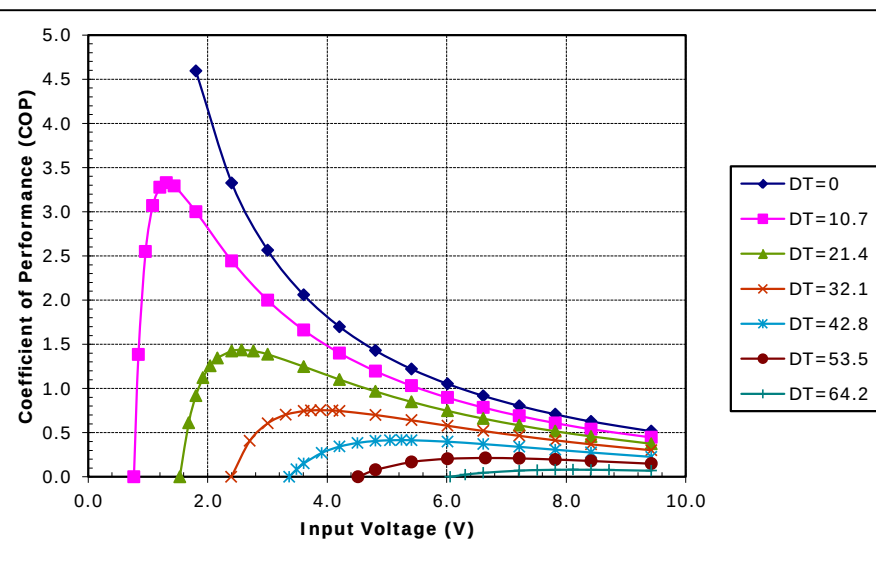
Potted TE-71-2.0-1.5 at a hot-side temperature of 50 °C
