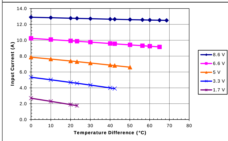
Unpotted TE-71-2.0-1.5 at a hot-side temperature of 30 °C
