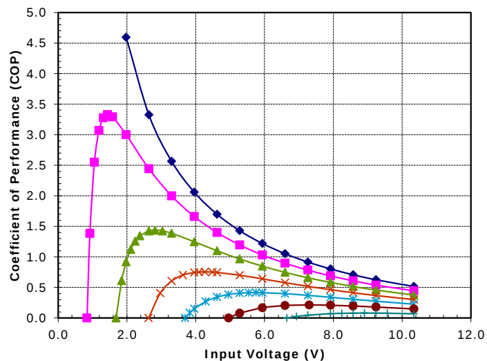
Potted TE-71-2.0-1.15 at a hot-side temperature of 70 °C
