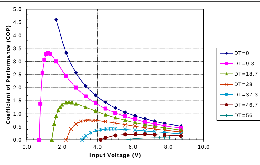
Potted TE-71-2.0-1.15 at a hot-side temperature of 30 °C
