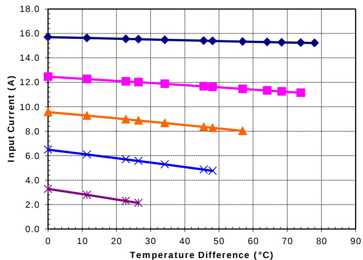
Potted TE-71-2.0-1.15 at a hot-side temperature of 70 °C
