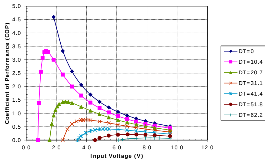
Potted TE-71-2.0-1.15 at a hot-side temperature of 50 °C
