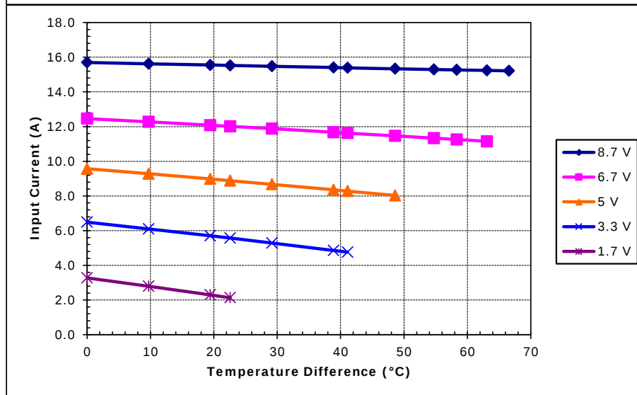
Unpotted TE-71-2.0-1.15 at a hot-side temperature of 30 °C
