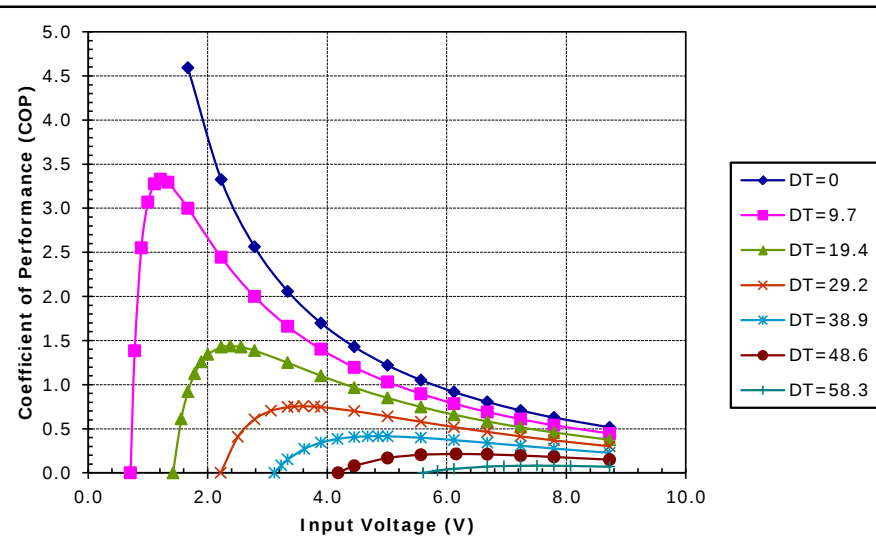
Unpotted TE-71-2.0-1.15 at a hot-side temperature of 30 °C
