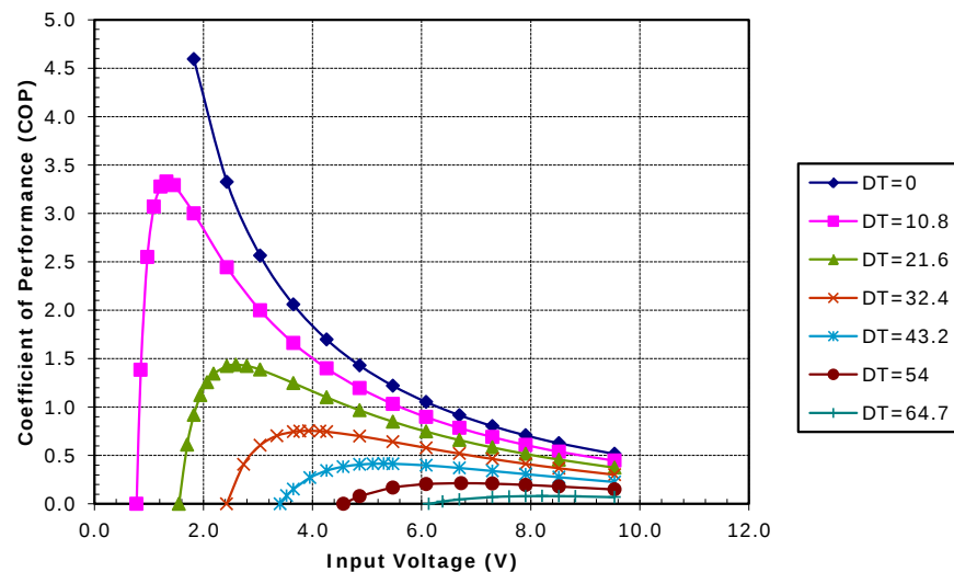
Unpotted TE-71-2.0-1.15 at a hot-side temperature of 50 °C
