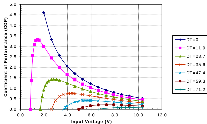
Unpotted TE-71-2.0-1.15 at a hot-side temperature of 70 °C
