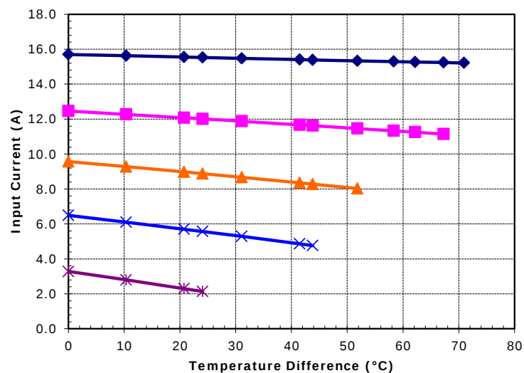
Potted TE-71-2.0-1.15 at a hot-side temperature of 50 °C
