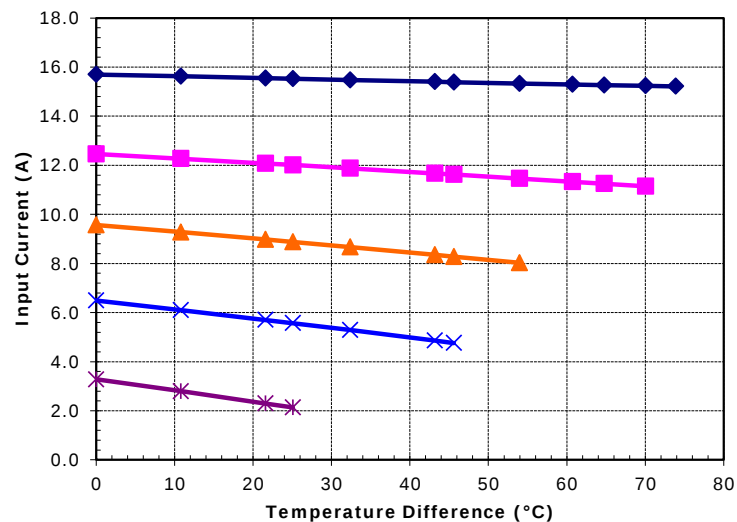
Unpotted TE-71-2.0-1.15 at a hot-side temperature of 50 °C
