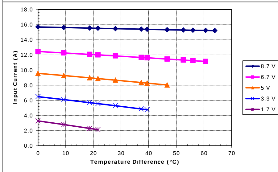
Potted TE-71-2.0-1.15 at a hot-side temperature of 30 °C
