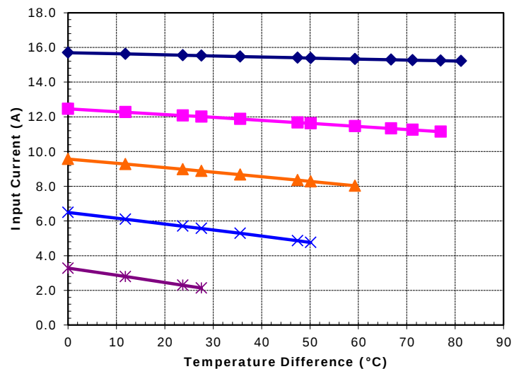
Unpotted TE-71-2.0-1.15 at a hot-side temperature of 70 °C
