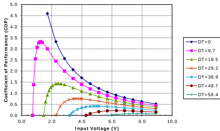
Potted TE-71-1.4-3.175 at a hot-side temperature of 30 °C
