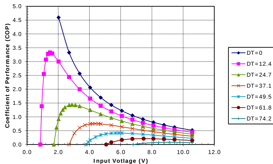
Unpotted TE-71-1.4-3.175 at a hot-side temperature of 70 °C
