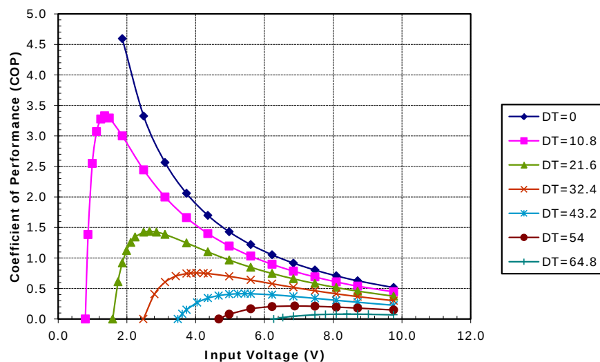
Potted TE-71-1.4-3.175 at a hot-side temperature of 50 °C
