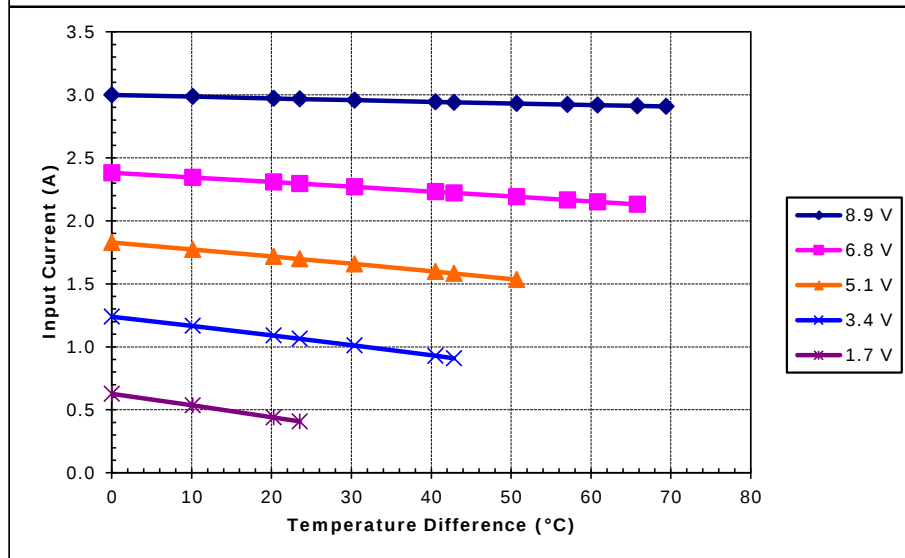
Unpotted TE-71-1.4-3.175 at a hot-side temperature of 30 °C
