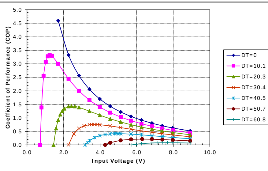
Unpotted TE-71-1.4-3.175 at a hot-side temperature of 30 °C
