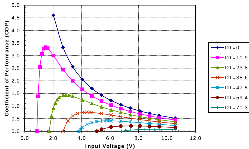
Potted TE-71-1.4-3.175 at a hot-side temperature of 70 °C
