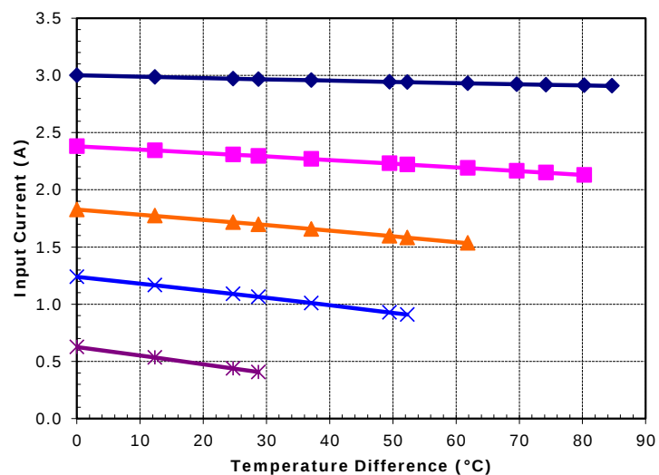
Unpotted TE-71-1.4-3.175 at a hot-side temperature of 70 °C
