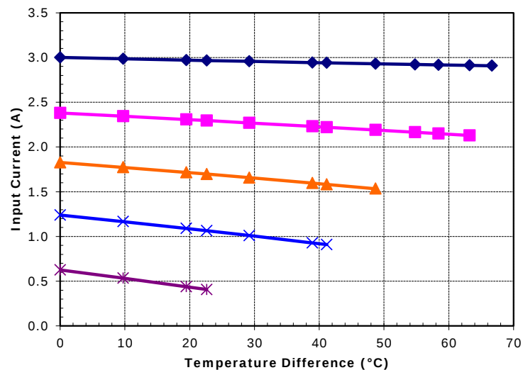
Potted TE-71-1.4-3.175 at a hot-side temperature of 30 °C
