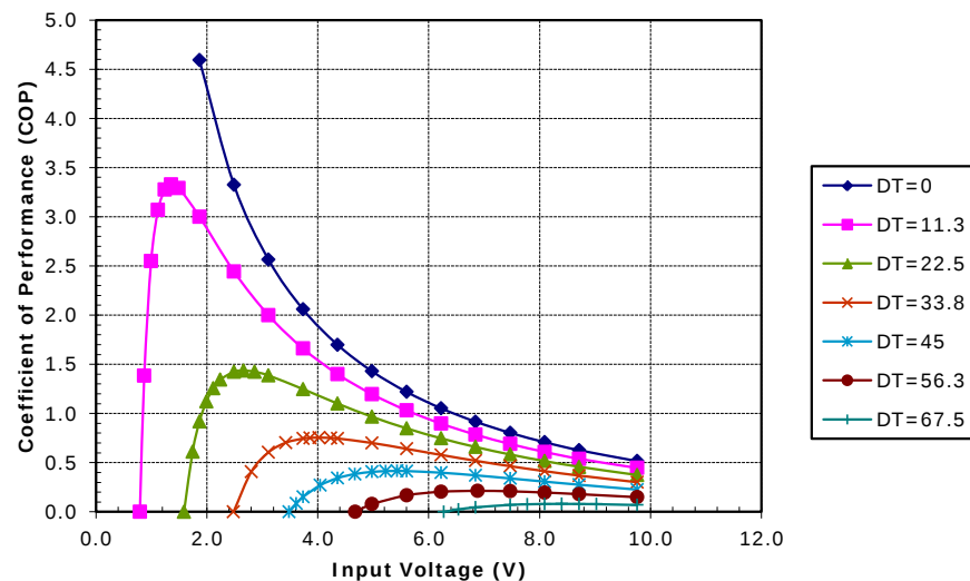
Unpotted TE-71-1.4-3.175 at a hot-side temperature of 50 °C
