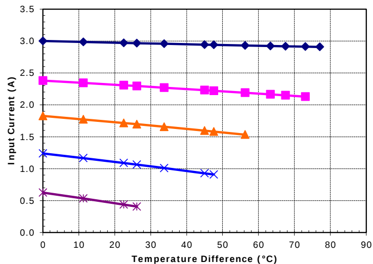
Unpotted TE-71-1.4-3.175 at a hot-side temperature of 50 °C
