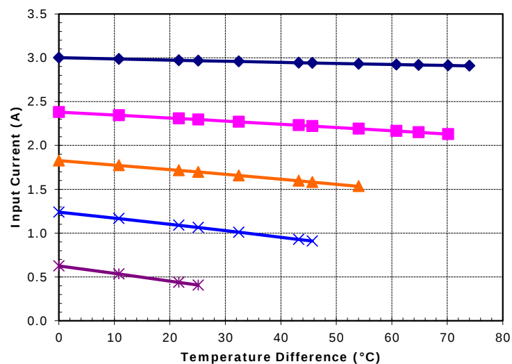
Potted TE-71-1.4-3.175 at a hot-side temperature of 50 °C
