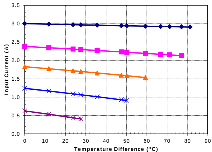
Potted TE-71-1.4-3.175 at a hot-side temperature of 70 °C
