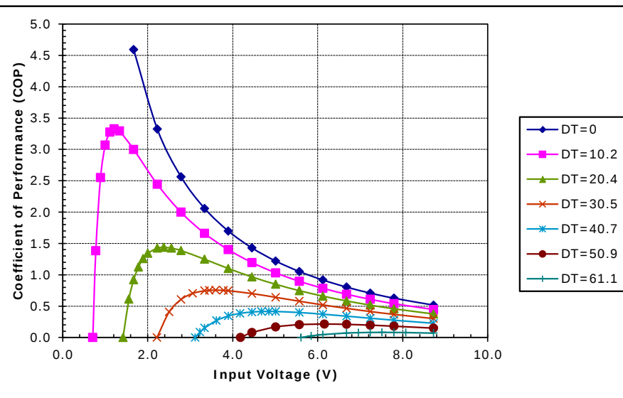
Unpotted TE-71-1.4-1.8 at a hot-side temperature of 30 °C
