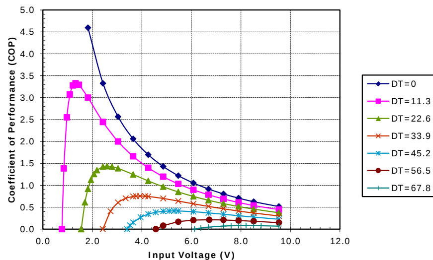
Unpotted TE-71-1.4-1.8 at a hot-side temperature of 50 °C
