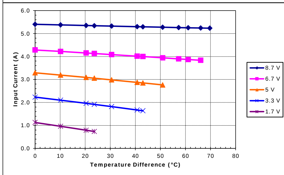
Unpotted TE-71-1.4-1.8 at a hot-side temperature of 30 °C
