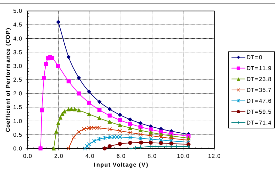
Potted TE-71-1.4-1.8 at a hot-side temperature of 70 °C
