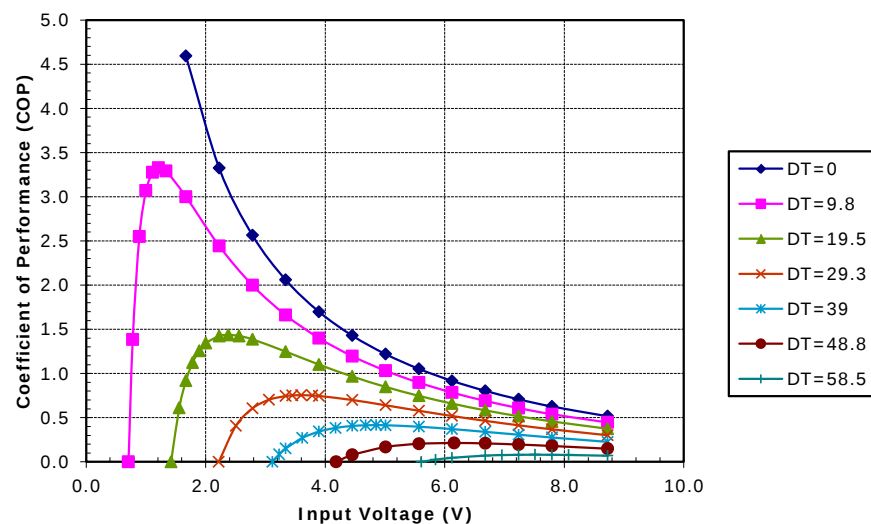
Potted TE-71-1.4-1.8 at a hot-side temperature of 30 °C
