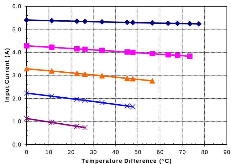
Unpotted TE-71-1.4-1.8 at a hot-side temperature of 50 °C
