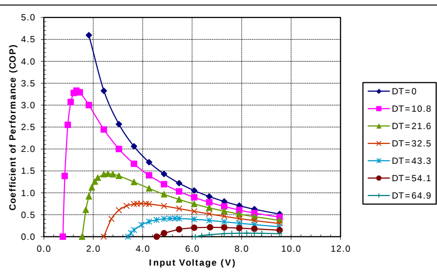
Potted TE-71-1.4-1.8 at a hot-side temperature of 50 °C
