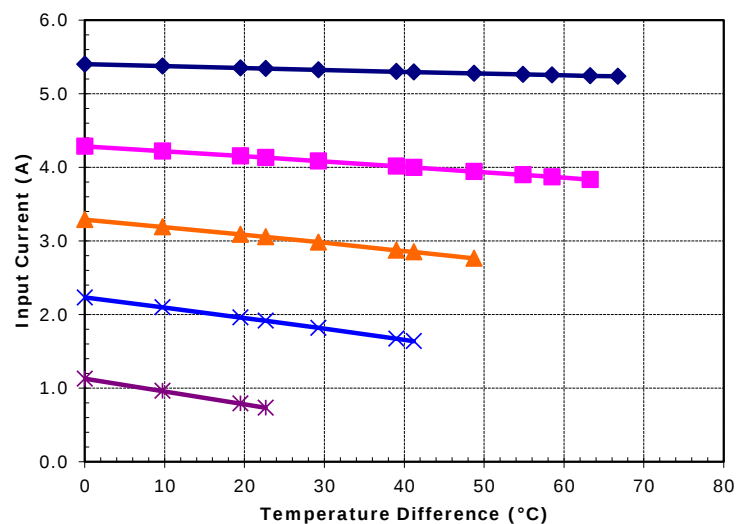
Potted TE-71-1.4-1.8 at a hot-side temperature of 30 °C
