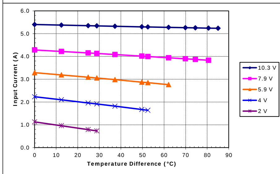
Unpotted TE-71-1.4-1.8 at a hot-side temperature of 70 °C
