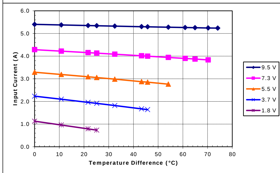
Potted TE-71-1.4-1.8 at a hot-side temperature of 50 °C
