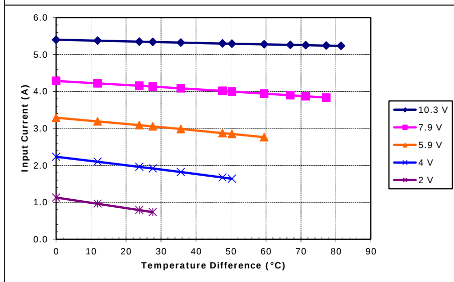
Potted TE-71-1.4-1.8 at a hot-side temperature of 70 °C
