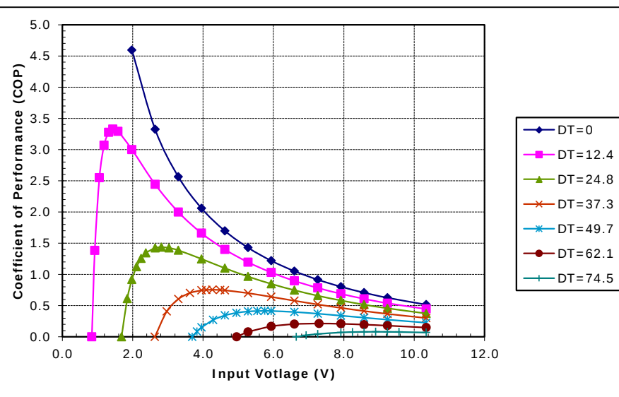
Unpotted TE-71-1.4-1.8 at a hot-side temperature of 70 °C
