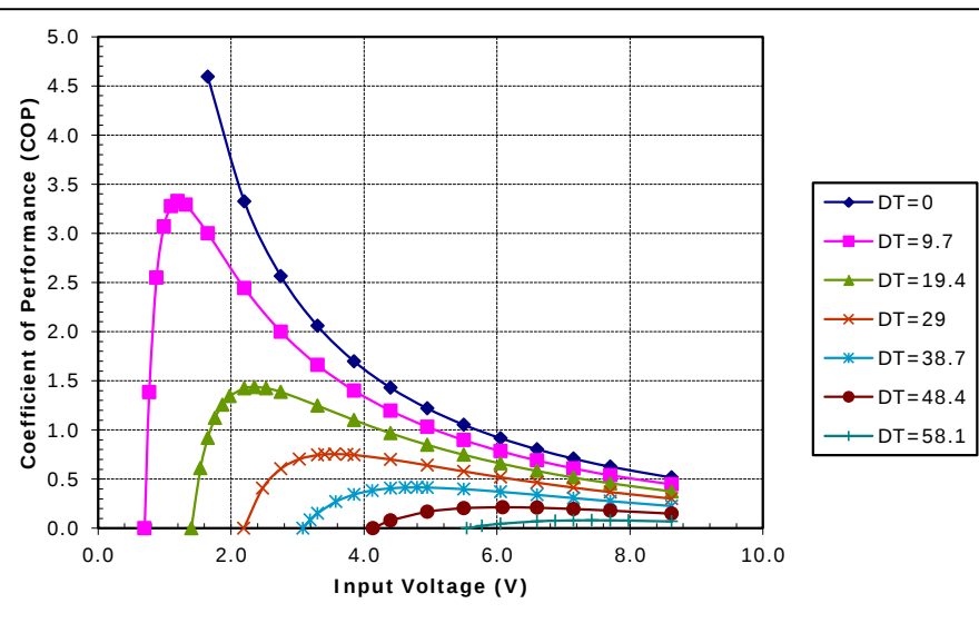
Potted TE-71-1.4-1.5 at a hot-side temperature of 30 °C
