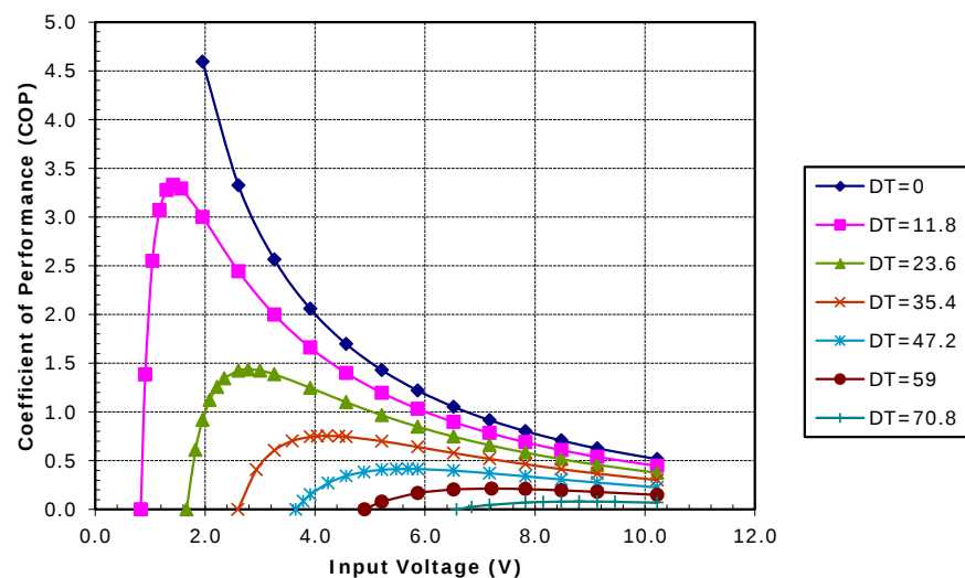
Potted TE-71-1.4-1.5 at a hot-side temperature of 70 °C
