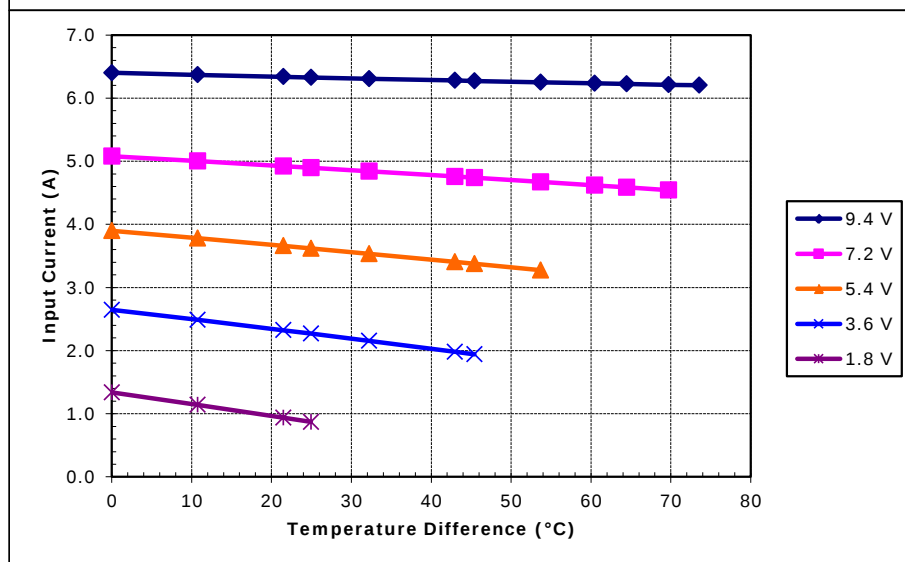
Potted TE-71-1.4-1.5 at a hot-side temperature of 50 °C
