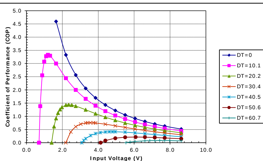
Unpotted TE-71-1.4-1.5 at a hot-side temperature of 30 °C
