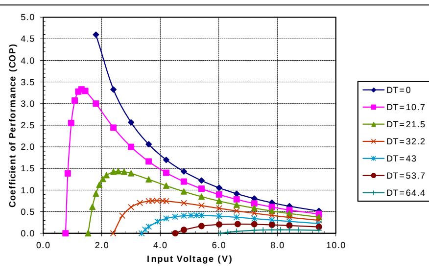
Potted TE-71-1.4-1.5 at a hot-side temperature of 50 °C
