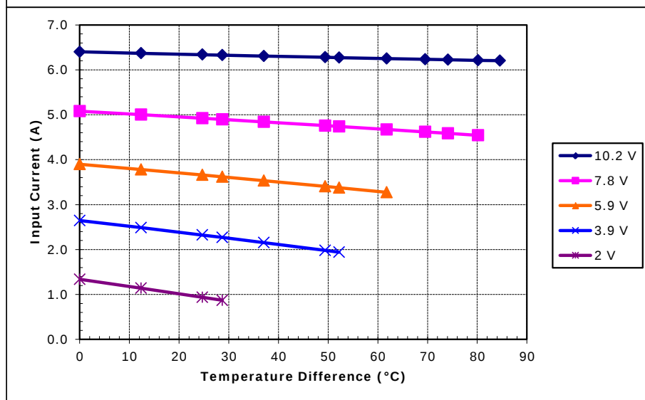
Unpotted TE-71-1.4-1.5 at a hot-side temperature of 70 °C
