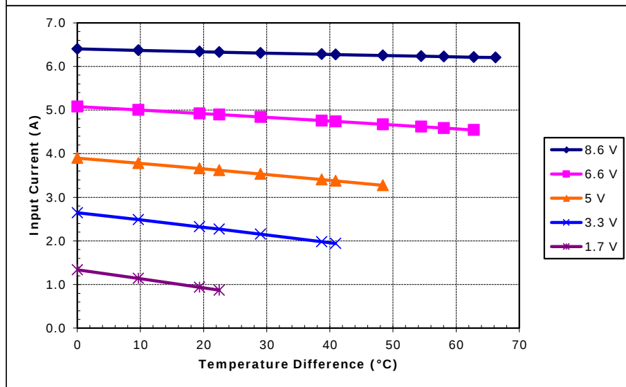
Potted TE-71-1.4-1.5 at a hot-side temperature of 30 °C
