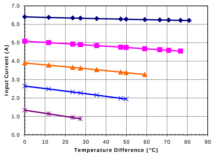
Potted TE-71-1.4-1.5 at a hot-side temperature of 70 °C
