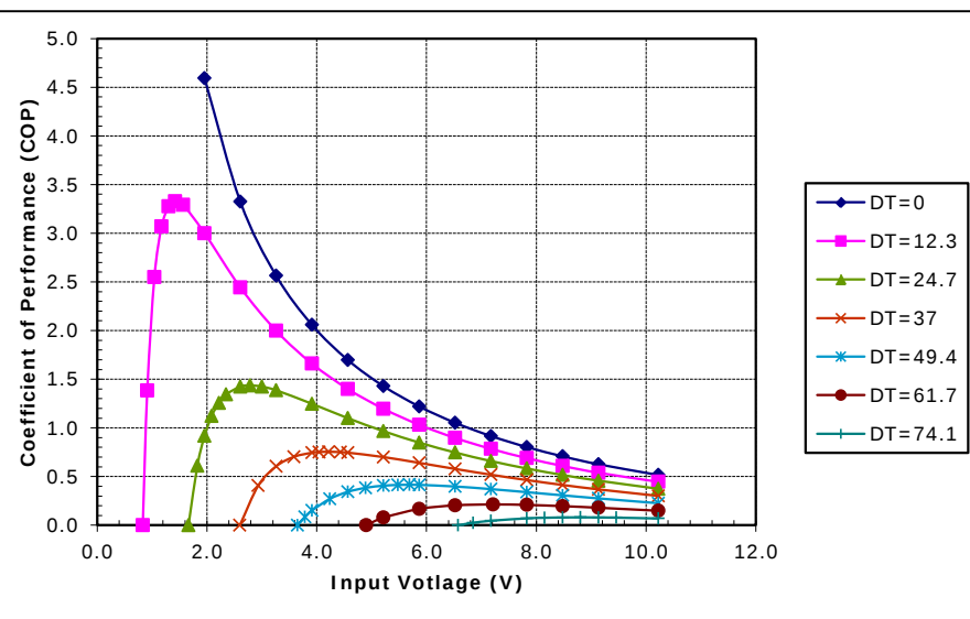
Unpotted TE-71-1.4-1.5 at a hot-side temperature of 70 °C
