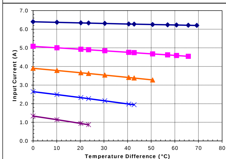
Unpotted TE-71-1.4-1.5 at a hot-side temperature of 30 °C
