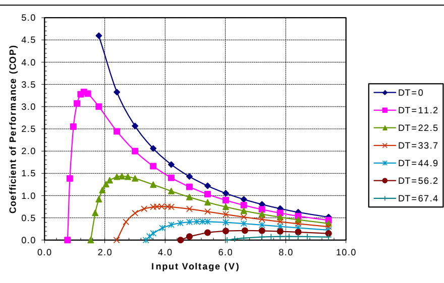
Unpotted TE-71-1.4-1.5 at a hot-side temperature of 50 °C
