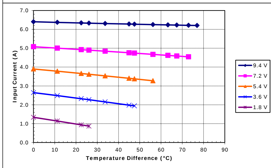
Unpotted TE-71-1.4-1.5 at a hot-side temperature of 50 °C
