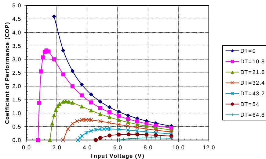
Potted TE-71-1.0-2.5 at a hot-side temperature of 50 °C
