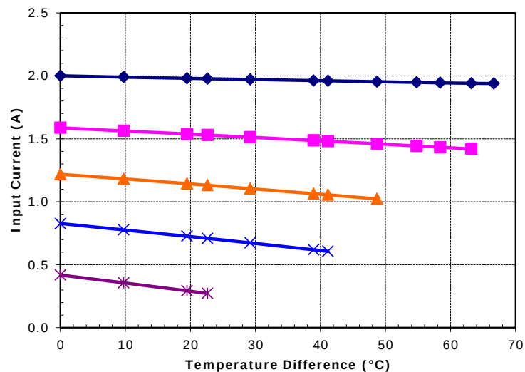
Potted TE-71-1.0-2.5 at a hot-side temperature of 30 °C
