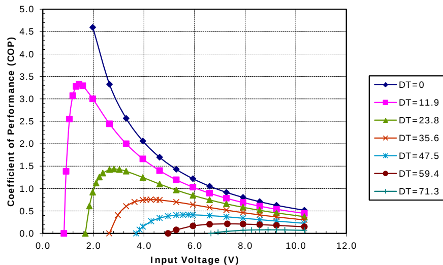
Potted TE-71-1.0-2.5 at a hot-side temperature of 70 °C
