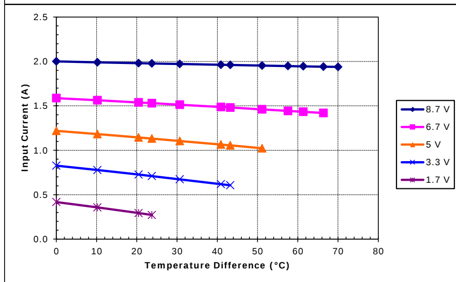
Unpotted TE-71-1.0-2.5 at a hot-side temperature of 30 °C
