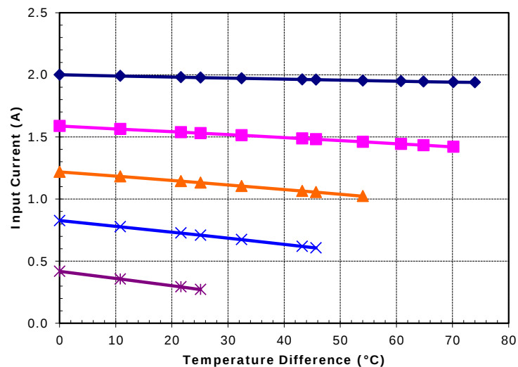
Potted TE-71-1.0-2.5 at a hot-side temperature of 50 °C
