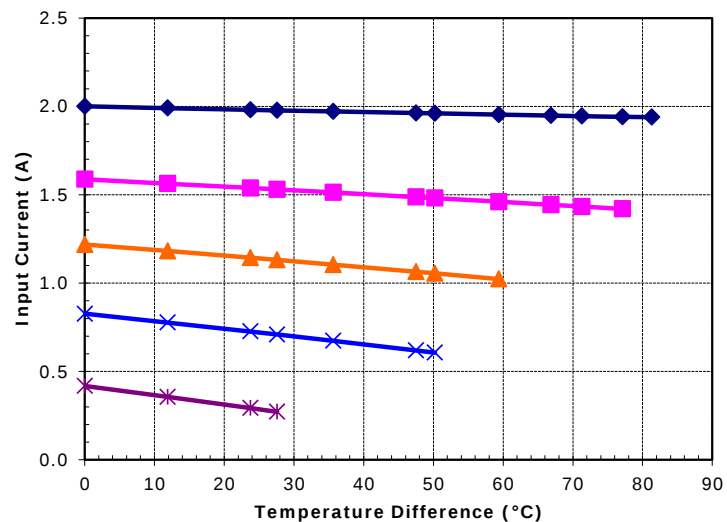
Potted TE-71-1.0-2.5 at a hot-side temperature of 70 °C
