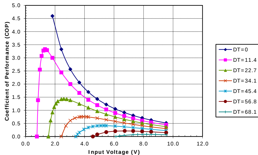
Unpotted TE-71-1.0-2.5 at a hot-side temperature of 50 °C
