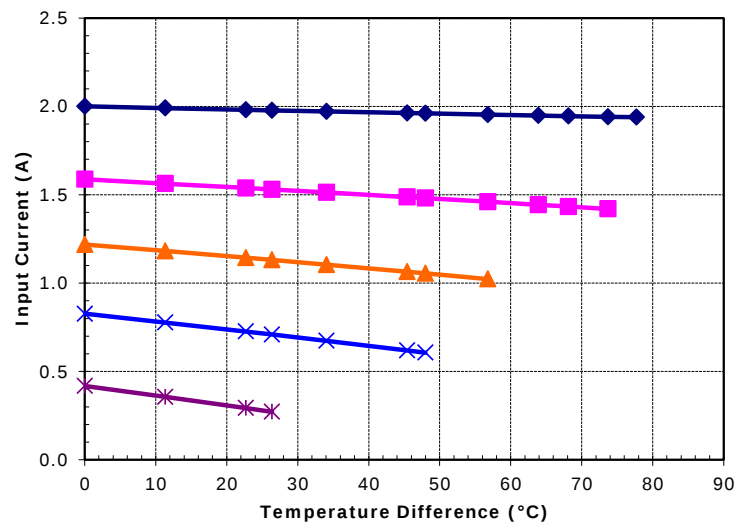
Unpotted TE-71-1.0-2.5 at a hot-side temperature of 50 °C
