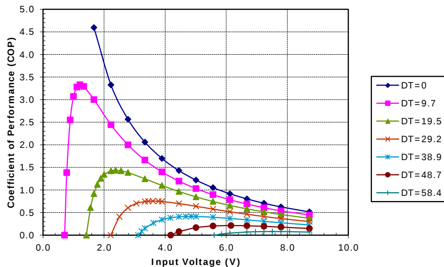
Potted TE-71-1.0-2.5 at a hot-side temperature of 30 °C
