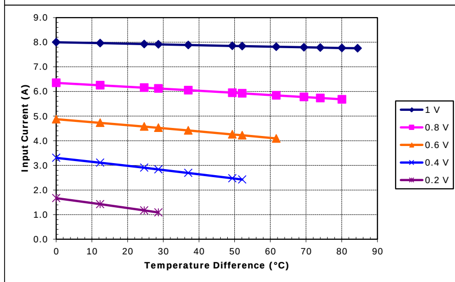
Unpotted TE-7-2.0-2.5 at a hot-side temperature of 70 °C
