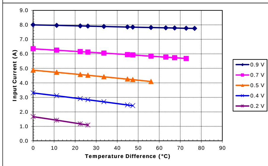
Unpotted TE-7-2.0-2.5 at a hot-side temperature of 50 °C
