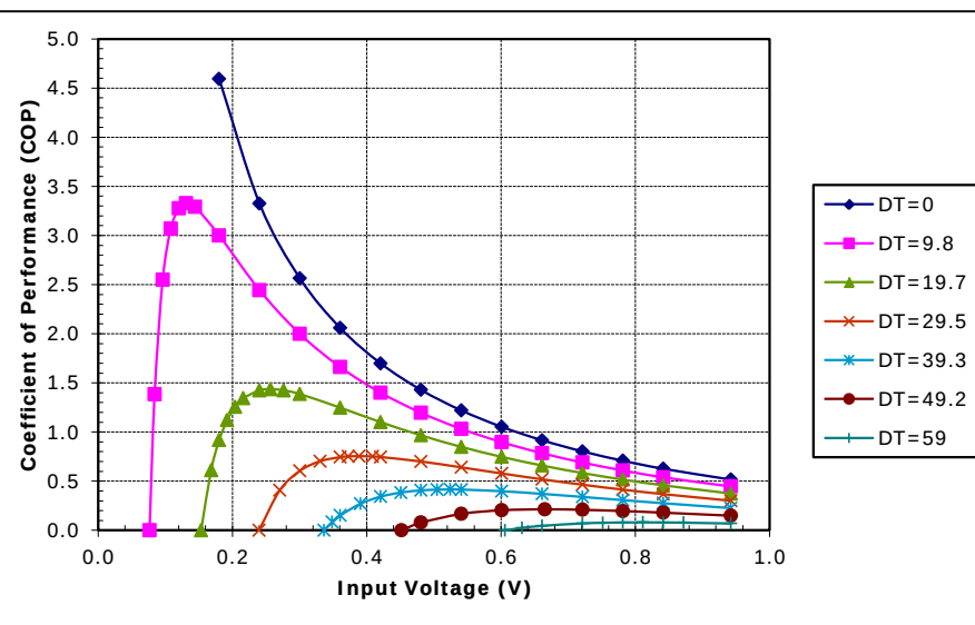
Potted TE-7-2.0-2.5 at a hot-side temperature of 50 °C
