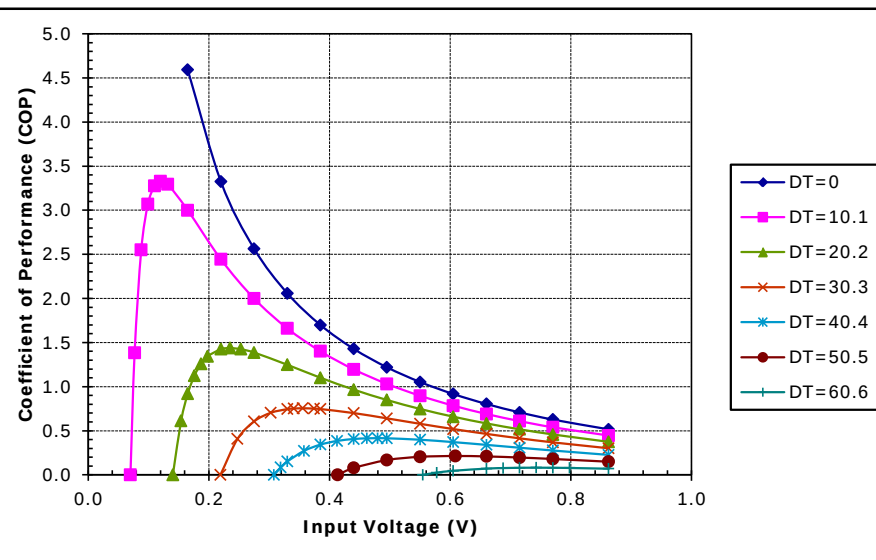
Unpotted TE-7-2.0-2.5 at a hot-side temperature of 30 °C
