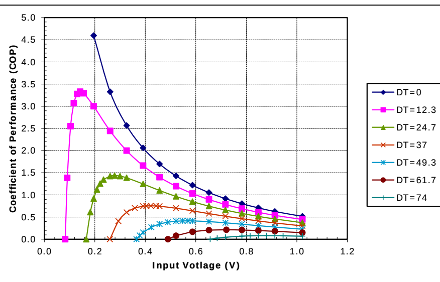
Unpotted TE-7-2.0-2.5 at a hot-side temperature of 70 °C
