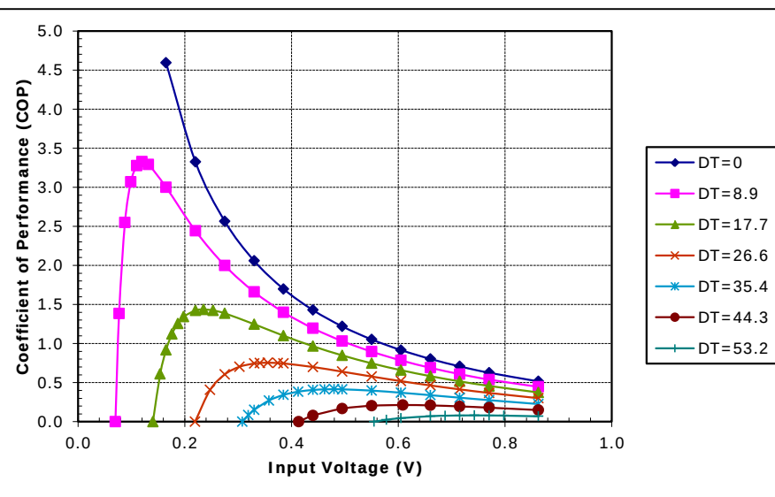
Potted TE-7-2.0-2.5 at a hot-side temperature of 30 °C
