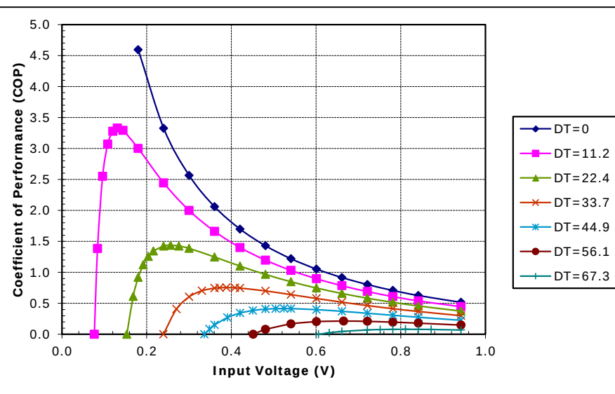
Unpotted TE-7-2.0-2.5 at a hot-side temperature of 50 °C
