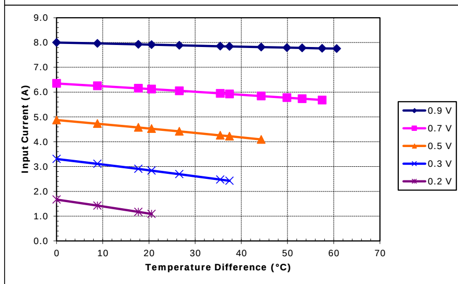
Potted TE-7-2.0-2.5 at a hot-side temperature of 30 °C
