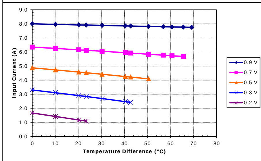
Unpotted TE-7-2.0-2.5 at a hot-side temperature of 30 °C
