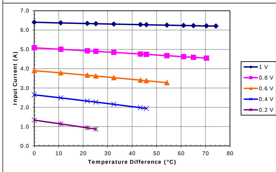
Potted TE-7-1.4-1.5 at a hot-side temperature of 70 °C
