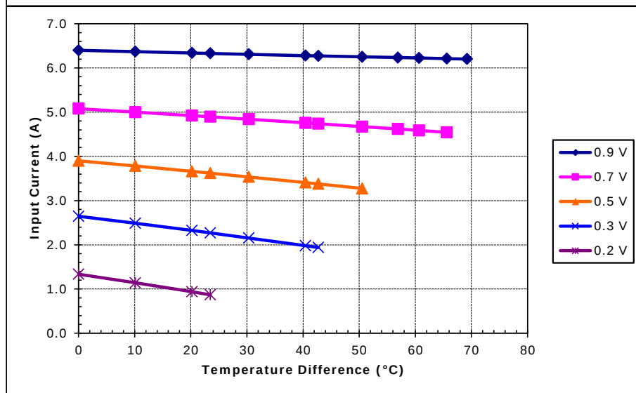
Unpotted TE-7-1.4-1.5 at a hot-side temperature of 30 °C
