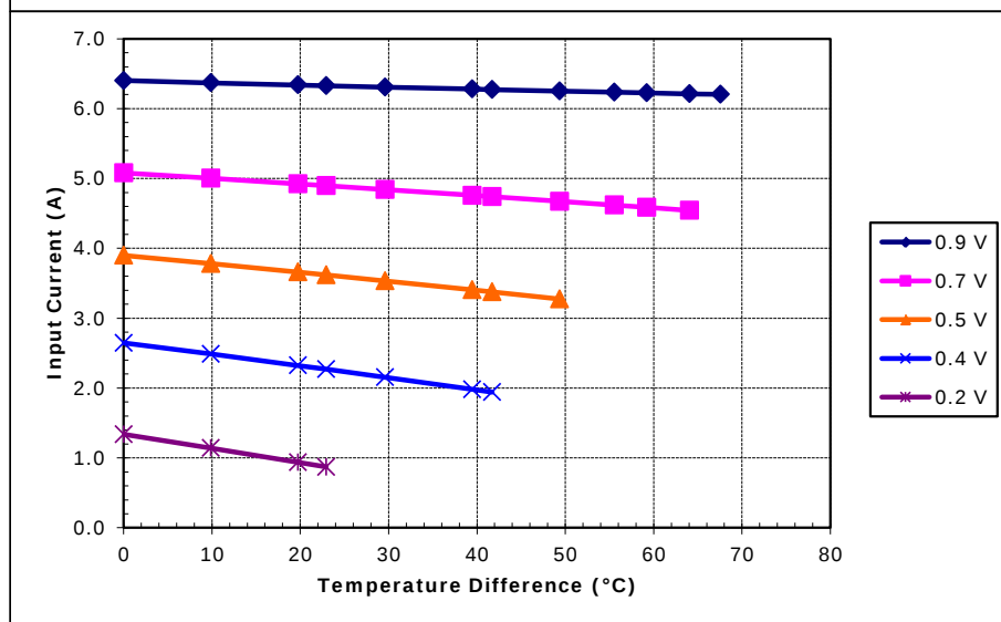
Potted TE-7-1.4-1.5 at a hot-side temperature of 50 °C
