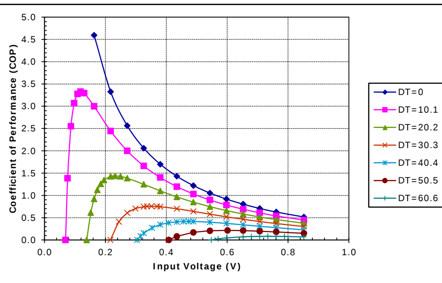
Unpotted TE-7-1.4-1.5 at a hot-side temperature of 30 °C
