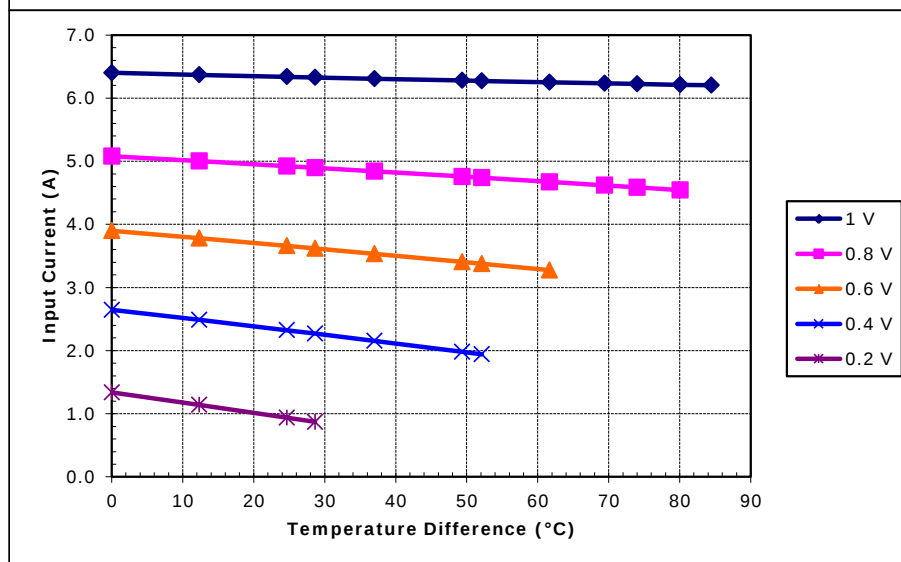
Unpotted TE-7-1.4-1.5 at a hot-side temperature of 70 °C
