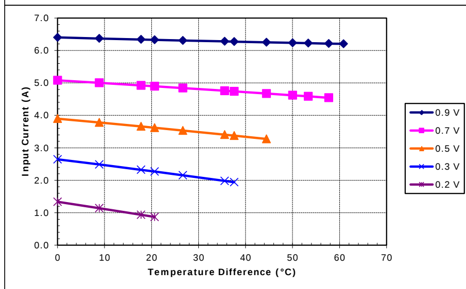
Potted TE-7-1.4-1.5 at a hot-side temperature of 30 °C
