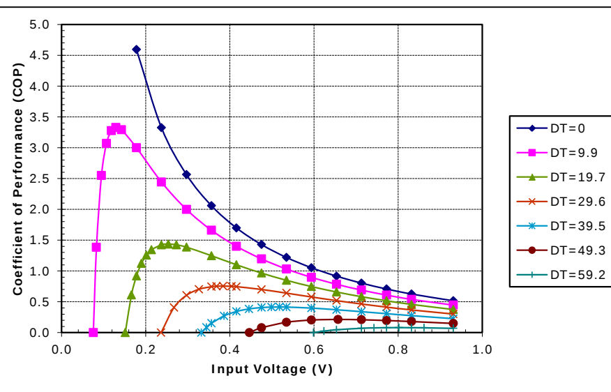
Potted TE-7-1.4-1.5 at a hot-side temperature of 50 °C
