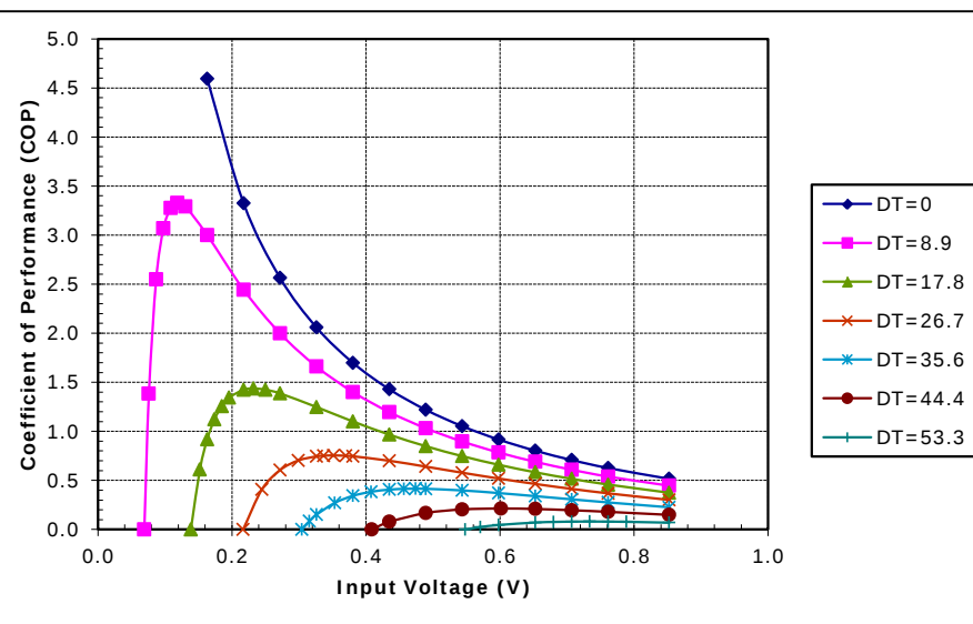
Potted TE-7-1.4-1.5 at a hot-side temperature of 30 °C
