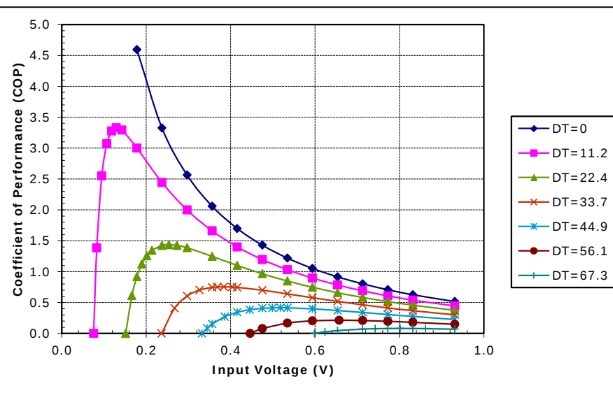
Unpotted TE-7-1.4-1.5 at a hot-side temperature of 50 °C
