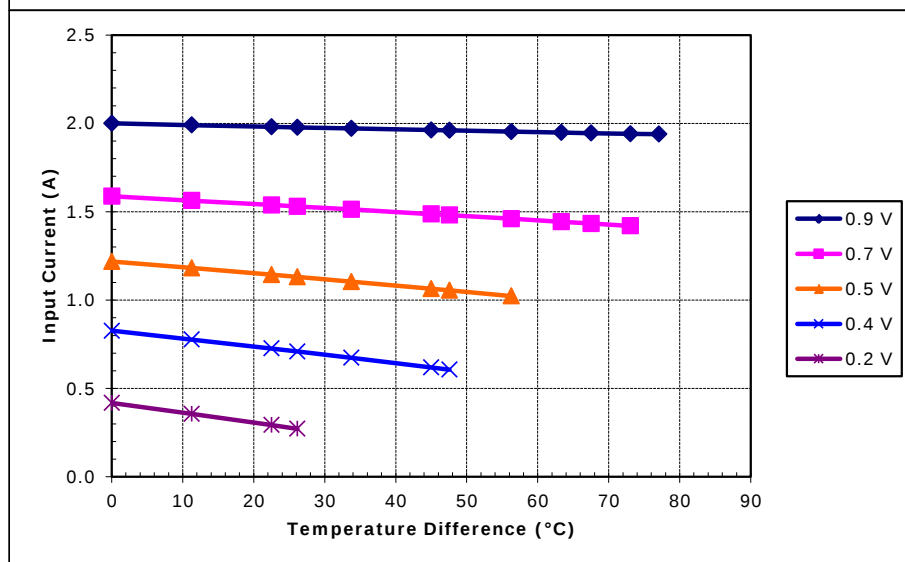
Unpotted TE-7-1.0-2.5 at a hot-side temperature of 50 °C
