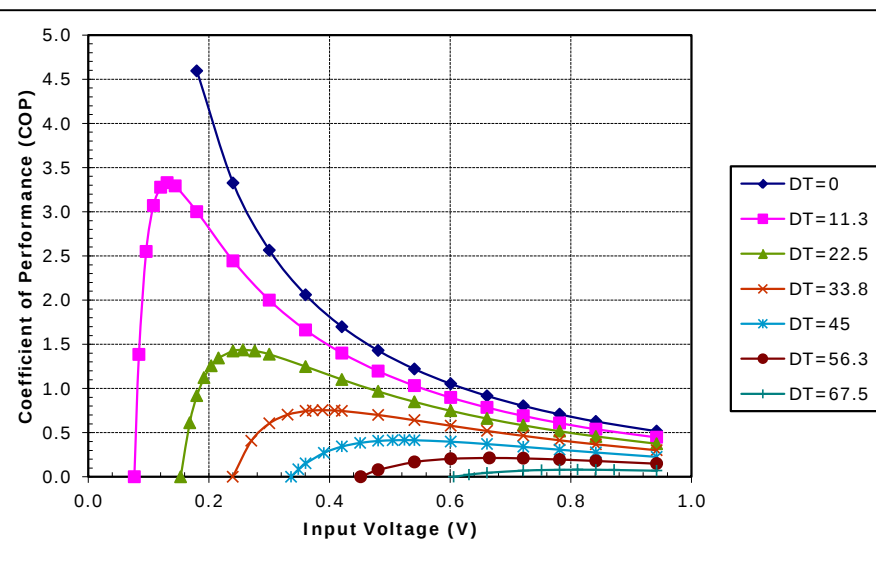
Unpotted TE-7-1.0-2.5 at a hot-side temperature of 50 °C
