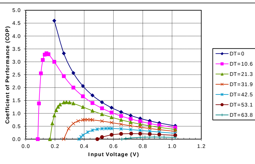
Potted TE-7-1.0-2.5 at a hot-side temperature of 70 °C
