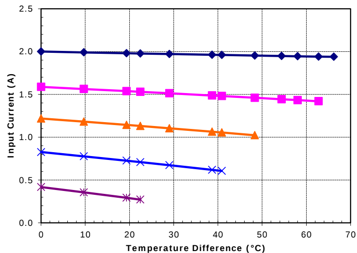
Potted TE-7-1.0-2.5 at a hot-side temperature of 50 °C
