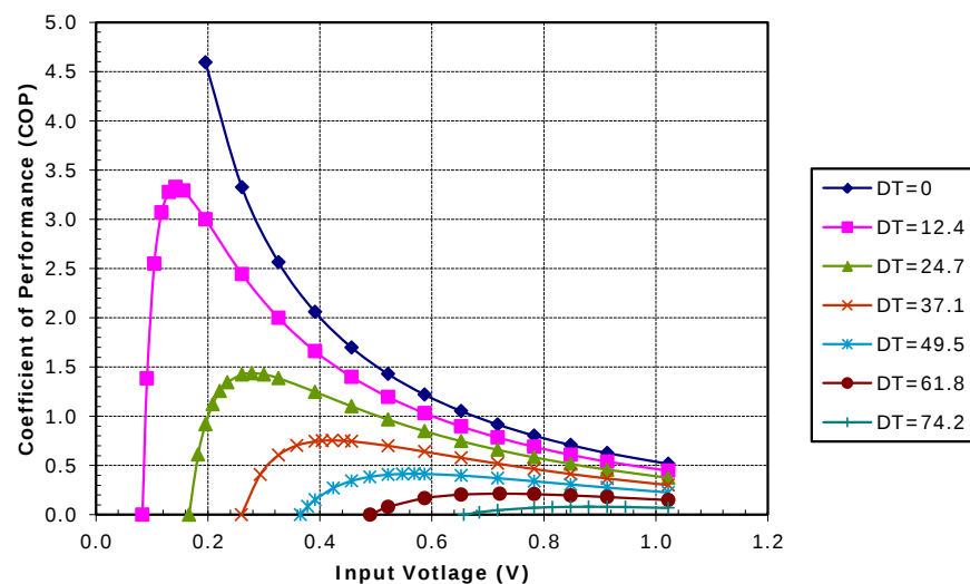
Unpotted TE-7-1.0-2.5 at a hot-side temperature of 70 °C
