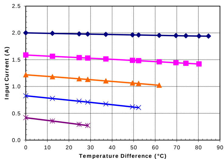
Unpotted TE-7-1.0-2.5 at a hot-side temperature of 70 °C
