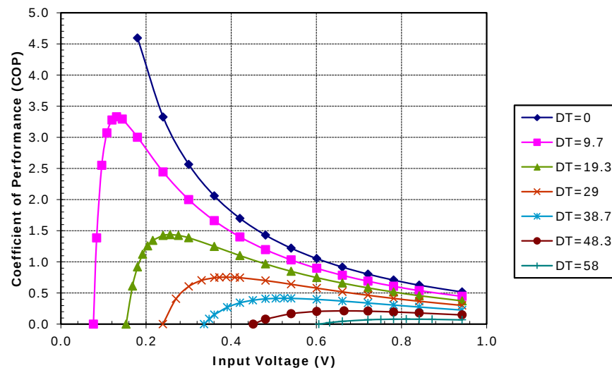
Potted TE-7-1.0-2.5 at a hot-side temperature of 50 °C
