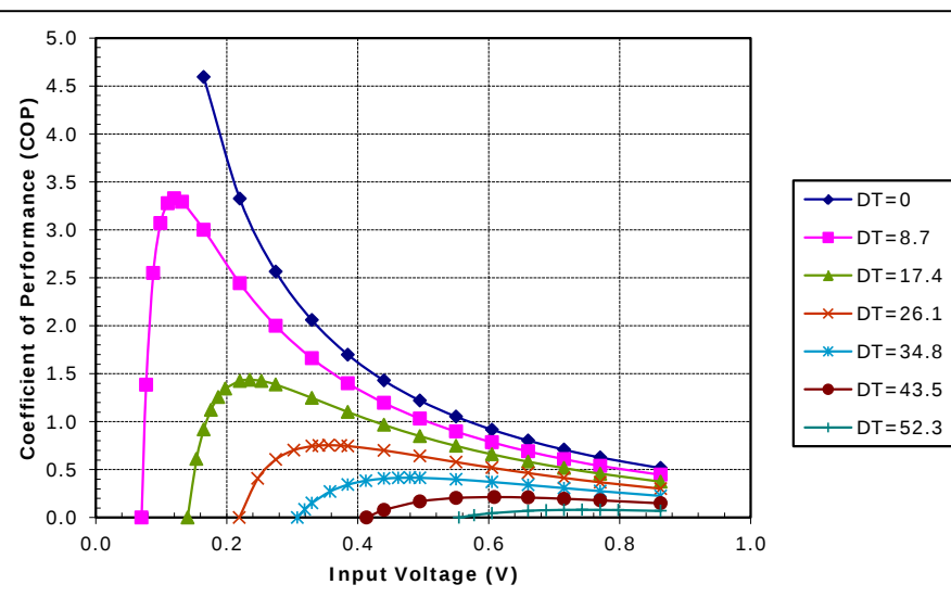
Potted TE-7-1.0-2.5 at a hot-side temperature of 30 °C
