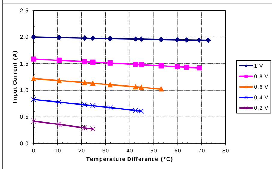
Potted TE-7-1.0-2.5 at a hot-side temperature of 70 °C
