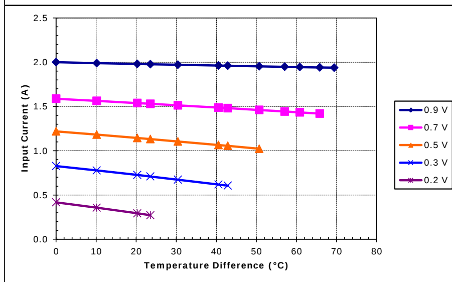
Unpotted TE-7-1.0-2.5 at a hot-side temperature of 30 °C
