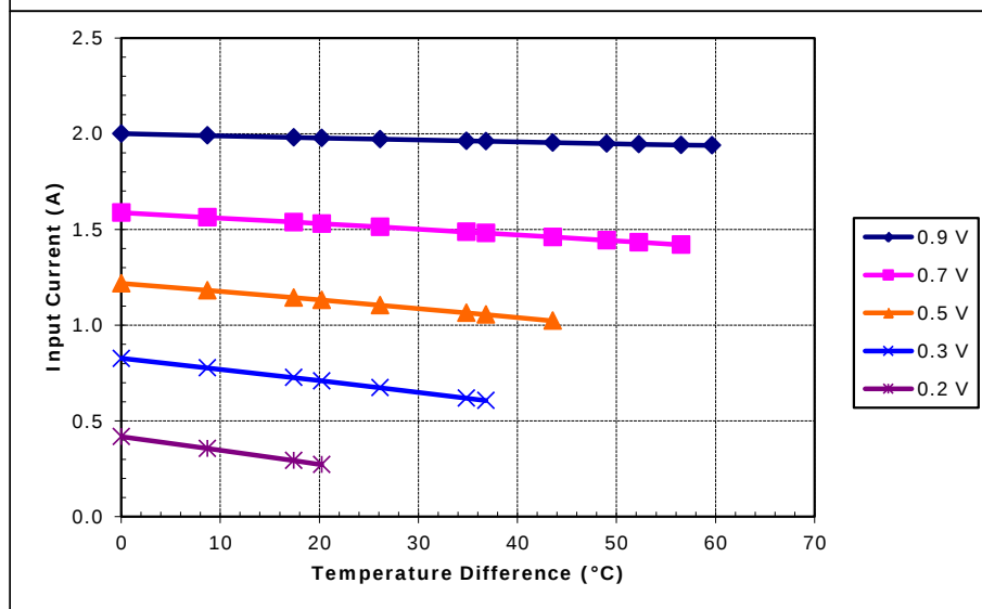
Potted TE-7-1.0-2.5 at a hot-side temperature of 30 °C
