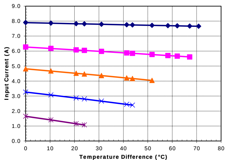
Potted TE-63-1.4-1.15 at a hot-side temperature of 50 °C
