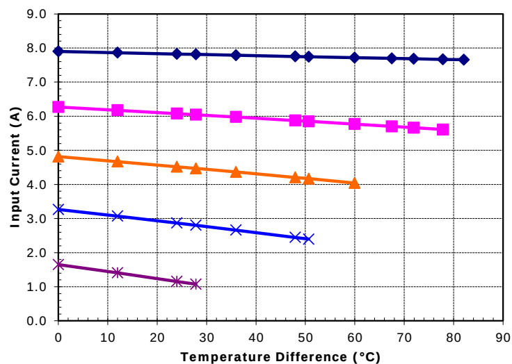
Unpotted TE-63-1.4-1.15 at a hot-side temperature of 70 °C
