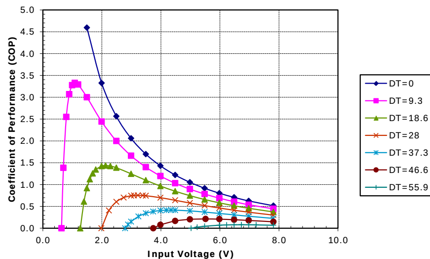
Potted TE-63-1.4-1.15 at a hot-side temperature of 30 °C
