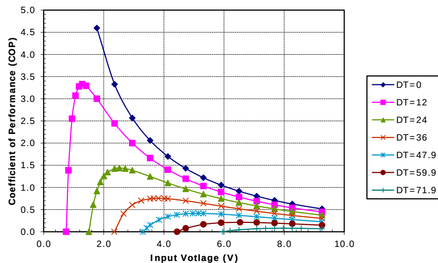
Unpotted TE-63-1.4-1.15 at a hot-side temperature of 70 °C
