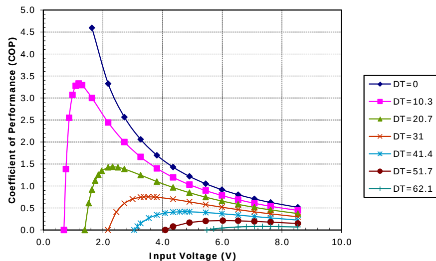
Potted TE-63-1.4-1.15 at a hot-side temperature of 50 °C
