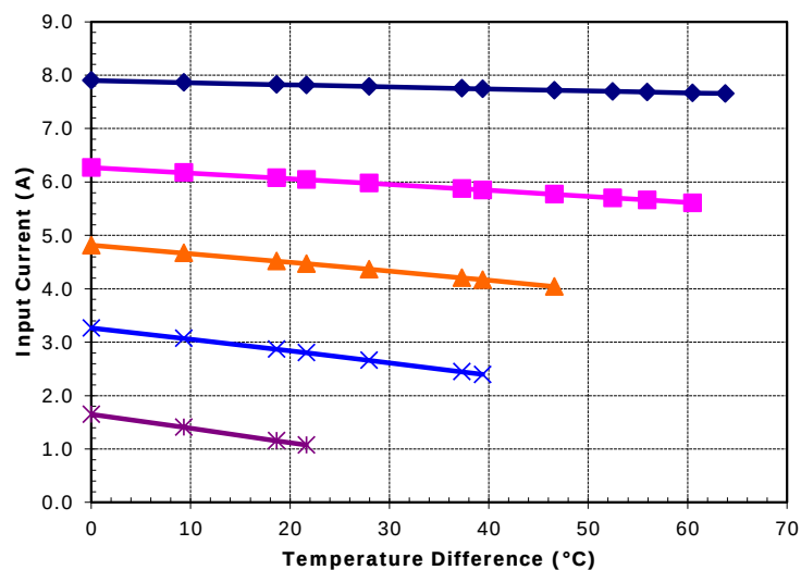
Potted TE-63-1.4-1.15 at a hot-side temperature of 30 °C
