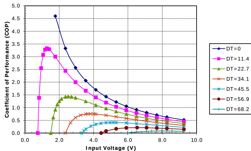
Potted TE-63-1.4-1.15 at a hot-side temperature of 70 °C
