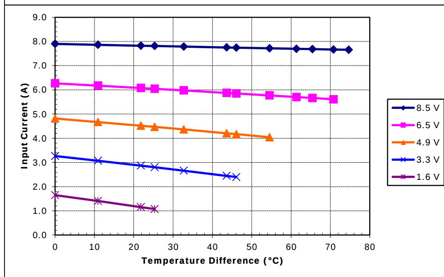
Unpotted TE-63-1.4-1.15 at a hot-side temperature of 50 °C
