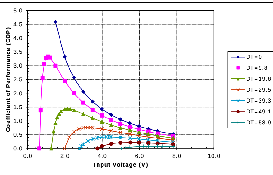
Unpotted TE-63-1.4-1.15 at a hot-side temperature of 30 °C
