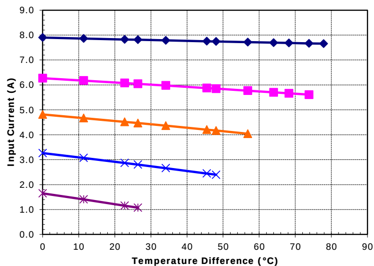
Potted TE-63-1.4-1.15 at a hot-side temperature of 70 °C
