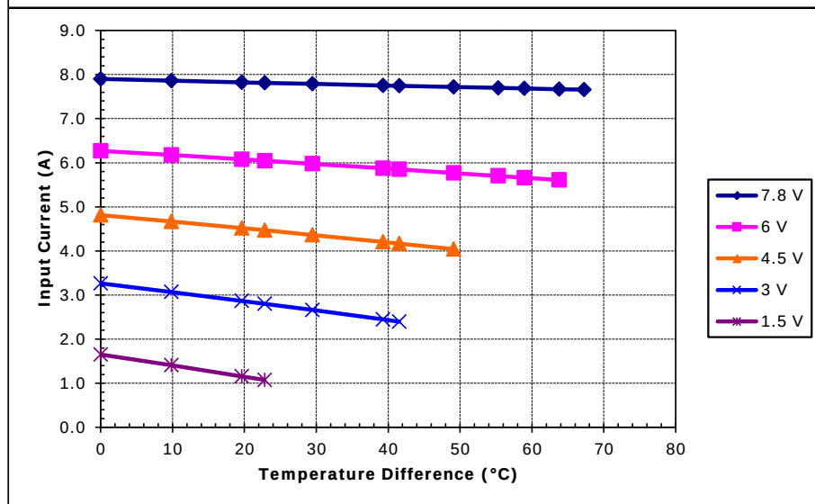
Unpotted TE-63-1.4-1.15 at a hot-side temperature of 30 °C
