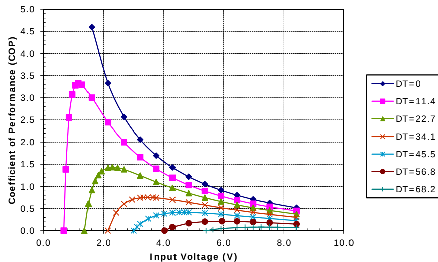
Unpotted TE-63-1.0-2.5 at a hot-side temperature of 50 °C
