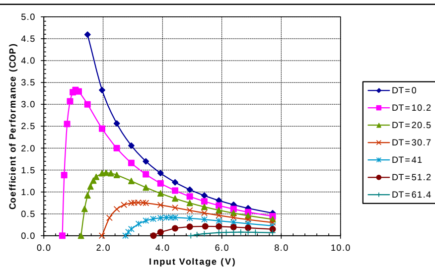
Unpotted TE-63-1.0-2.5 at a hot-side temperature of 30 °C
