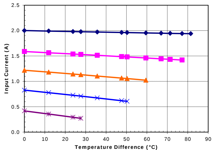
Potted TE-63-1.0-2.5 at a hot-side temperature of 70 °C
