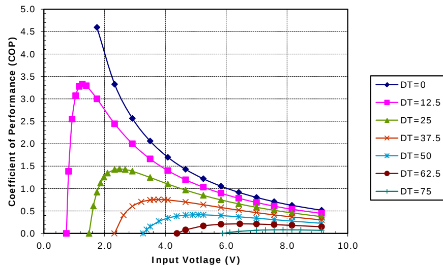
Unpotted TE-63-1.0-2.5 at a hot-side temperature of 70 °C
