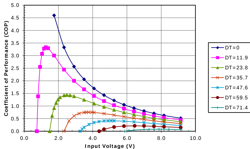
Potted TE-63-1.0-2.5 at a hot-side temperature of 70 °C
