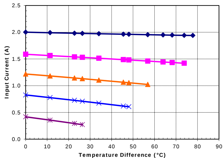
Unpotted TE-63-1.0-2.5 at a hot-side temperature of 50 °C
