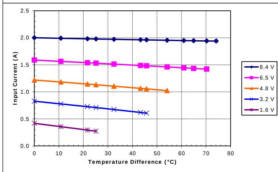
Potted TE-63-1.0-2.5 at a hot-side temperature of 50 °C
