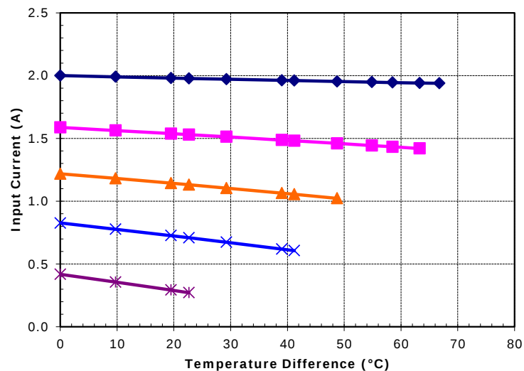
Potted TE-63-1.0-2.5 at a hot-side temperature of 30 °C
