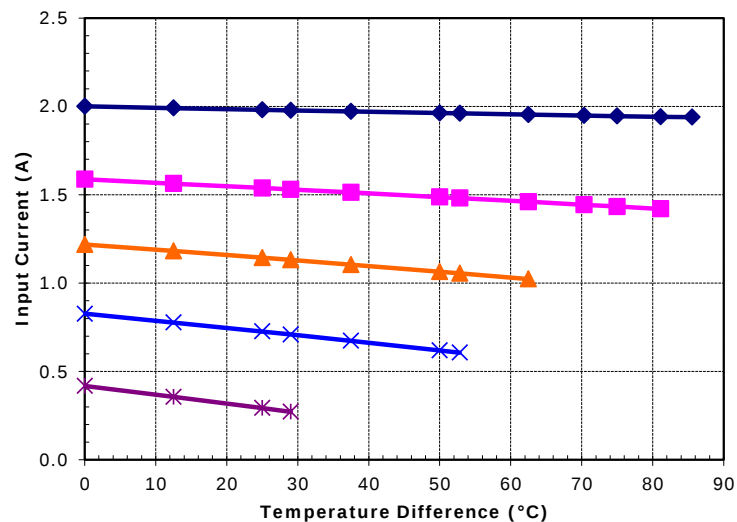
Unpotted TE-63-1.0-2.5 at a hot-side temperature of 70 °C
