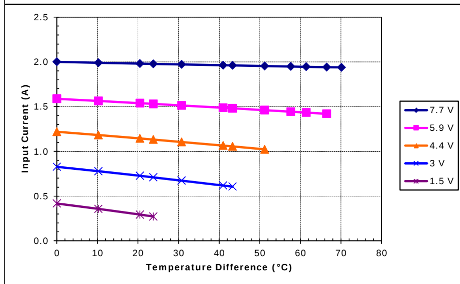
Unpotted TE-63-1.0-2.5 at a hot-side temperature of 30 °C
