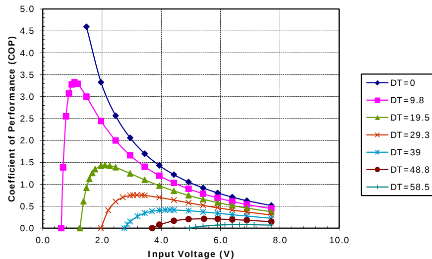
Potted TE-63-1.0-2.5 at a hot-side temperature of 30 °C
