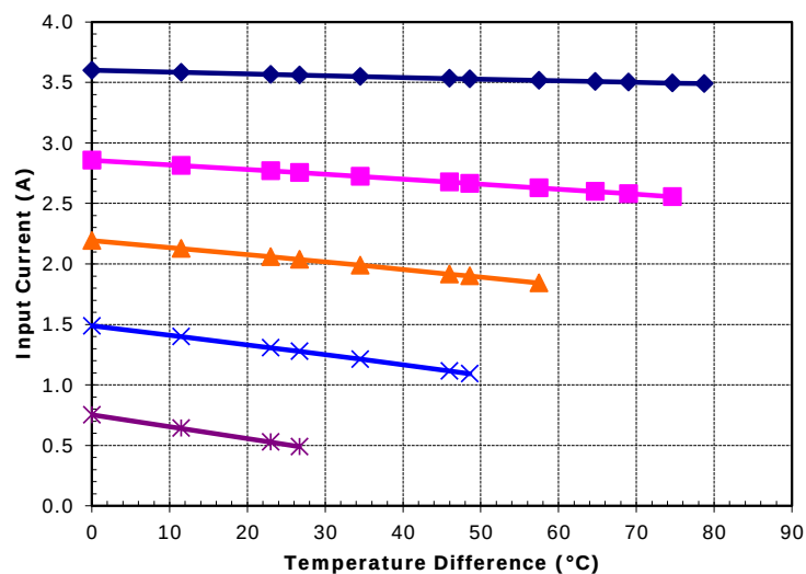
Potted TE-63-1.0-1.3 at a hot-side temperature of 70 °C
