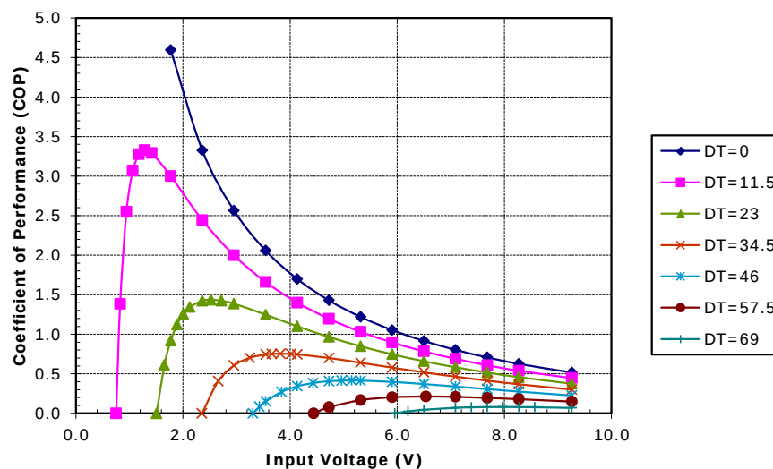
Potted TE-63-1.0-1.3 at a hot-side temperature of 70 °C
