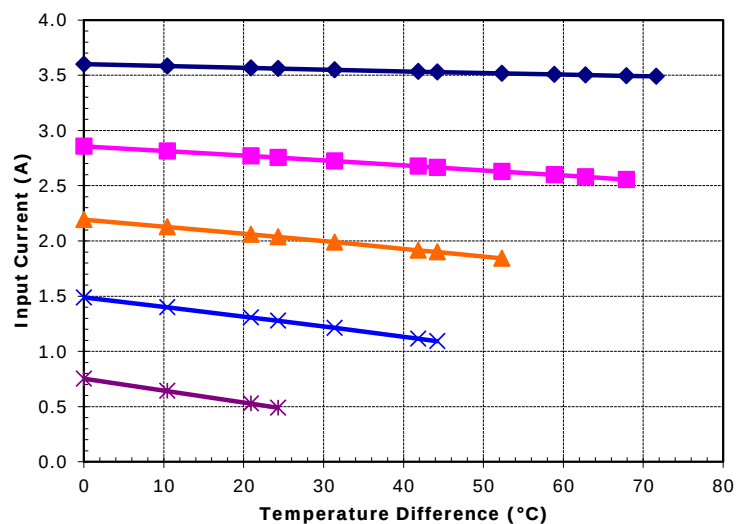
Potted TE-63-1.0-1.3 at a hot-side temperature of 50 °C
