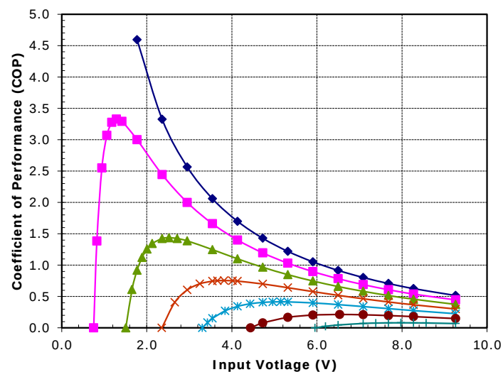
Unpotted TE-63-1.0-1.3 at a hot-side temperature of 70 °C
