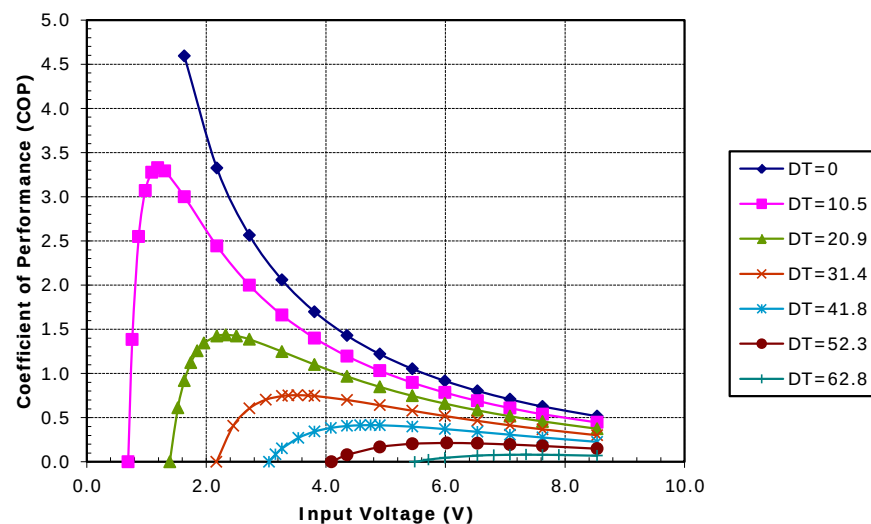
Potted TE-63-1.0-1.3 at a hot-side temperature of 50 °C
