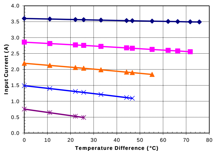
Unpotted TE-63-1.0-1.3 at a hot-side temperature of 50 °C
