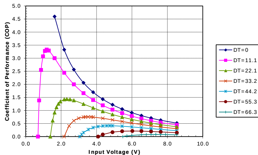
Unpotted TE-63-1.0-1.3 at a hot-side temperature of 50 °C
