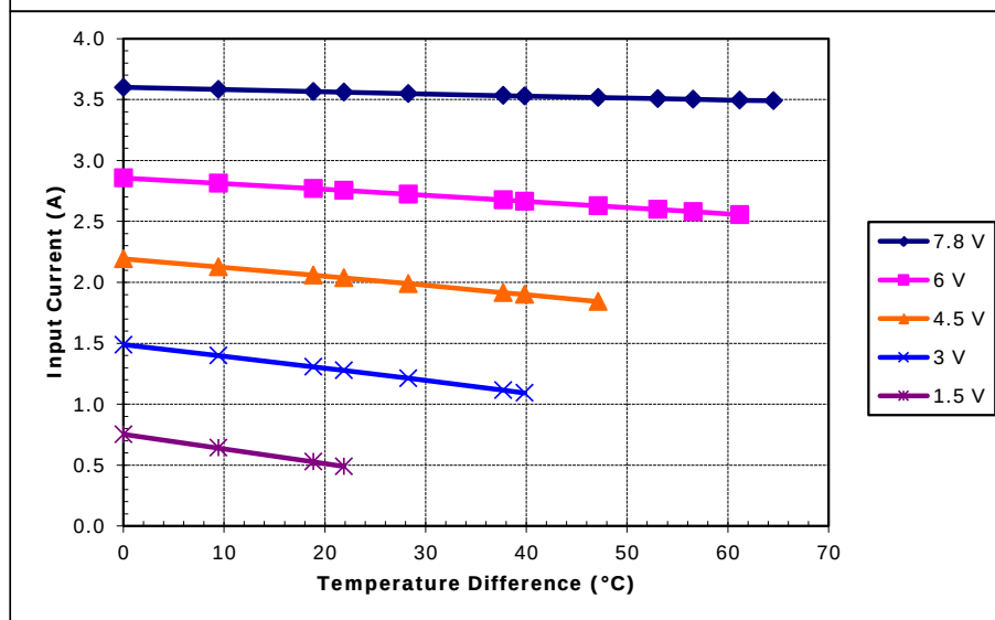
Potted TE-63-1.0-1.3 at a hot-side temperature of 30 °C
