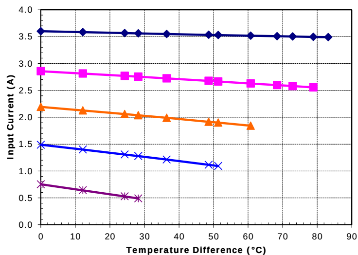
Unpotted TE-63-1.0-1.3 at a hot-side temperature of 70 °C
