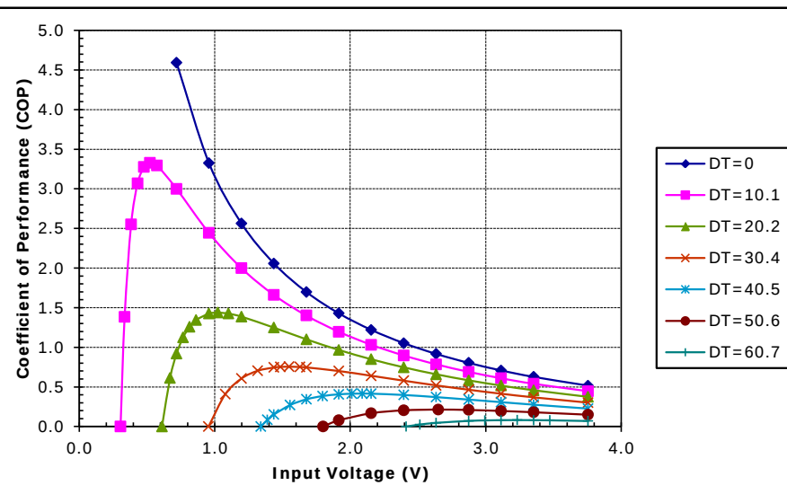
Unpotted TE-31-2.0-2.5 at a hot-side temperature of 30 °C
