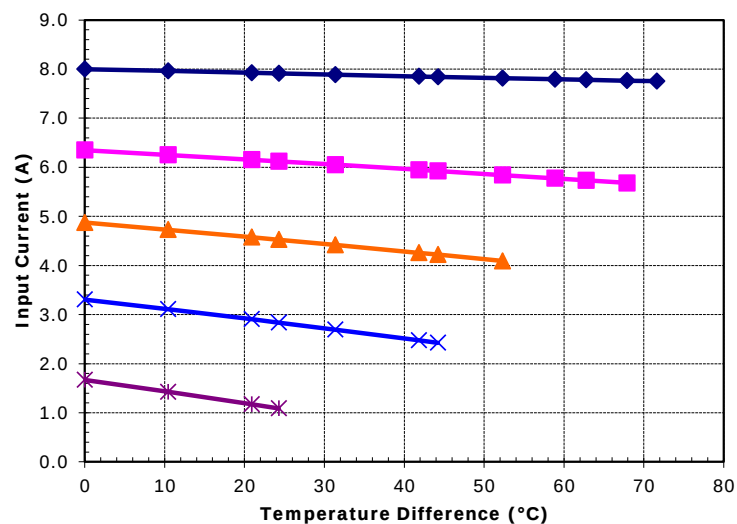
Potted TE-31-2.0-2.5 at a hot-side temperature of 50 °C
