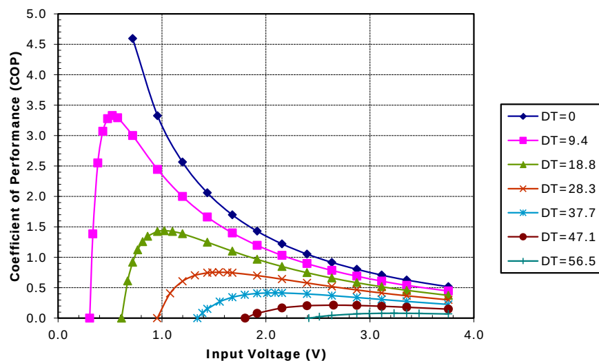
Potted TE-31-2.0-2.5 at a hot-side temperature of 30 °C
