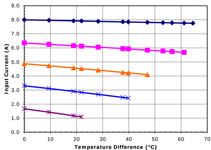
Potted TE-31-2.0-2.5 at a hot-side temperature of 30 °C
