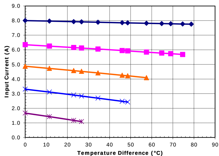
Potted TE-31-2.0-2.5 at a hot-side temperature of 70 °C
