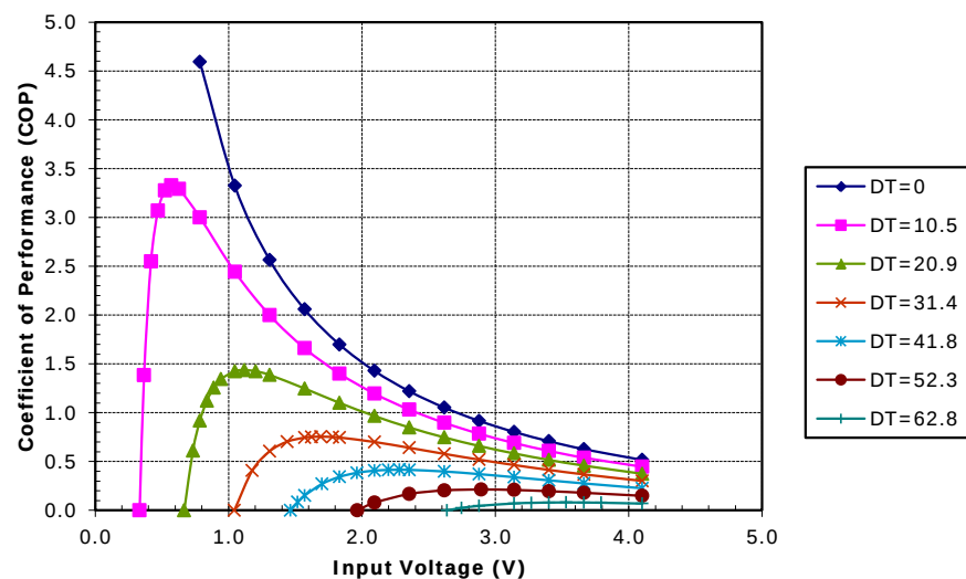
Potted TE-31-2.0-2.5 at a hot-side temperature of 50 °C
