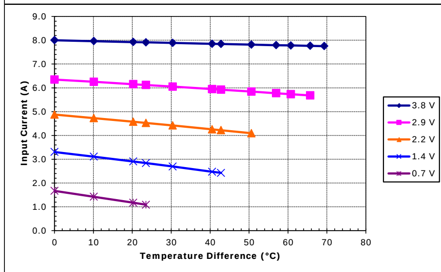
Unpotted TE-31-2.0-2.5 at a hot-side temperature of 30 °C
