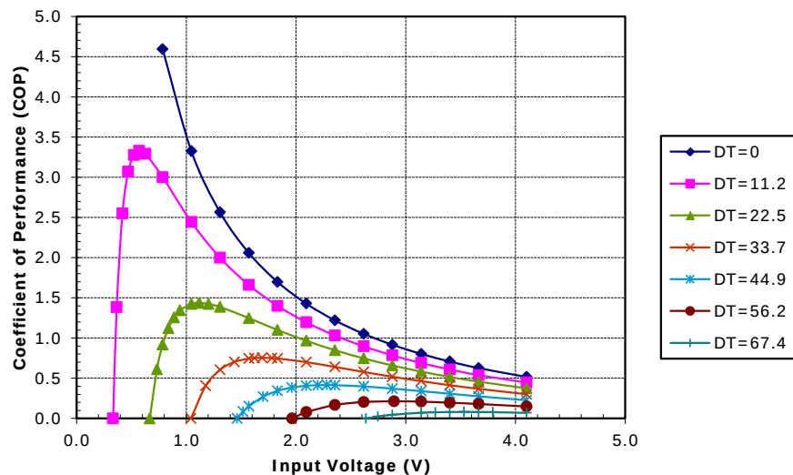
Unpotted TE-31-2.0-2.5 at a hot-side temperature of 50 °C
