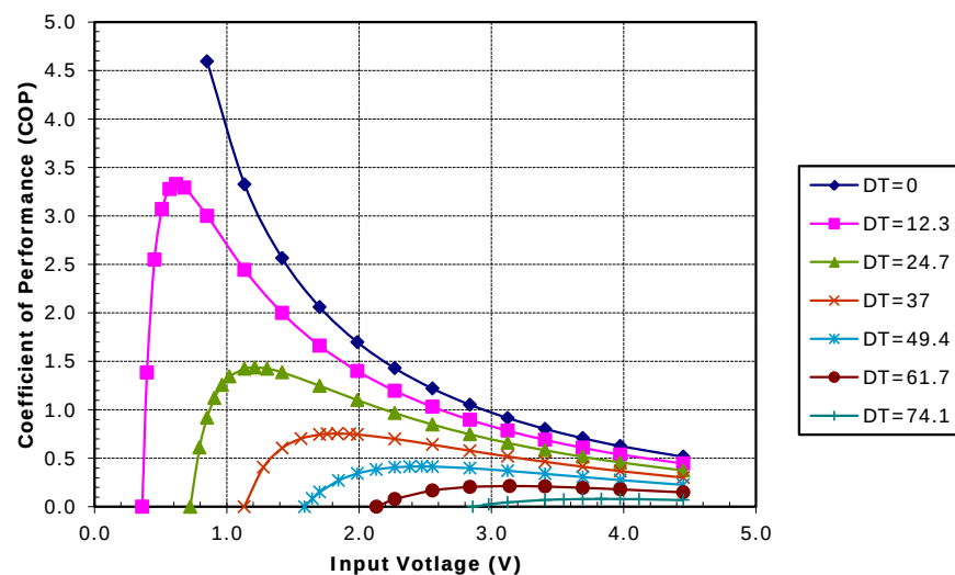
Unpotted TE-31-2.0-2.5 at a hot-side temperature of 70 °C
