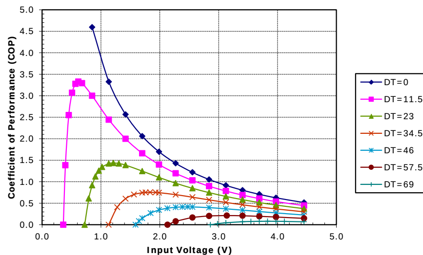
Potted TE-31-2.0-2.5 at a hot-side temperature of 70 °C
