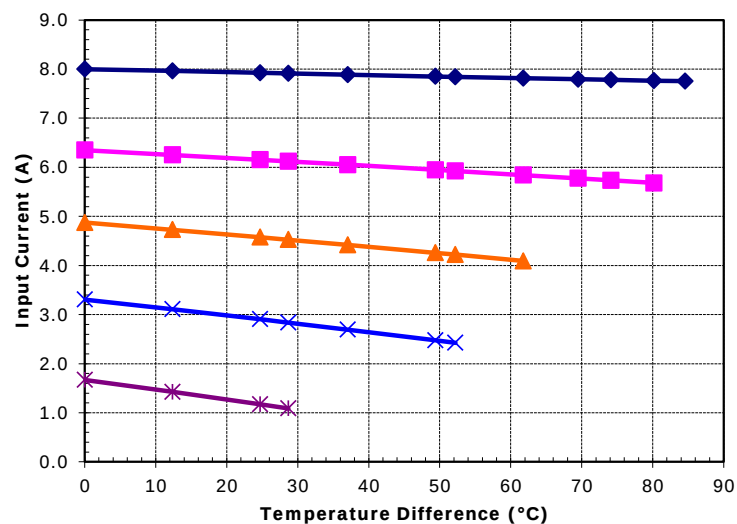
Unpotted TE-31-2.0-2.5 at a hot-side temperature of 70 °C
