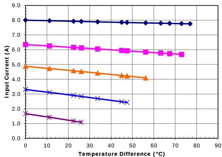
Unpotted TE-31-2.0-2.5 at a hot-side temperature of 50 °C
