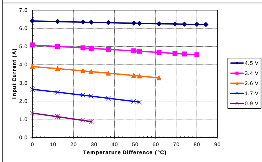
Unpotted TE-31-1.4-1.5 at a hot-side temperature of 70 °C
