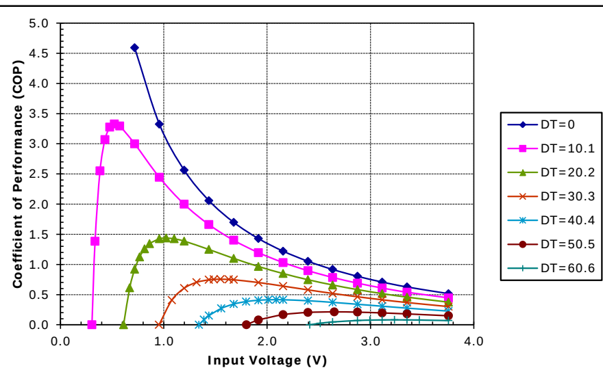
Unpotted TE-31-1.4-1.5 at a hot-side temperature of 30 °C
