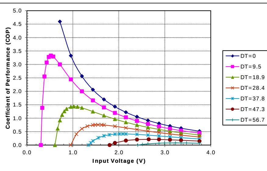
Potted TE-31-1.4-1.5 at a hot-side temperature of 30 °C
