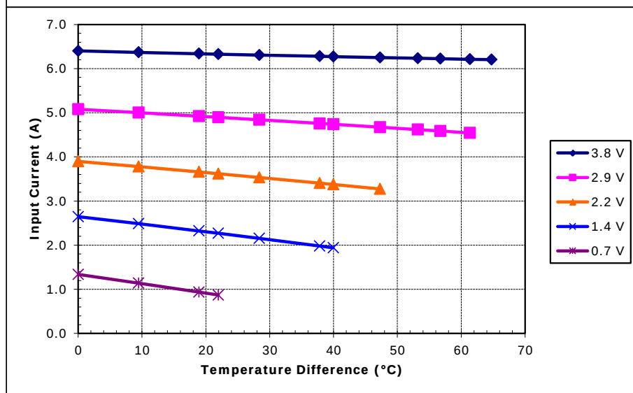
Potted TE-31-1.4-1.5 at a hot-side temperature of 30 °C
