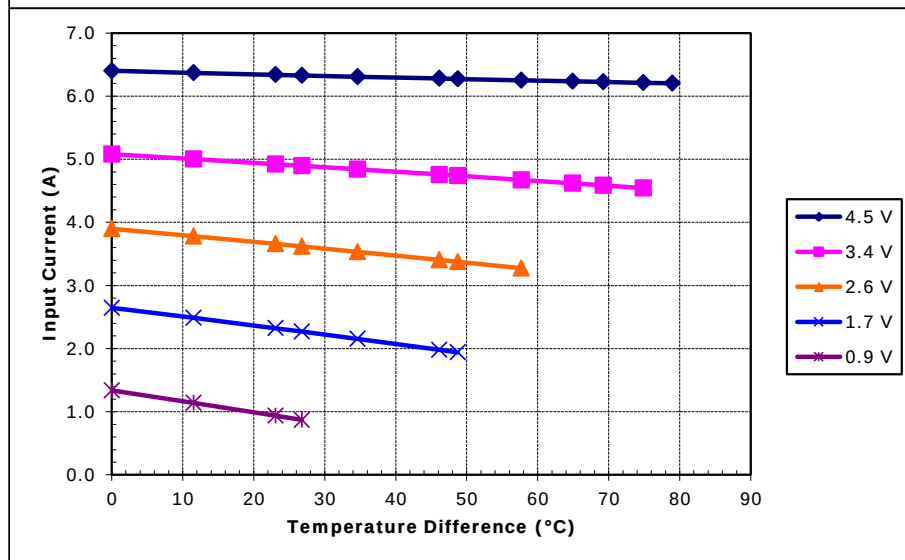
Potted TE-31-1.4-1.5 at a hot-side temperature of 70 °C
