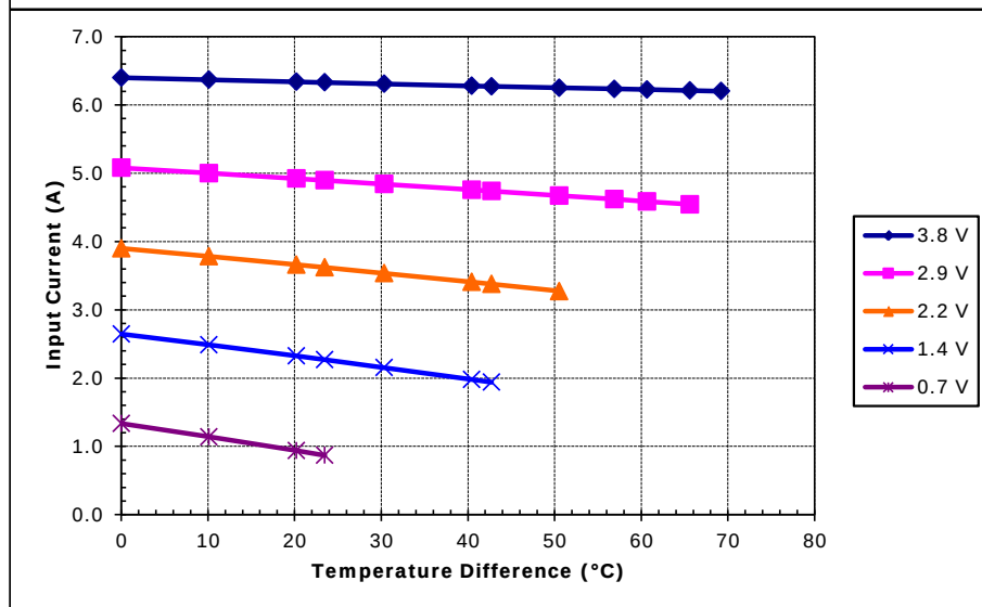
Unpotted TE-31-1.4-1.5 at a hot-side temperature of 30 °C
