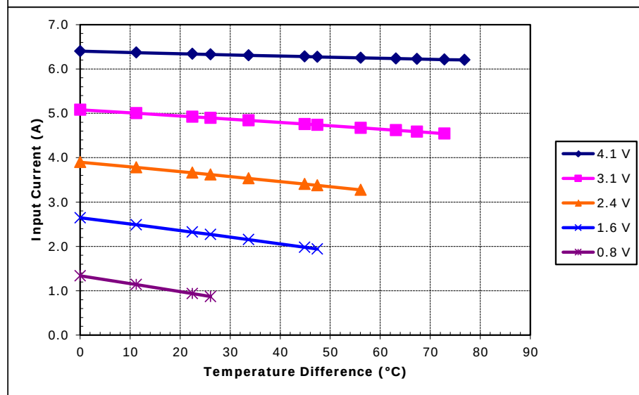
Unpotted TE-31-1.4-1.5 at a hot-side temperature of 50 °C
