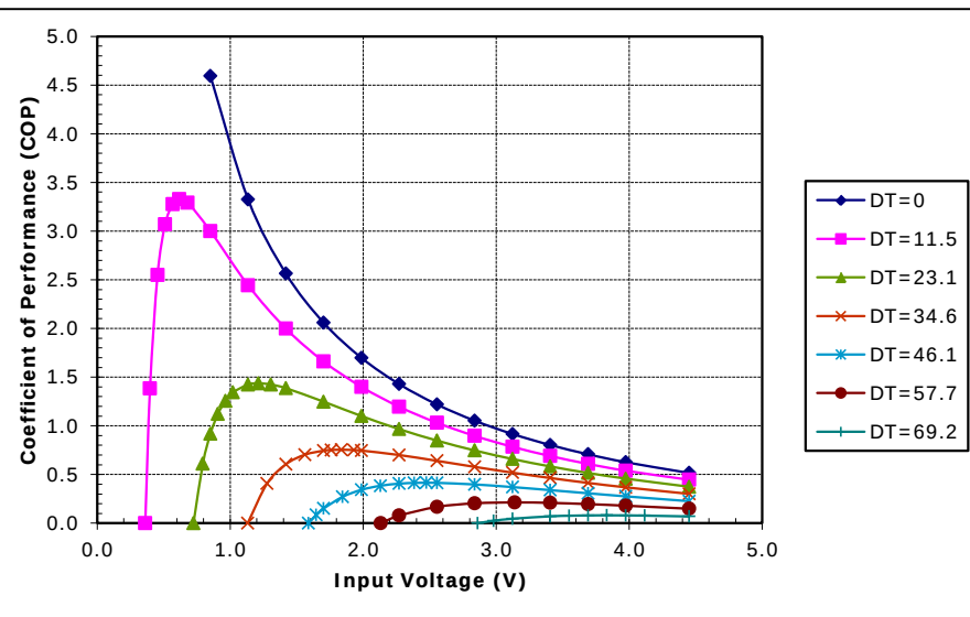
Potted TE-31-1.4-1.5 at a hot-side temperature of 70 °C
