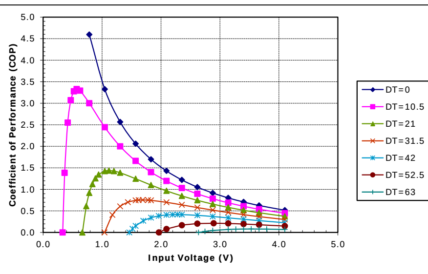
Potted TE-31-1.4-1.5 at a hot-side temperature of 50 °C
