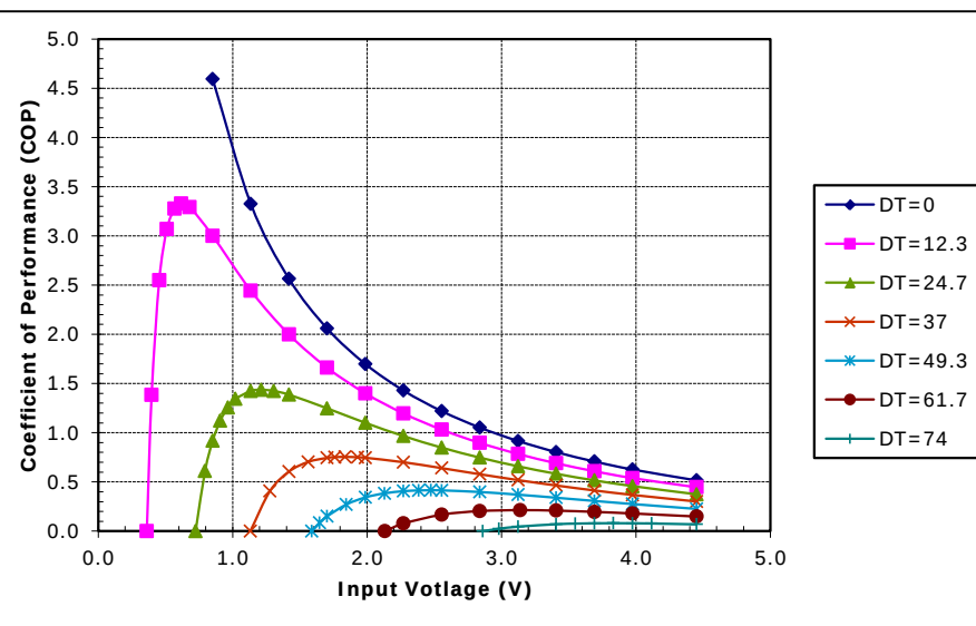
Unpotted TE-31-1.4-1.5 at a hot-side temperature of 70 °C
