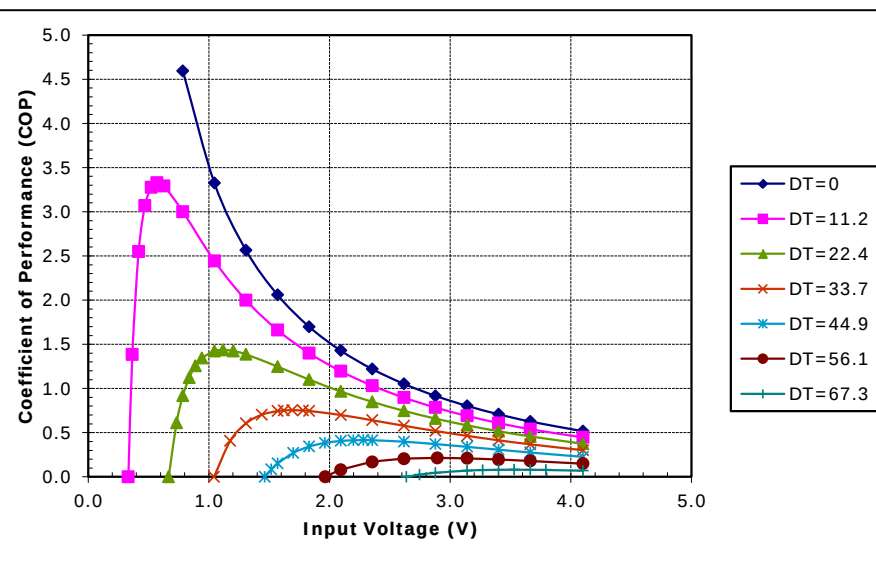
Unpotted TE-31-1.4-1.5 at a hot-side temperature of 50 °C
