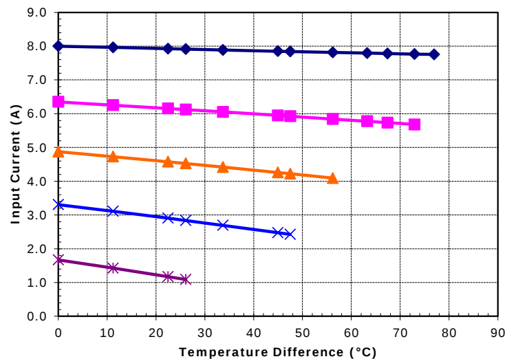
Unpotted TE-17-2.0-2.5 at a hot-side temperature of 50 °C
