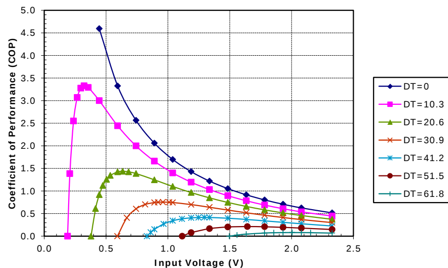
Potted TE-17-2.0-2.5 at a hot-side temperature of 50 °C
