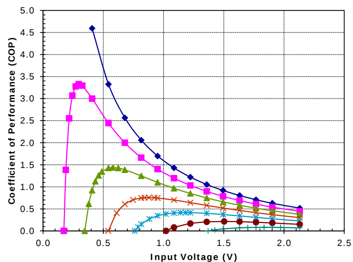
Unpotted TE-17-2.0-2.5 at a hot-side temperature of 30 °C
