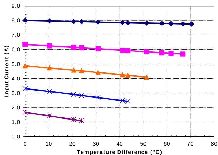
Potted TE-17-2.0-2.5 at a hot-side temperature of 50 °C
