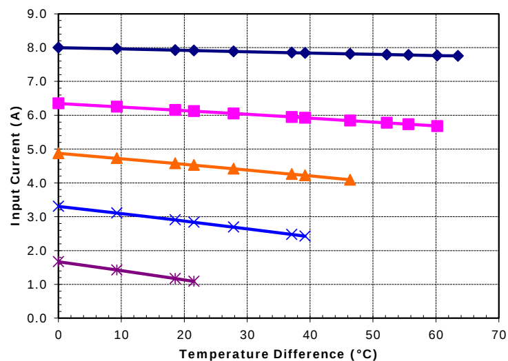
Potted TE-17-2.0-2.5 at a hot-side temperature of 30 °C
