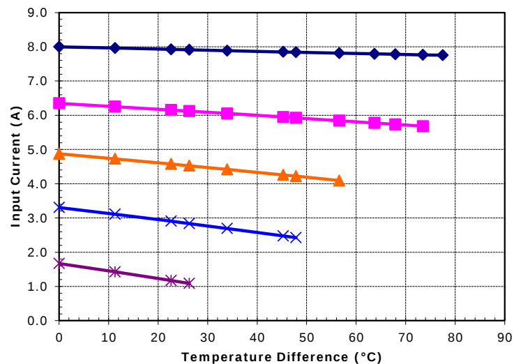
Potted TE-17-2.0-2.5 at a hot-side temperature of 70 °C
