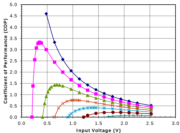
Potted TE-17-2.0-2.5 at a hot-side temperature of 70 °C
