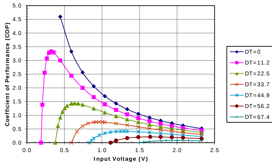
Unpotted TE-17-2.0-2.5 at a hot-side temperature of 50 °C
