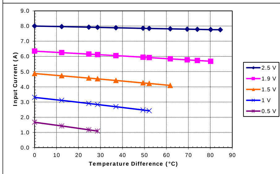
Unpotted TE-17-2.0-2.5 at a hot-side temperature of 70 °C
