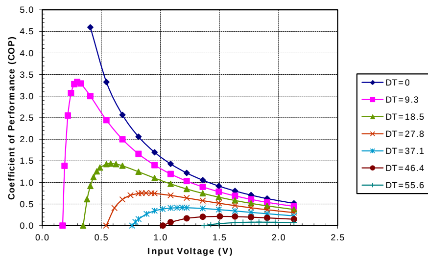
Potted TE-17-2.0-2.5 at a hot-side temperature of 30 °C
