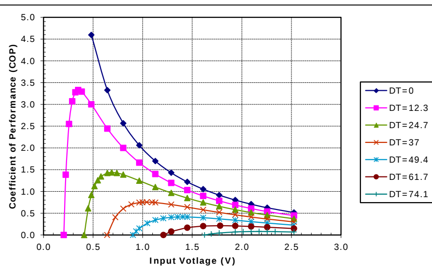
Unpotted TE-17-2.0-2.5 at a hot-side temperature of 70 °C
