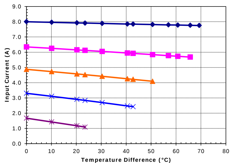
Unpotted TE-17-2.0-2.5 at a hot-side temperature of 30 °C
