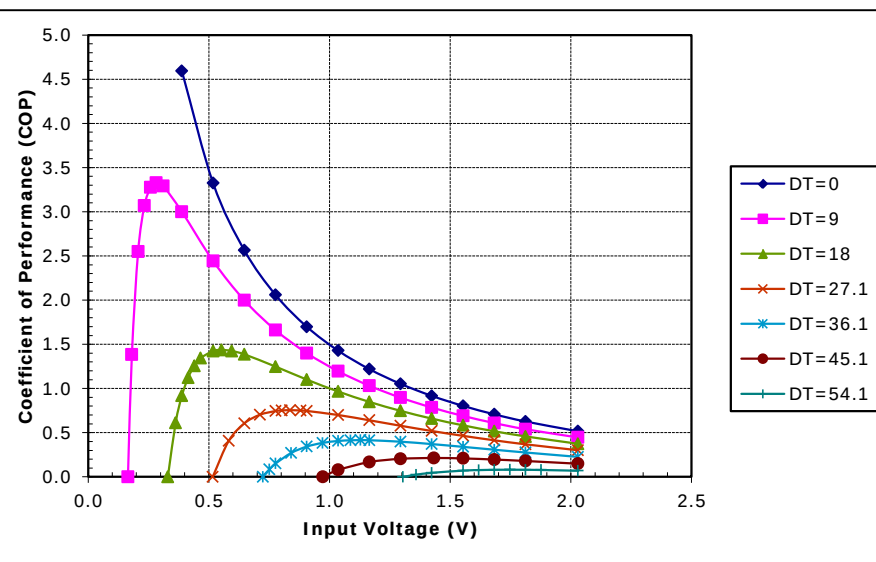
Potted TE-17-2.0-1.5 at a hot-side temperature of 30 °C
