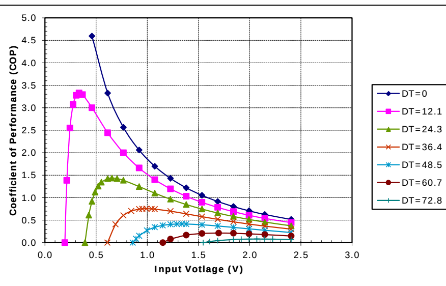
Unpotted TE-17-2.0-1.5 at a hot-side temperature of 70 °C
