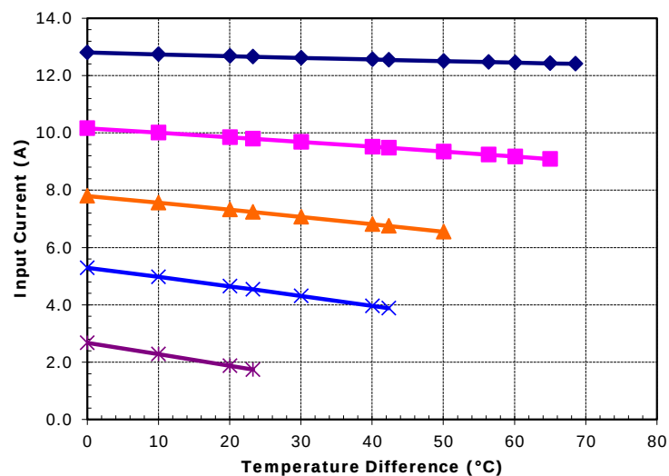
Potted TE-17-2.0-1.5 at a hot-side temperature of 50 °C
