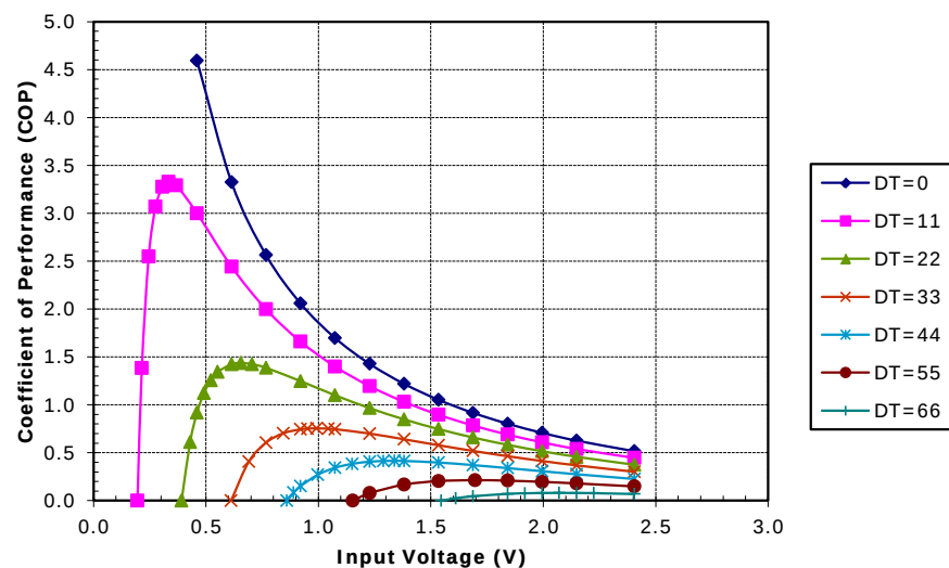
Potted TE-17-2.0-1.5 at a hot-side temperature of 70 °C
