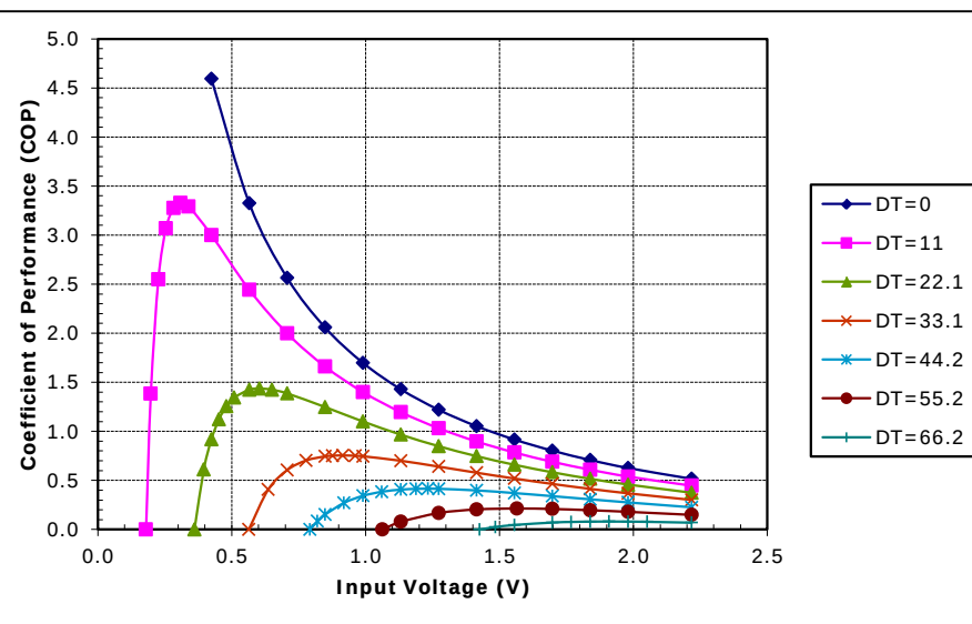
Unpotted TE-17-2.0-1.5 at a hot-side temperature of 50 °C
