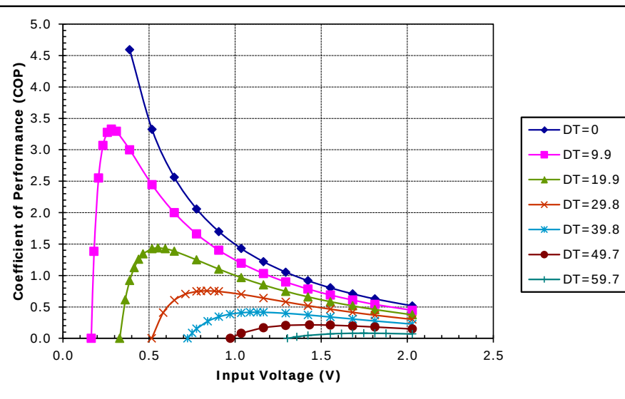
Unpotted TE-17-2.0-1.5 at a hot-side temperature of 30 °C
