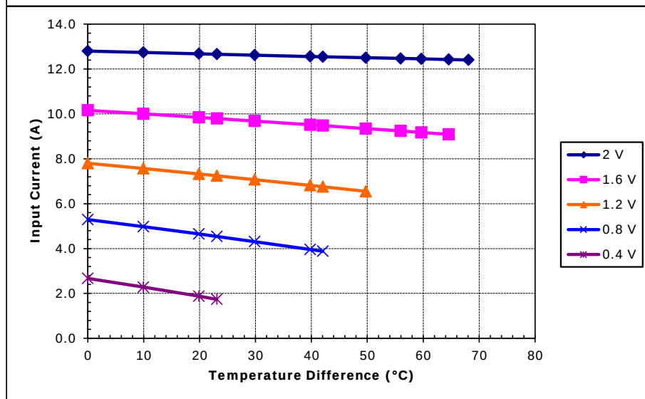
Unpotted TE-17-2.0-1.5 at a hot-side temperature of 30 °C
