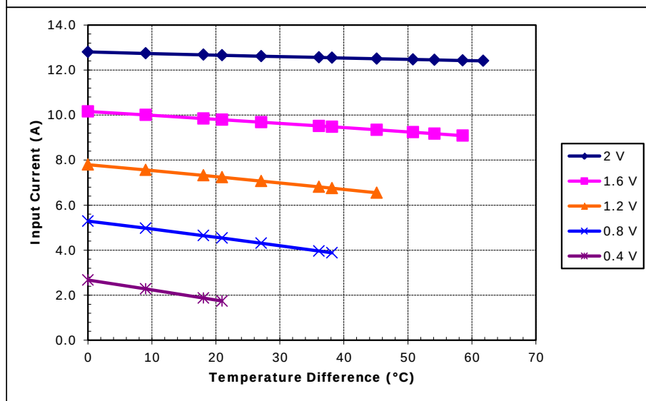
Potted TE-17-2.0-1.5 at a hot-side temperature of 30 °C
