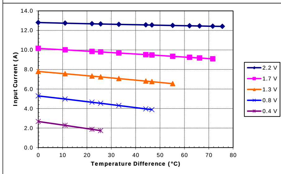
Unpotted TE-17-2.0-1.5 at a hot-side temperature of 50 °C
