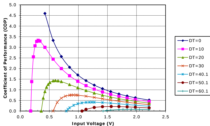
Potted TE-17-2.0-1.5 at a hot-side temperature of 50 °C
