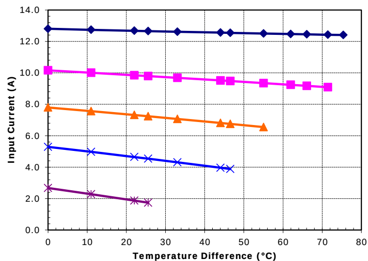
Potted TE-17-2.0-1.5 at a hot-side temperature of 70 °C
