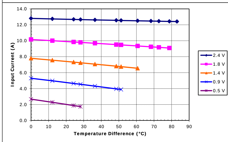
Unpotted TE-17-2.0-1.5 at a hot-side temperature of 70 °C
