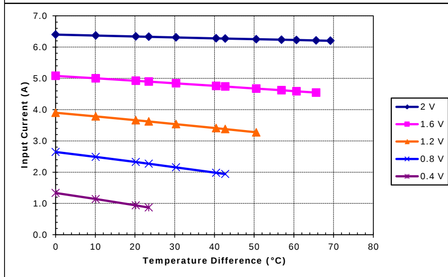
Unpotted TE-17-1.4-1.5 at a hot-side temperature of 30 °C
