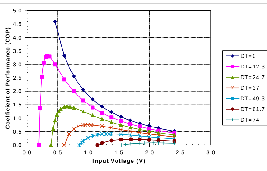
Unpotted TE-17-1.4-1.5 at a hot-side temperature of 70 °C
