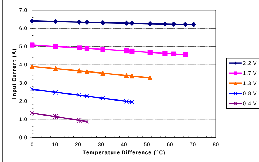
Potted TE-17-1.4-1.5 at a hot-side temperature of 50 °C
