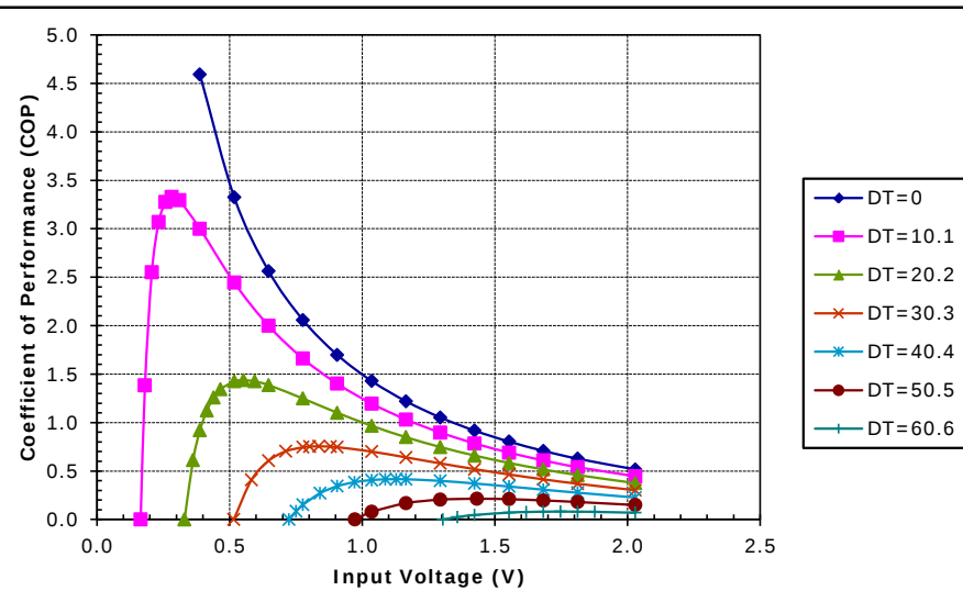
Unpotted TE-17-1.4-1.5 at a hot-side temperature of 30 °C
