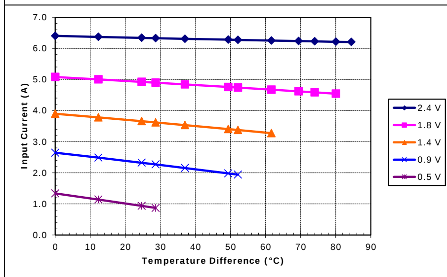
Unpotted TE-17-1.4-1.5 at a hot-side temperature of 70 °C
