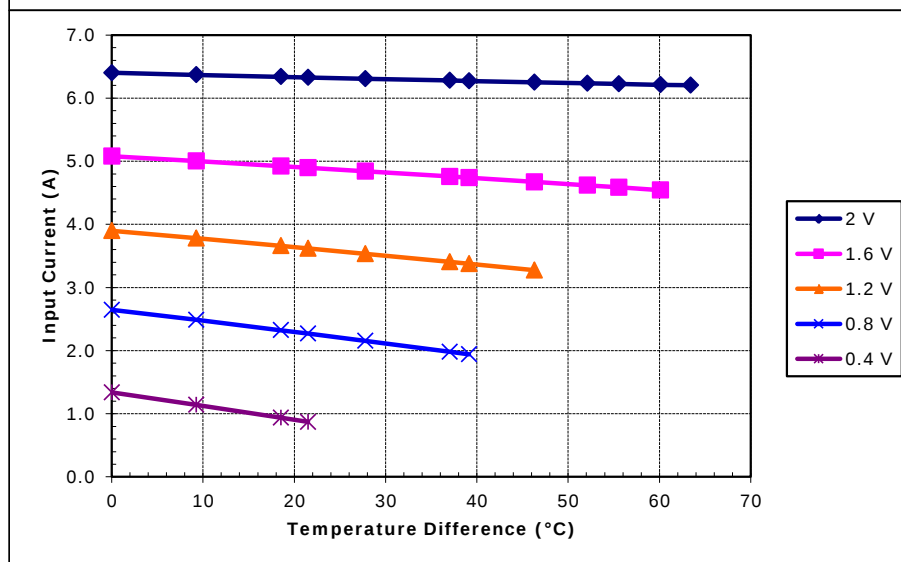
Potted TE-17-1.4-1.5 at a hot-side temperature of 30 °C
