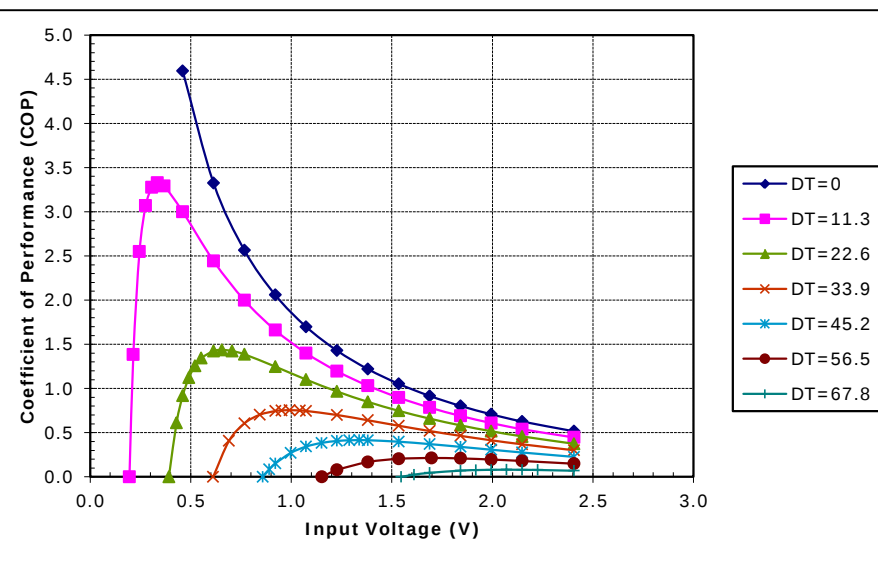
Potted TE-17-1.4-1.5 at a hot-side temperature of 70 °C
