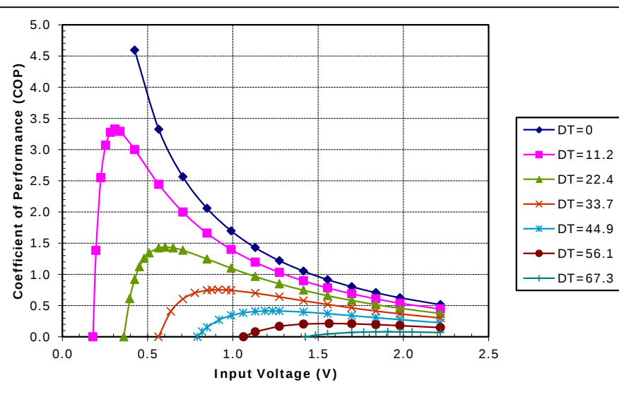
Unpotted TE-17-1.4-1.5 at a hot-side temperature of 50 °C
