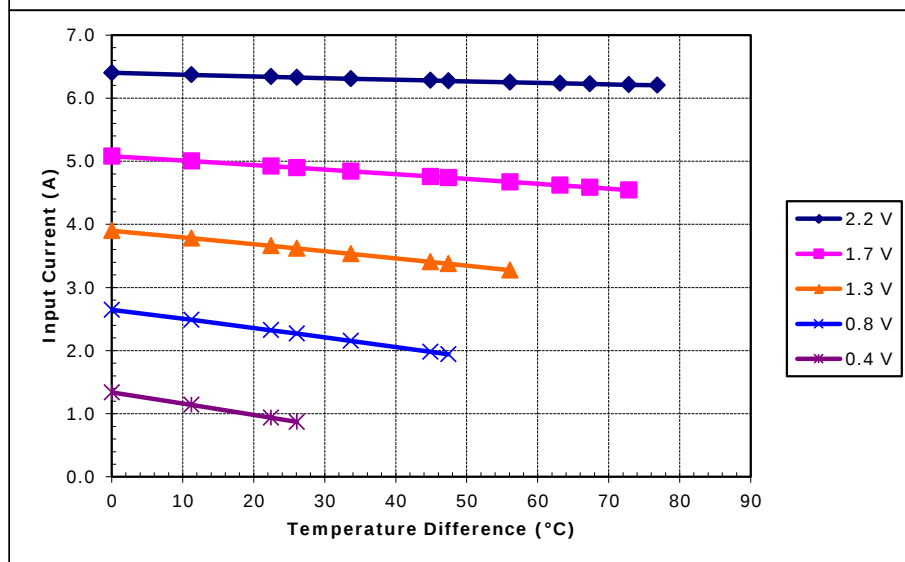
Unpotted TE-17-1.4-1.5 at a hot-side temperature of 50 °C
