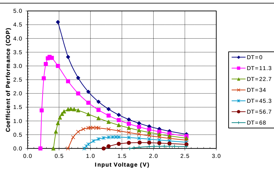
Potted TE-17-1.0-2.5 at a hot-side temperature of 70 °C
