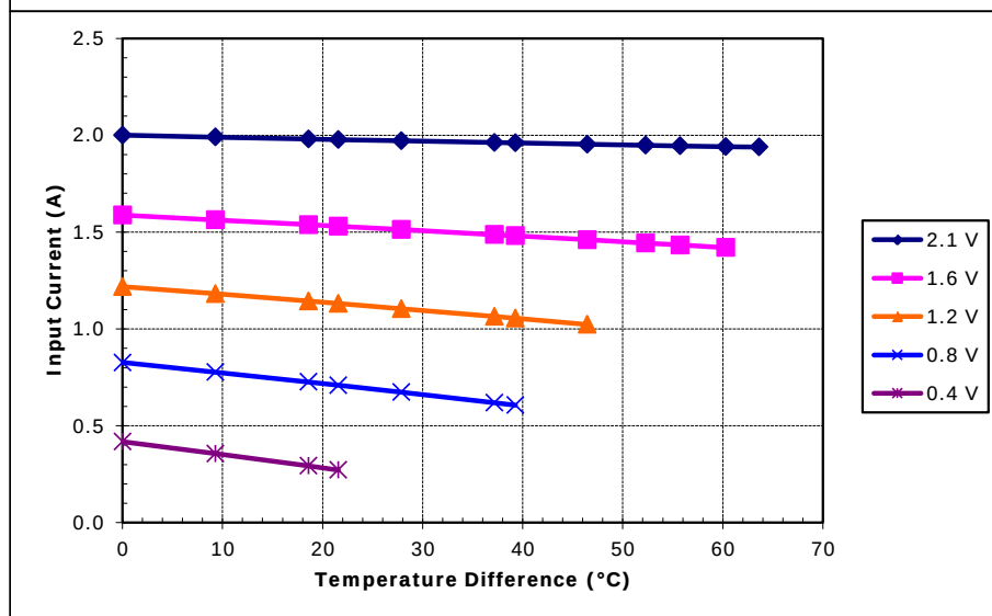
Potted TE-17-1.0-2.5 at a hot-side temperature of 30 °C
