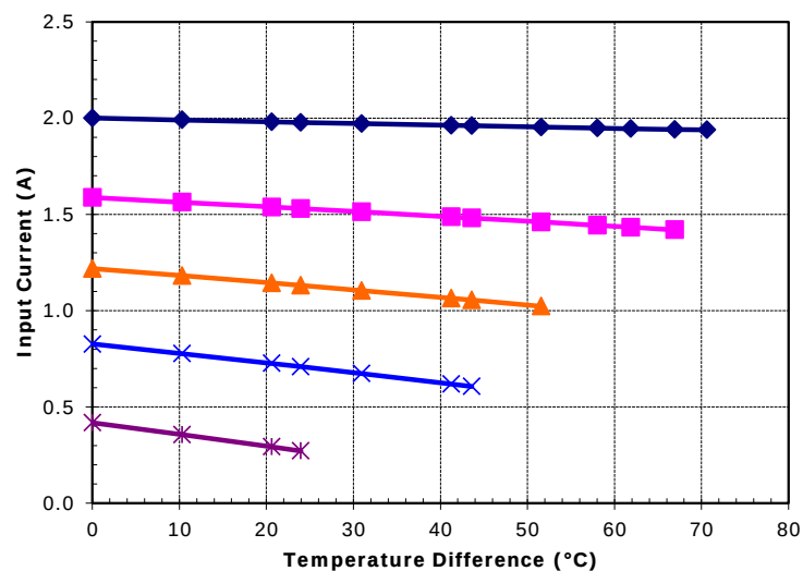
Potted TE-17-1.0-2.5 at a hot-side temperature of 50 °C
