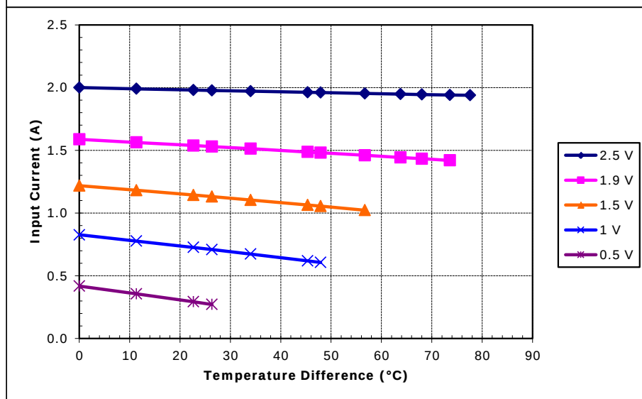
Potted TE-17-1.0-2.5 at a hot-side temperature of 70 °C
