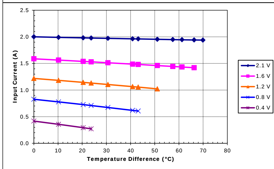
Unpotted TE-17-1.0-2.5 at a hot-side temperature of 30 °C
