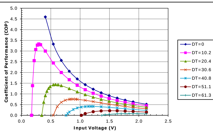
Unpotted TE-17-1.0-2.5 at a hot-side temperature of 30 °C
