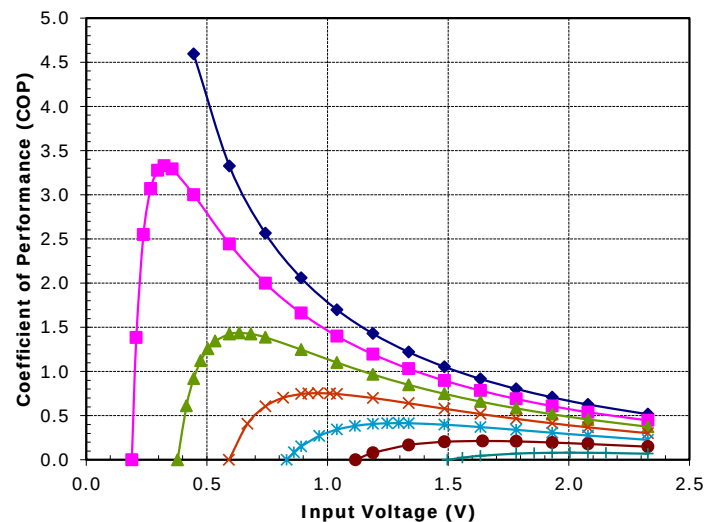
Unpotted TE-17-1.0-2.5 at a hot-side temperature of 50 °C
