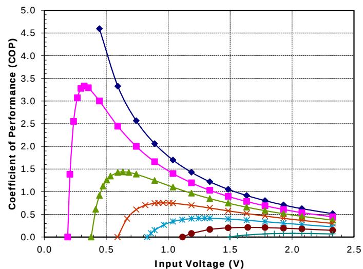
Potted TE-17-1.0-2.5 at a hot-side temperature of 50 °C
