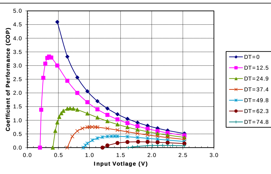
Unpotted TE-17-1.0-2.5 at a hot-side temperature of 70 °C
