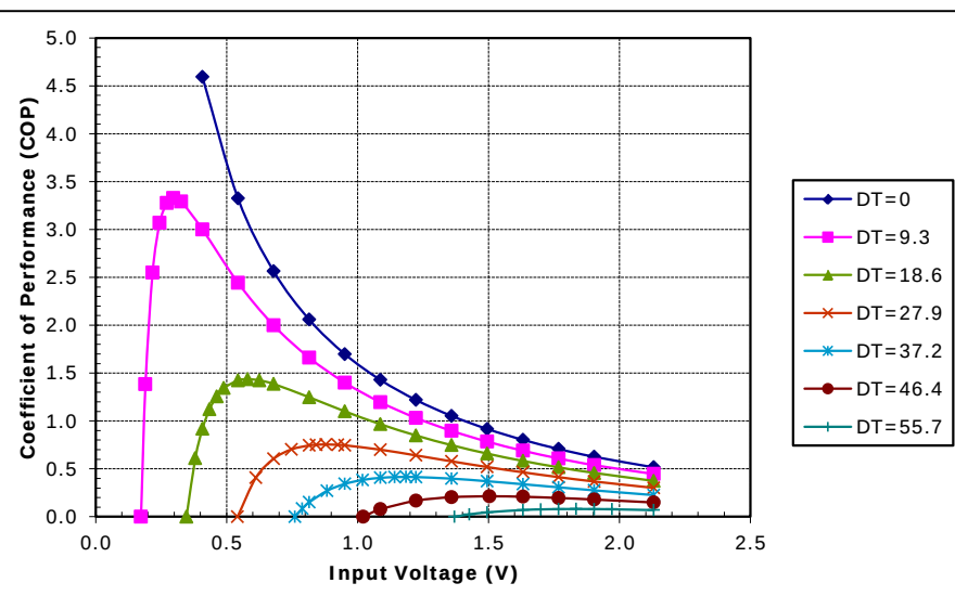
Potted TE-17-1.0-2.5 at a hot-side temperature of 30 °C
