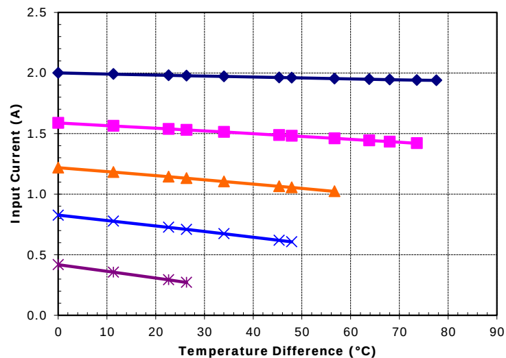
Unpotted TE-17-1.0-2.5 at a hot-side temperature of 50 °C
