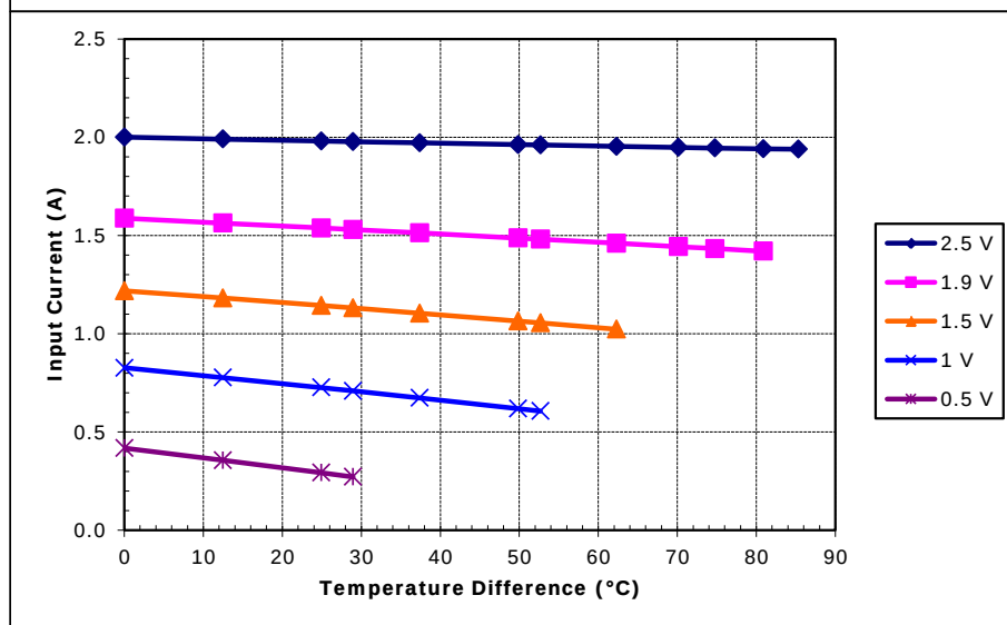
Unpotted TE-17-1.0-2.5 at a hot-side temperature of 70 °C
