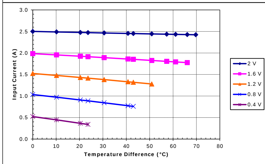
Unpotted TE-17-1.0-2.0 at a hot-side temperature of 30 °C
