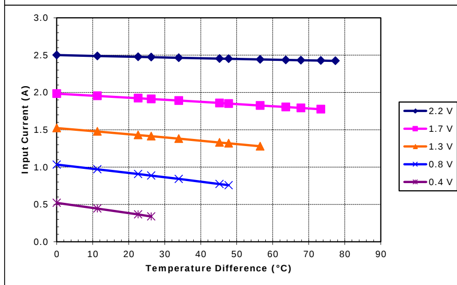
Unpotted TE-17-1.0-2.0 at a hot-side temperature of 50 °C
