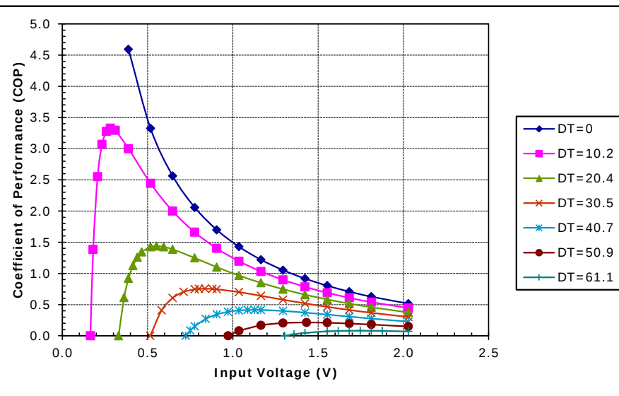
Unpotted TE-17-1.0-2.0 at a hot-side temperature of 30 °C
