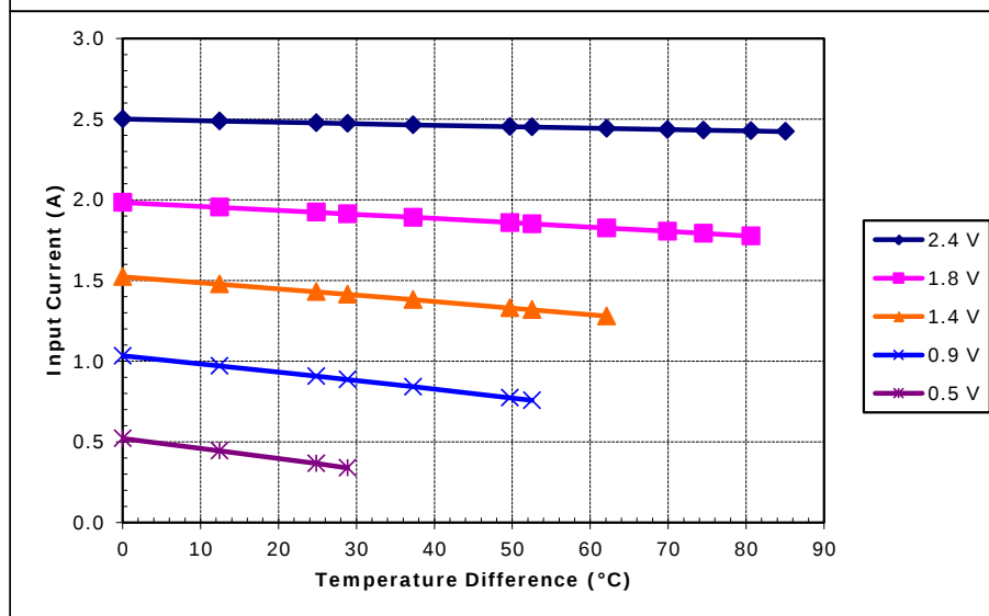
Unpotted TE-17-1.0-2.0 at a hot-side temperature of 70 °C
