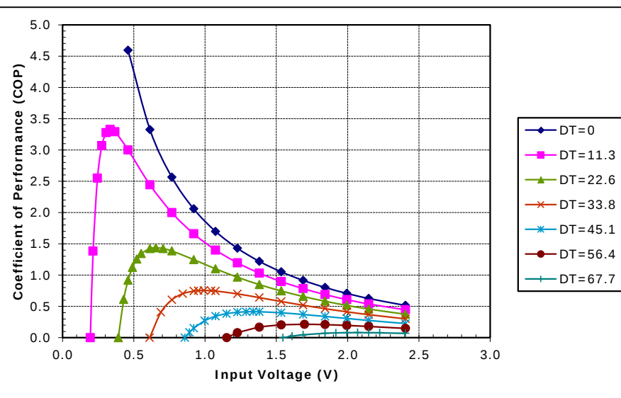
Potted TE-17-1.0-2.0 at a hot-side temperature of 70 °C
