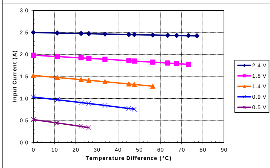
Potted TE-17-1.0-2.0 at a hot-side temperature of 70 °C
