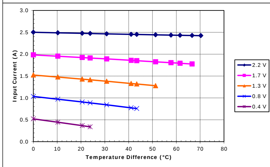
Potted TE-17-1.0-2.0 at a hot-side temperature of 50 °C
