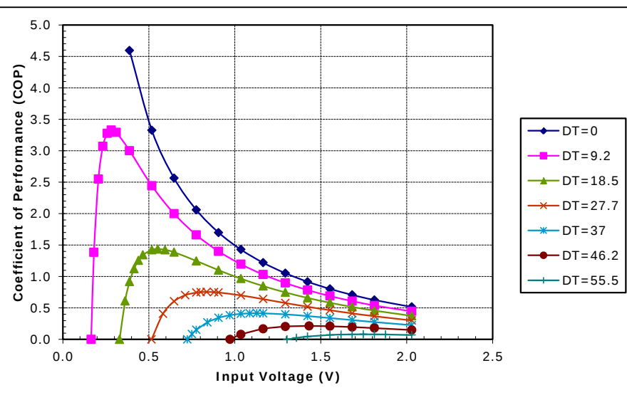
Potted TE-17-1.0-2.0 at a hot-side temperature of 30 °C
