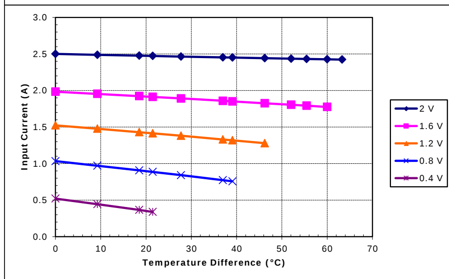
Potted TE-17-1.0-2.0 at a hot-side temperature of 30 °C
