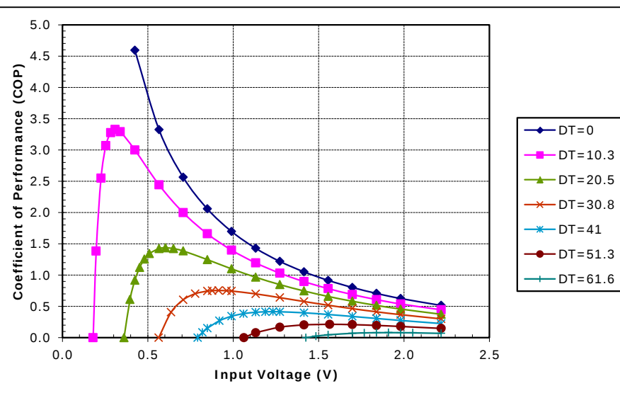
Potted TE-17-1.0-2.0 at a hot-side temperature of 50 °C
