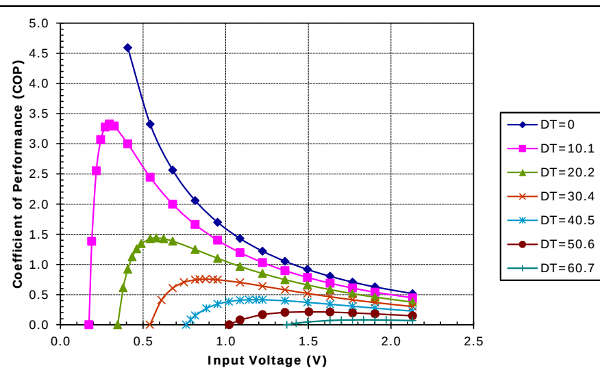
Unpotted TE-17-1.0-1.5 at a hot-side temperature of 30 °C
