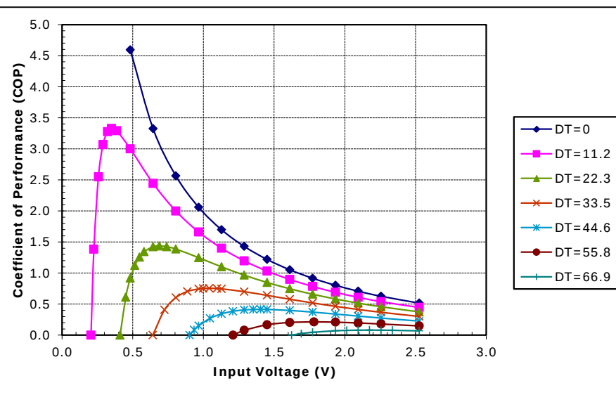
Potted TE-17-1.0-1.5 at a hot-side temperature of 70 °C
