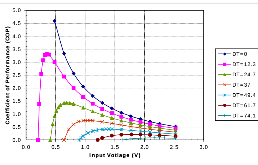
Unpotted TE-17-1.0-1.5 at a hot-side temperature of 70 °C
