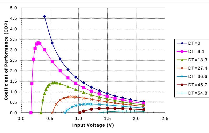
Potted TE-17-1.0-1.5 at a hot-side temperature of 30 °C
