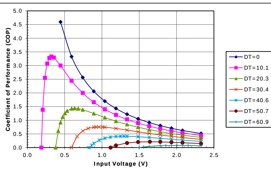
Potted TE-17-1.0-1.5 at a hot-side temperature of 50 °C
