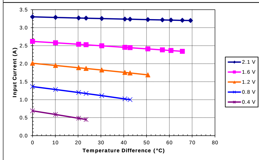
Unpotted TE-17-1.0-1.5 at a hot-side temperature of 30 °C
