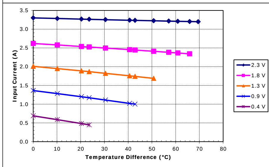
Potted TE-17-1.0-1.5 at a hot-side temperature of 50 °C
