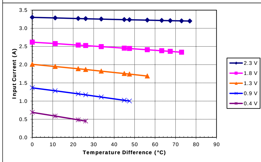
Unpotted TE-17-1.0-1.5 at a hot-side temperature of 50 °C
