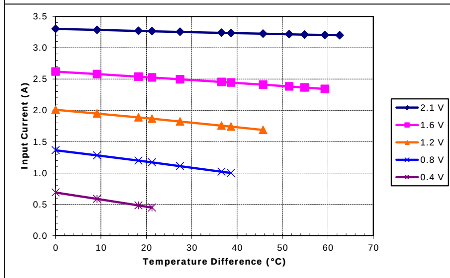
Potted TE-17-1.0-1.5 at a hot-side temperature of 30 °C
