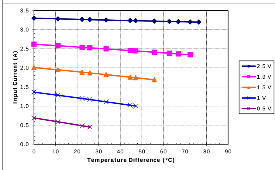
Potted TE-17-1.0-1.5 at a hot-side temperature of 70 °C
