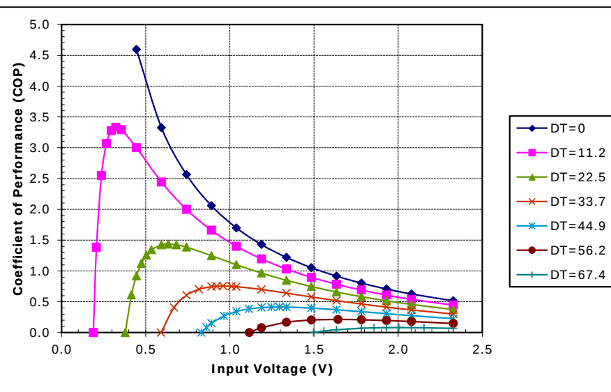
Unpotted TE-17-1.0-1.5 at a hot-side temperature of 50 °C
