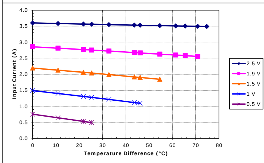
Potted TE-17-1.0-1.3 at a hot-side temperature of 70 °C
