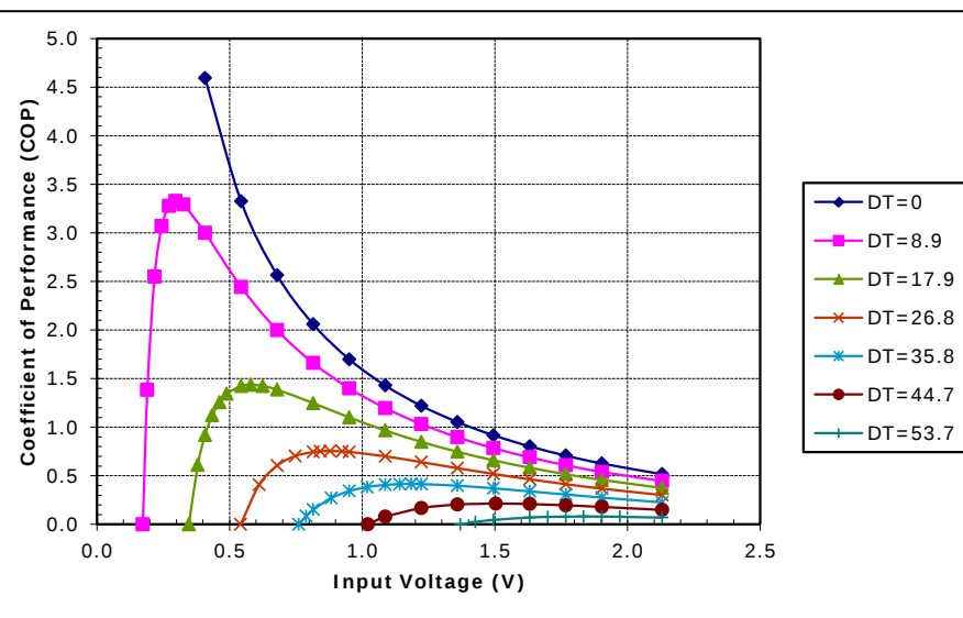
Potted TE-17-1.0-1.3 at a hot-side temperature of 30 °C
