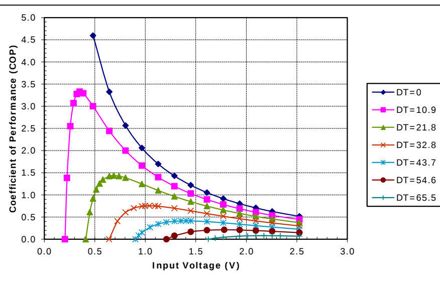
Potted TE-17-1.0-1.3 at a hot-side temperature of 70 °C
