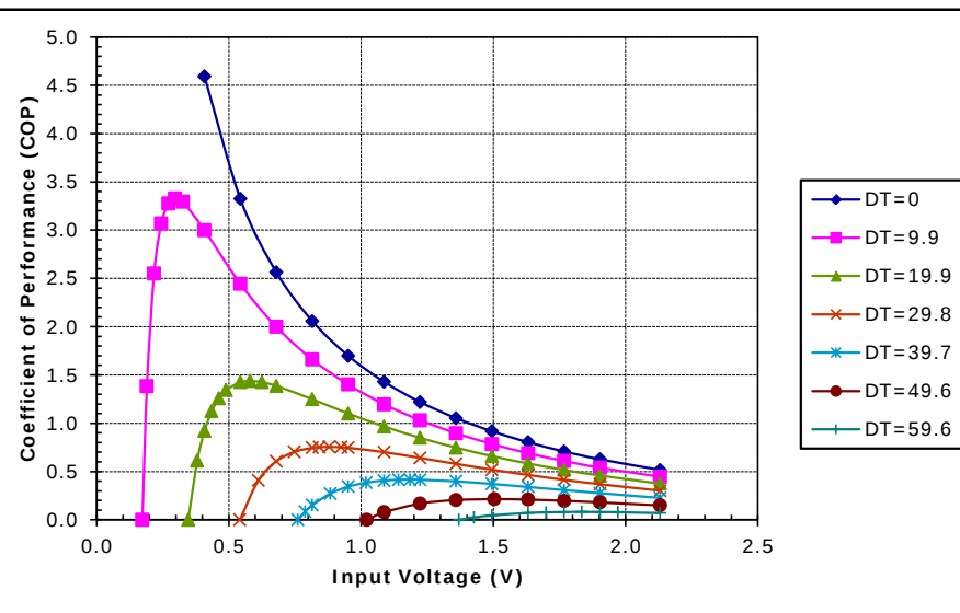
Unpotted TE-17-1.0-1.3 at a hot-side temperature of 30 °C
