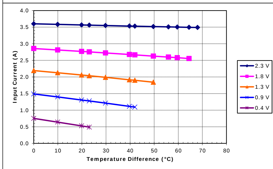
Potted TE-17-1.0-1.3 at a hot-side temperature of 50 °C
