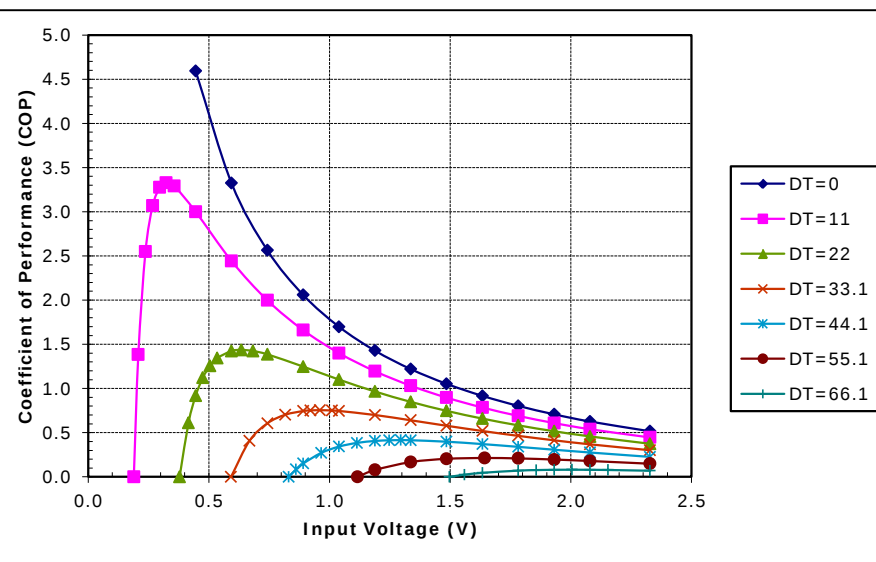
Unpotted TE-17-1.0-1.3 at a hot-side temperature of 50 °C
