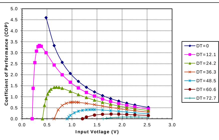
Unpotted TE-17-1.0-1.3 at a hot-side temperature of 70 °C
