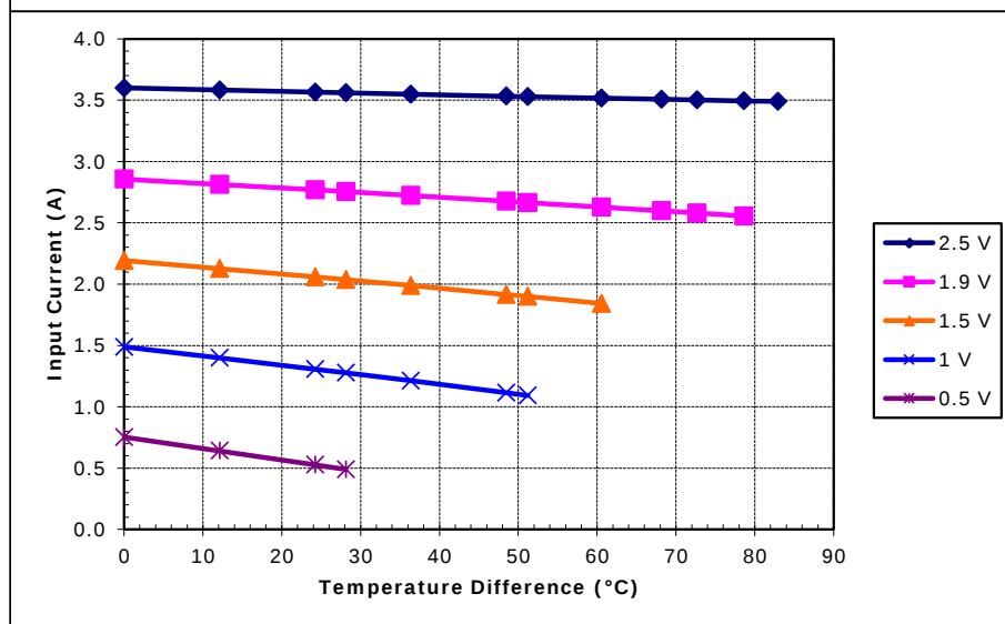
Unpotted TE-17-1.0-1.3 at a hot-side temperature of 70 °C
