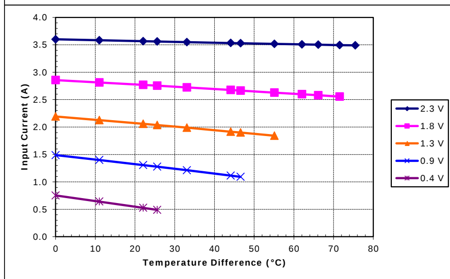
Unpotted TE-17-1.0-1.3 at a hot-side temperature of 50 °C
