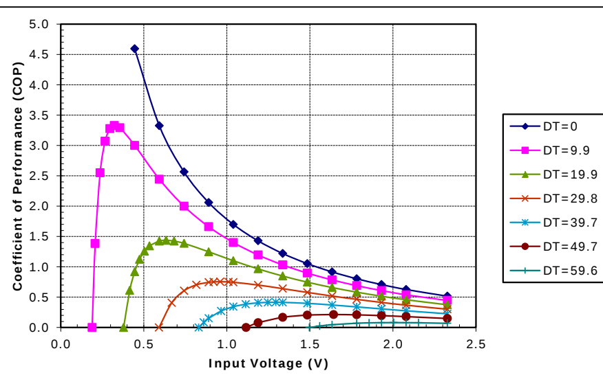
Potted TE-17-1.0-1.3 at a hot-side temperature of 50 °C
