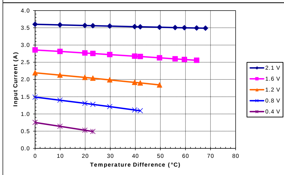
Unpotted TE-17-1.0-1.3 at a hot-side temperature of 30 °C
