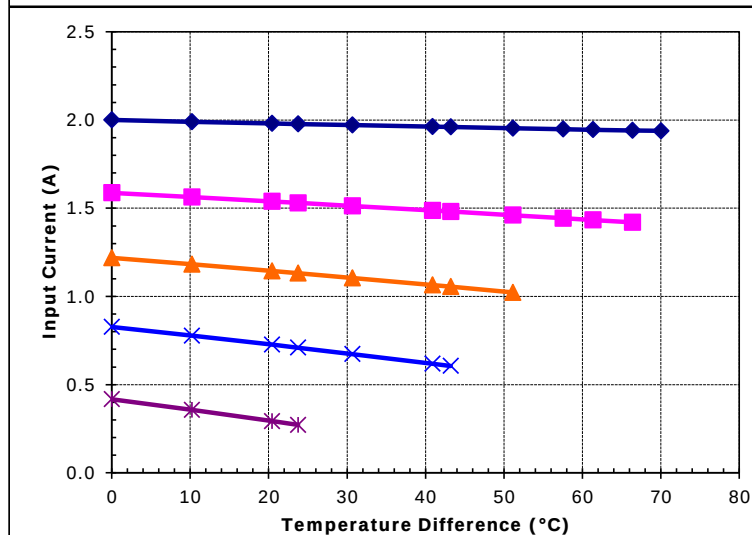
Unpotted TE-127-1.0-2.5 at a hot-side temperature of 30 °C
