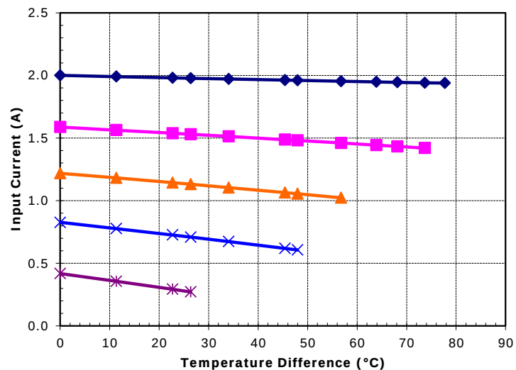
Unpotted TE-127-1.0-2.5 at a hot-side temperature of 50 °C
