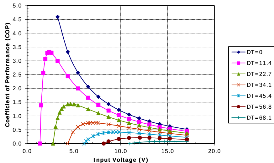
Unpotted TE-127-1.0-2.5 at a hot-side temperature of 50 °C
