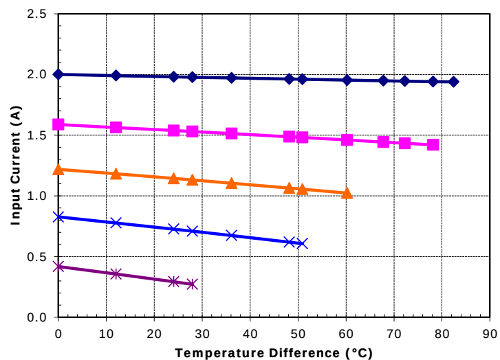
Potted TE-127-1.0-2.5 at a hot-side temperature of 70 °C
