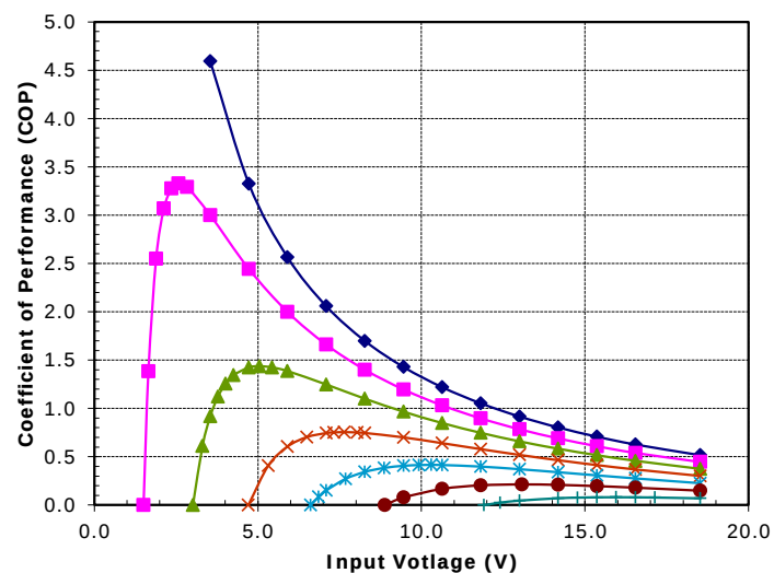
Unpotted TE-127-1.0-2.5 at a hot-side temperature of 70 °C
