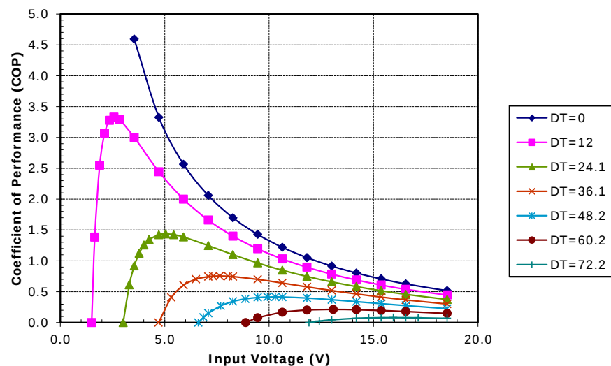
Potted TE-127-1.0-2.5 at a hot-side temperature of 70 °C
