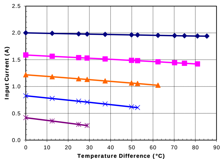
Unpotted TE-127-1.0-2.5 at a hot-side temperature of 70 °C
