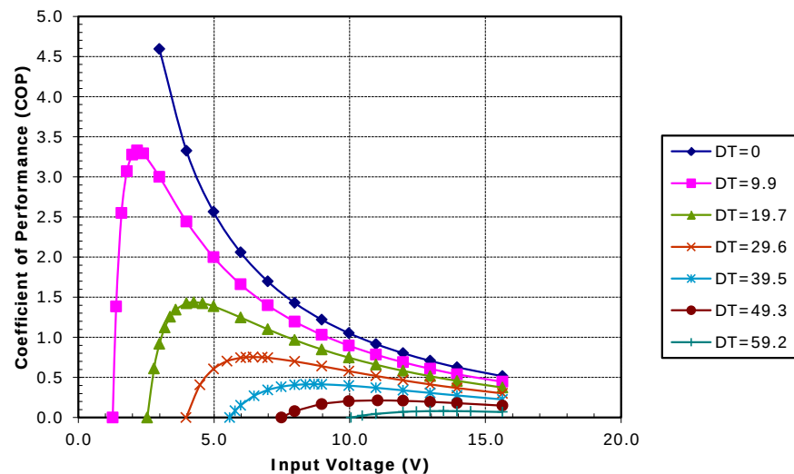
Potted TE-127-1.0-2.5 at a hot-side temperature of 30 °C
