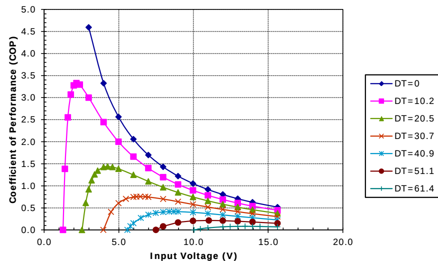
Unpotted TE-127-1.0-2.5 at a hot-side temperature of 30 °C
