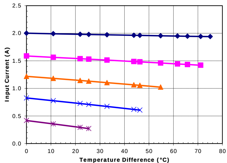
Potted TE-127-1.0-2.5 at a hot-side temperature of 50 °C
