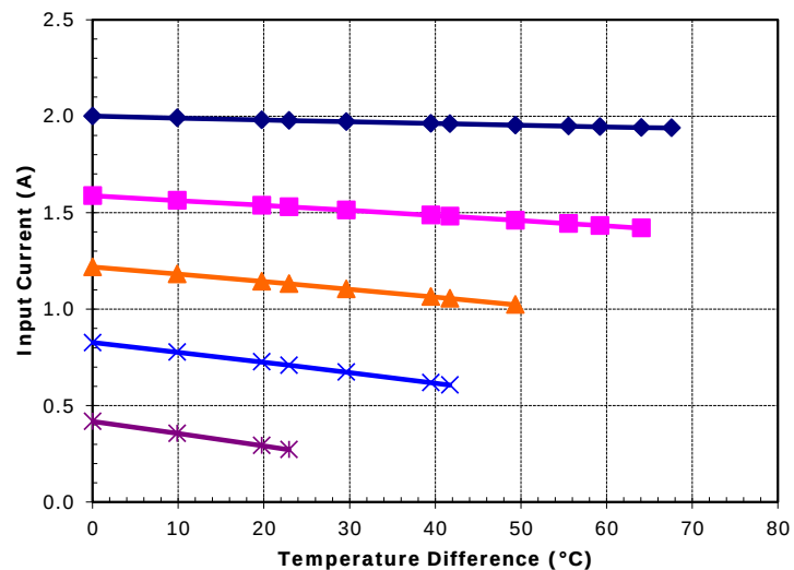
Potted TE-127-1.0-2.5 at a hot-side temperature of 30 °C
