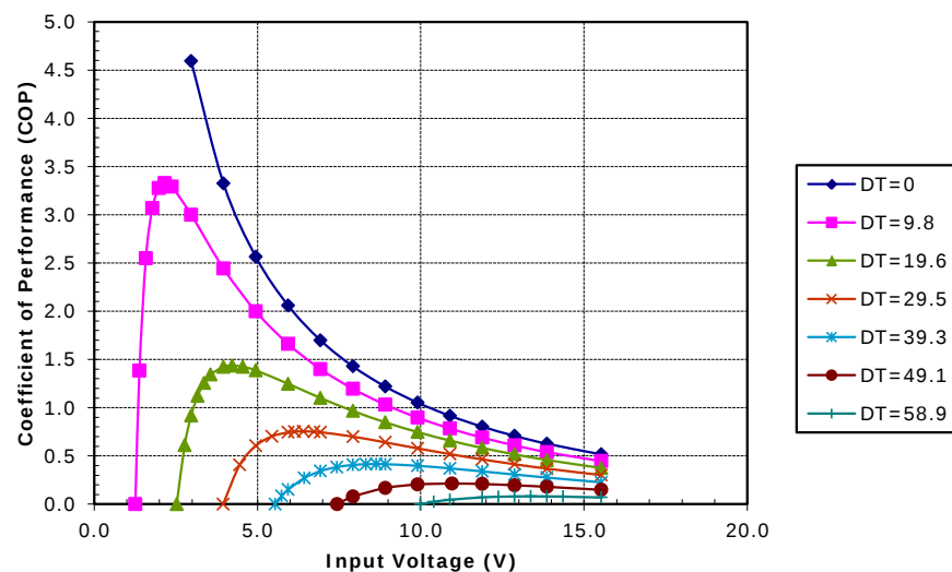
Potted TE-127-1.0-2.0 at a hot-side temperature of 30 °C
