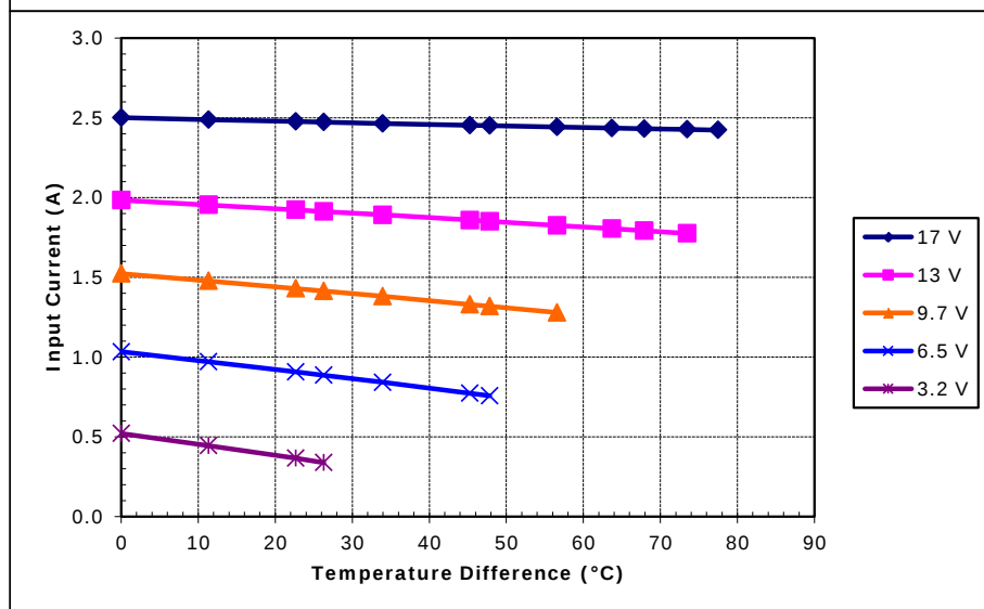
Unpotted TE-127-1.0-2.0 at a hot-side temperature of 50 °C
