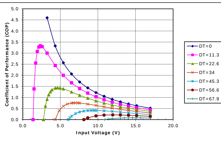
Unpotted TE-127-1.0-2.0 at a hot-side temperature of 50 °C
