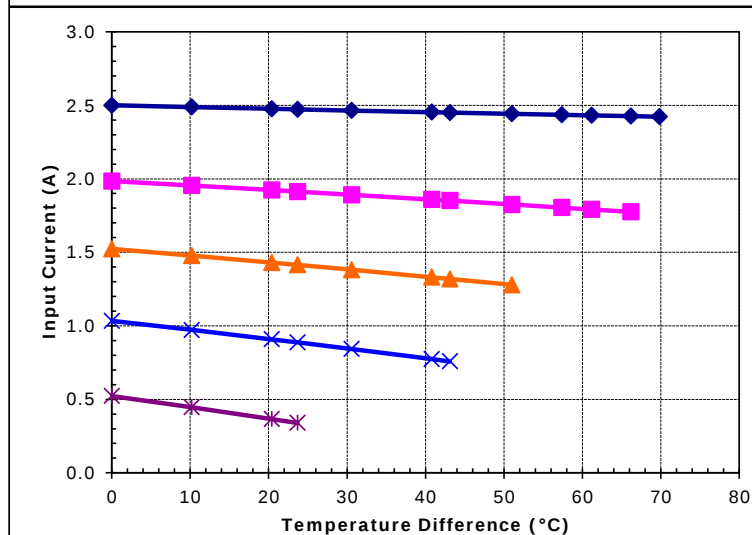
Unpotted TE-127-1.0-2.0 at a hot-side temperature of 30 °C
