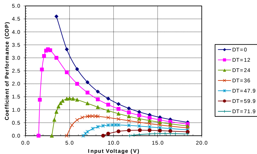
Potted TE-127-1.0-2.0 at a hot-side temperature of 70 °C
