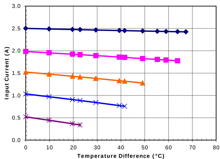
Potted TE-127-1.0-2.0 at a hot-side temperature of 30 °C
