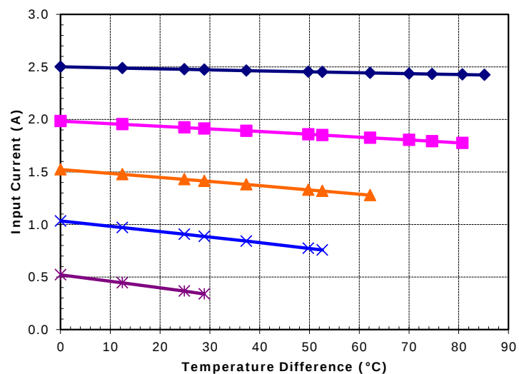
Unpotted TE-127-1.0-2.0 at a hot-side temperature of 70 °C
