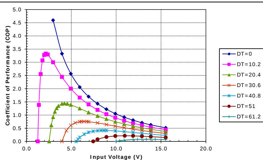
Unpotted TE-127-1.0-2.0 at a hot-side temperature of 30 °C
