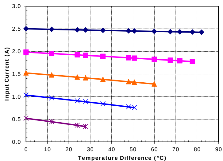
Potted TE-127-1.0-2.0 at a hot-side temperature of 70 °C
