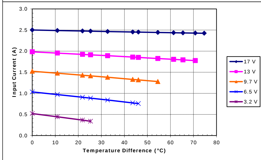
Potted TE-127-1.0-2.0 at a hot-side temperature of 50 °C
