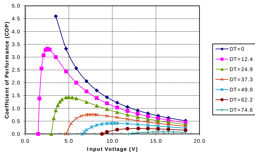
Unpotted TE-127-1.0-2.0 at a hot-side temperature of 70 °C
