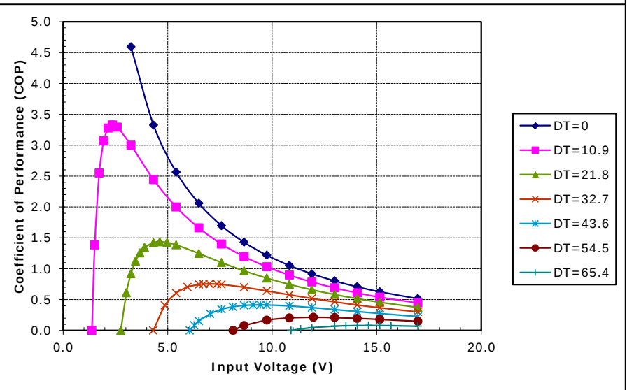
Potted TE-127-1.0-2.0 at a hot-side temperature of 50 °C
