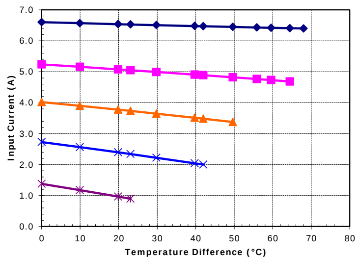
Potted SP-254-1.0-1.5 (Parallel) at a hot-side temperature of 30 °C
