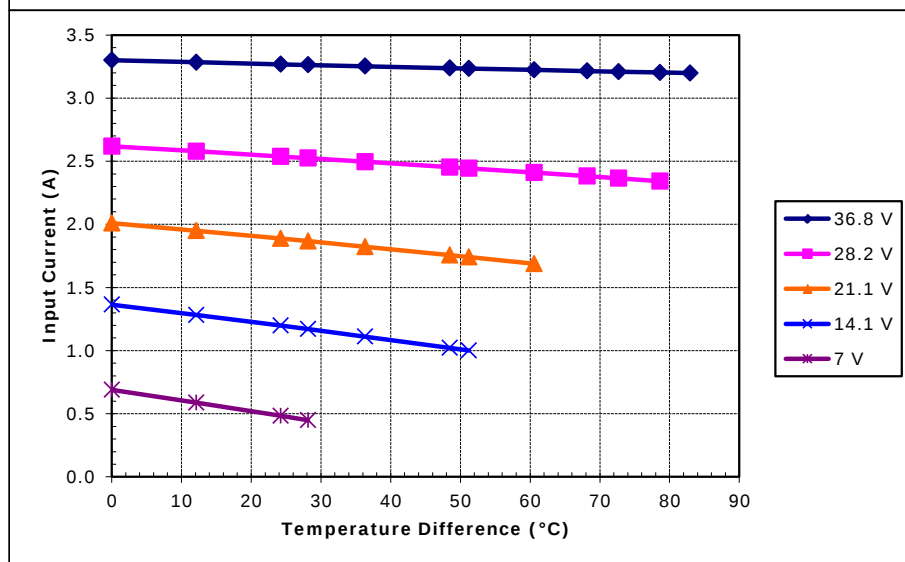
Potted SP-254-1.0-1.5 (Series) at a hot-side temperature of 70 °C
