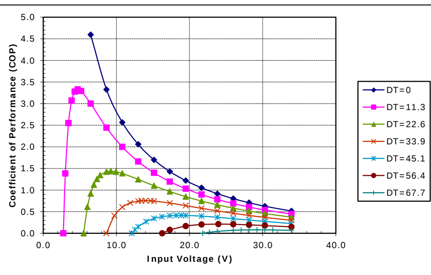
Unpotted SP-254-1.0-1.5 (Series) at a hot-side temperature of 50 °C
