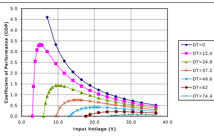
Unpotted SP-254-1.0-1.5 (Series) at a hot-side temperature of 70 °C
