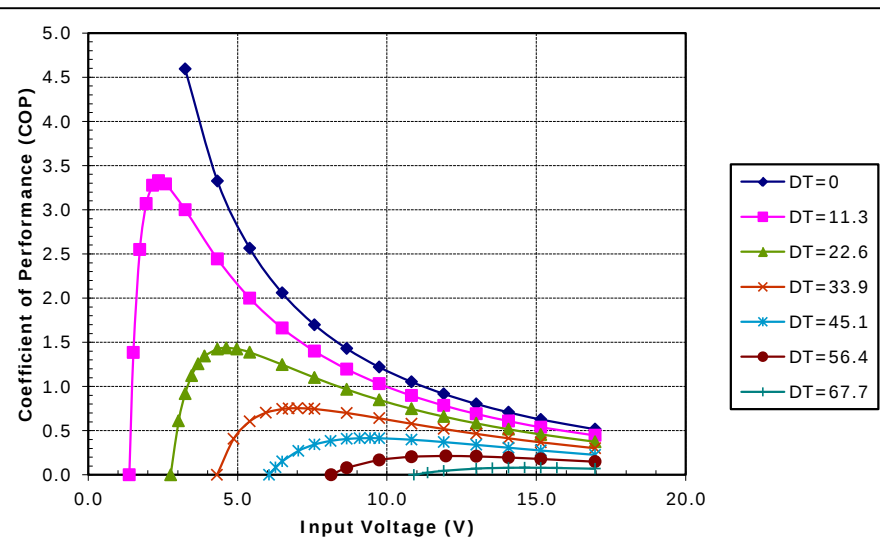
Unpotted SP-254-1.0-1.5 (Parallel) at a hot-side temperature of 50 °C
