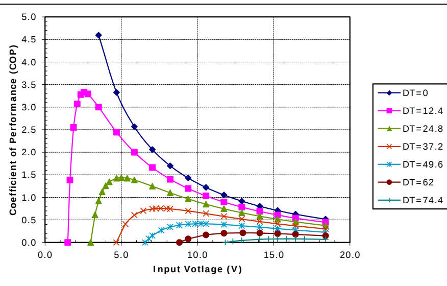
Unpotted SP-254-1.0-1.5 (Parallel) at a hot-side temperature of 70 °C
