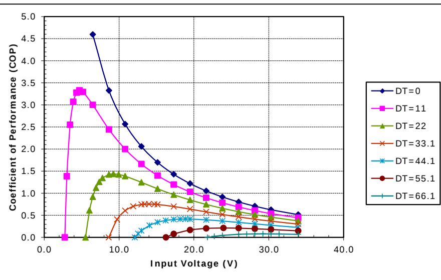
Potted SP-254-1.0-1.5 (Series) at a hot-side temperature of 50 °C
