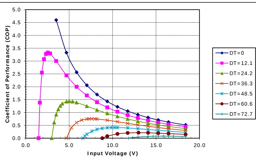
Potted SP-254-1.0-1.5 (Parallel) at a hot-side temperature of 70 °C
