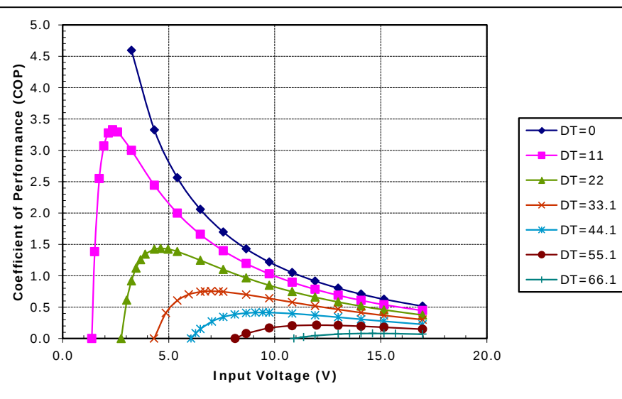
Potted SP-254-1.0-1.5 (Parallel) at a hot-side temperature of 50 °C
