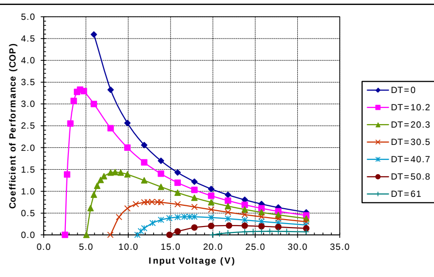
Unpotted SP-254-1.0-1.5 (Series) at a hot-side temperature of 30 °C
