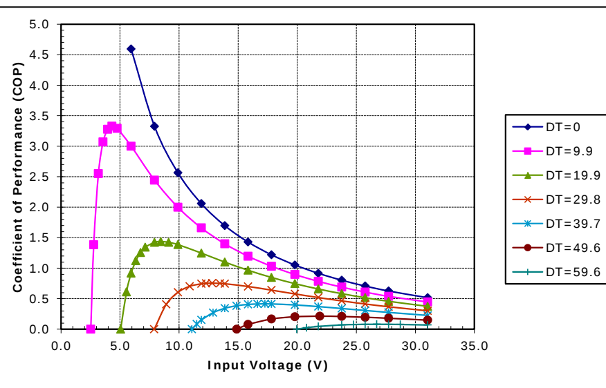
Potted SP-254-1.0-1.5 (Series) at a hot-side temperature of 30 °C
