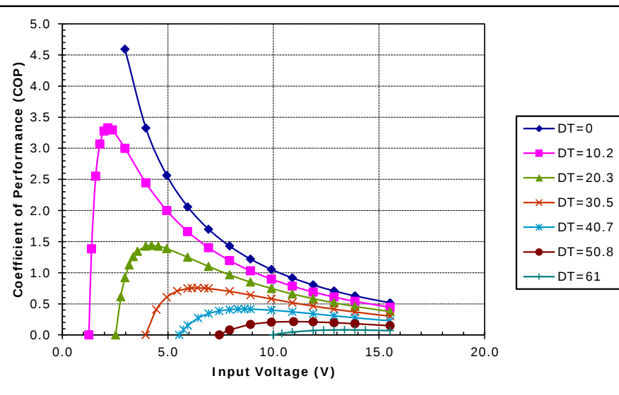
Unpotted SP-254-1.0-1.5 (Parallel) at a hot-side temperature of 30 °C
