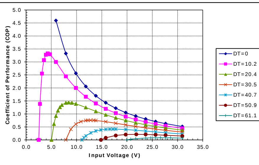
Unpotted RD-253-1.4-1.5 at a hot-side temperature of 30 °C
