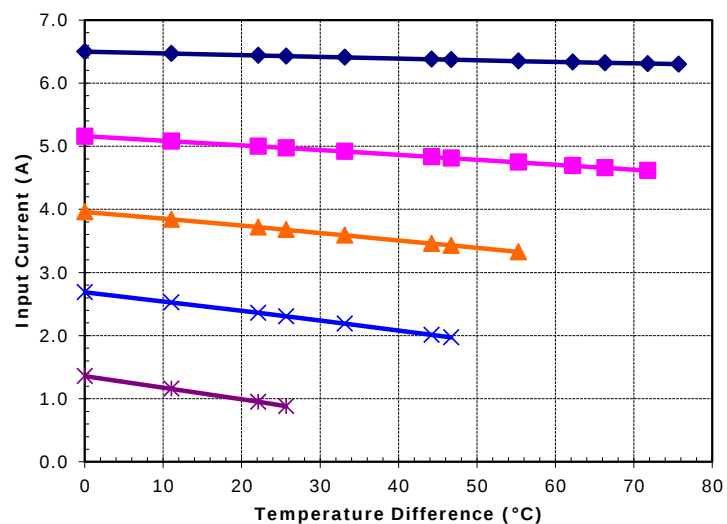
Potted RD-253-1.4-1.5 at a hot-side temperature of 50 °C
