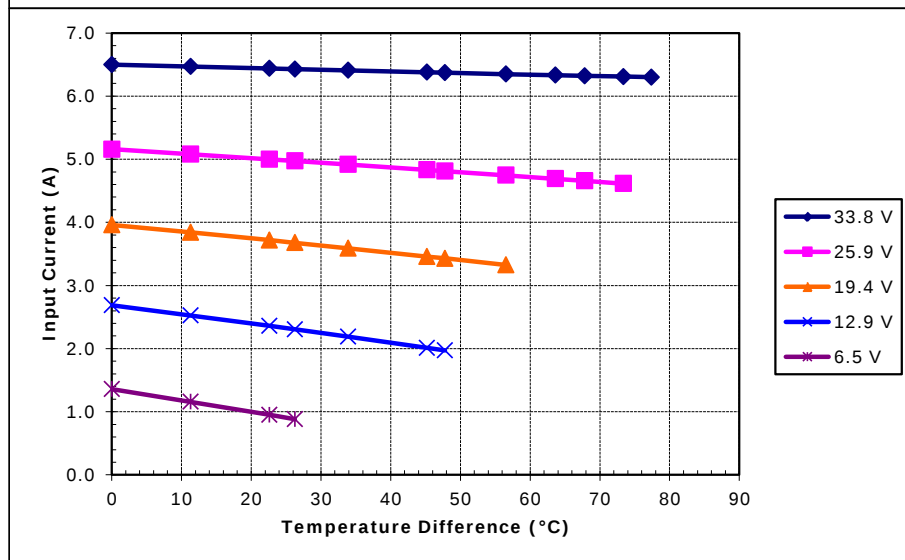
Unpotted RD-253-1.4-1.5 at a hot-side temperature of 50 °C
