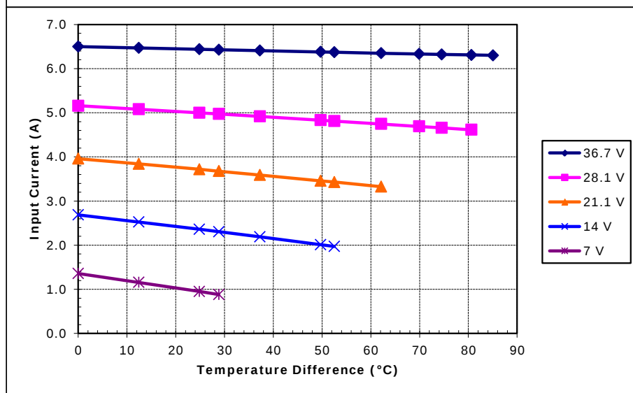
Unpotted RD-253-1.4-1.5 at a hot-side temperature of 70 °C
