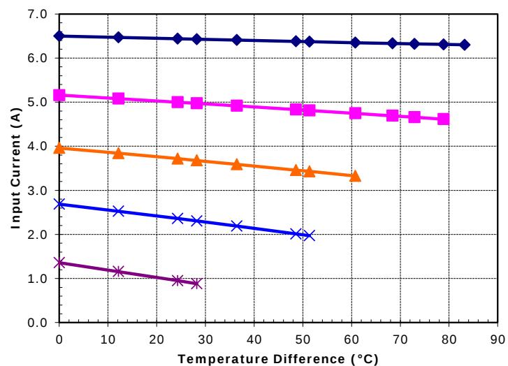
Potted RD-253-1.4-1.5 at a hot-side temperature of 70 °C
