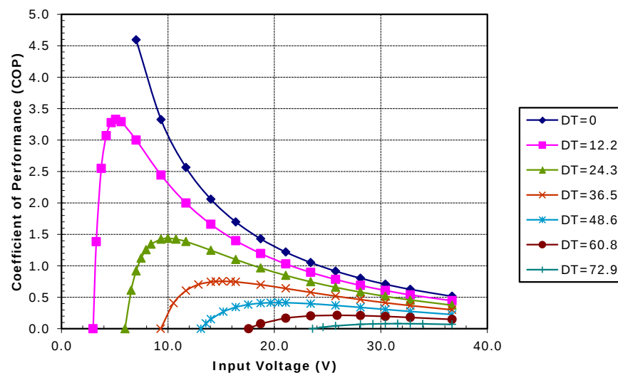
Potted RD-253-1.4-1.5 at a hot-side temperature of 70 °C
