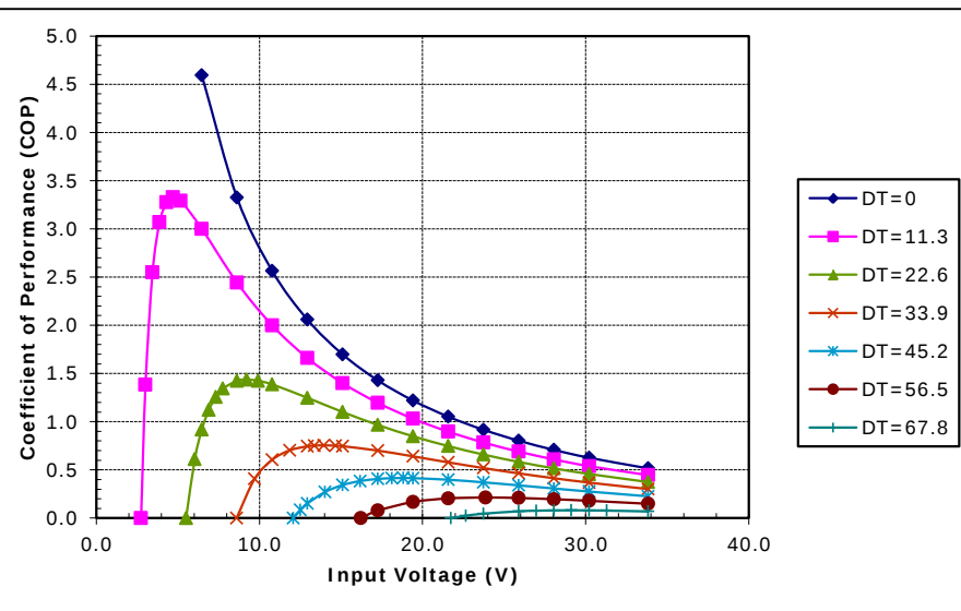
Unpotted RD-253-1.4-1.5 at a hot-side temperature of 50 °C
