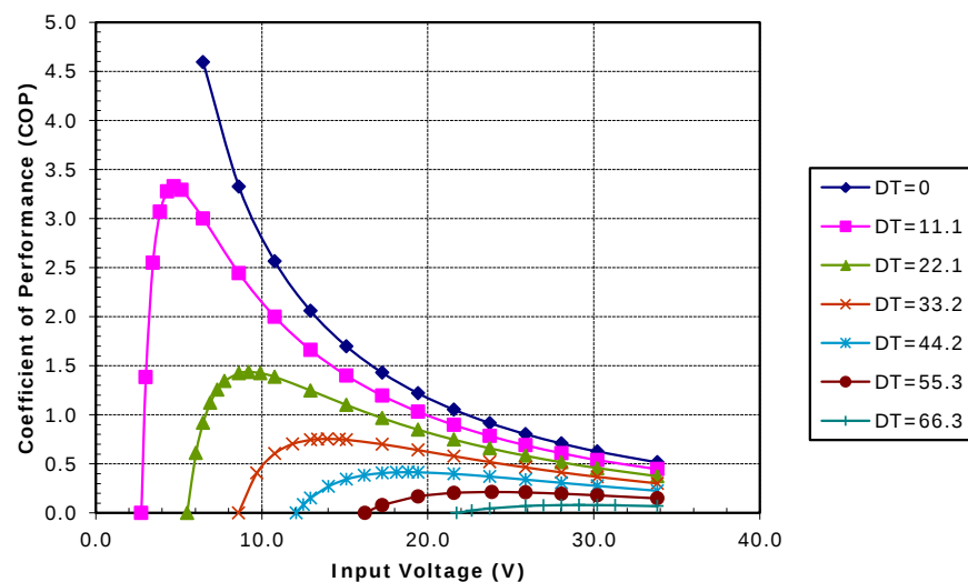
Potted RD-253-1.4-1.5 at a hot-side temperature of 50 °C
