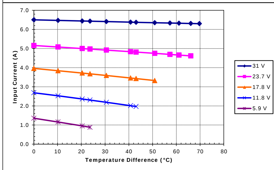
Unpotted RD-253-1.4-1.5 at a hot-side temperature of 30 °C
