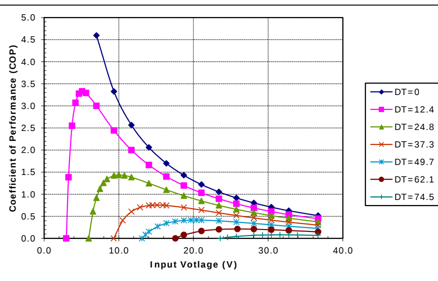
Unpotted RD-253-1.4-1.5 at a hot-side temperature of 70 °C
